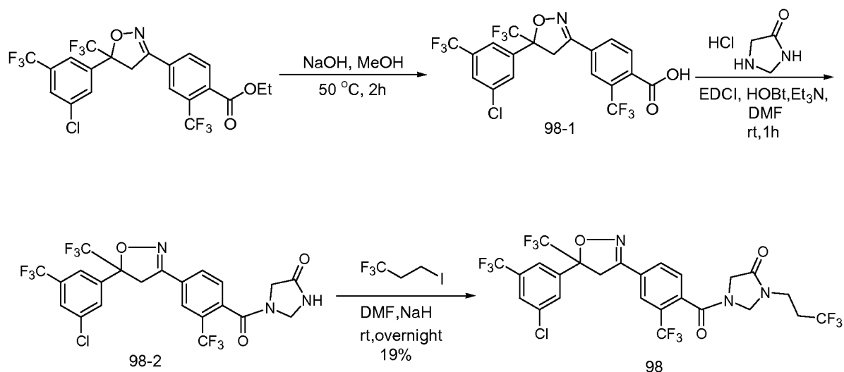
Scheme 12
