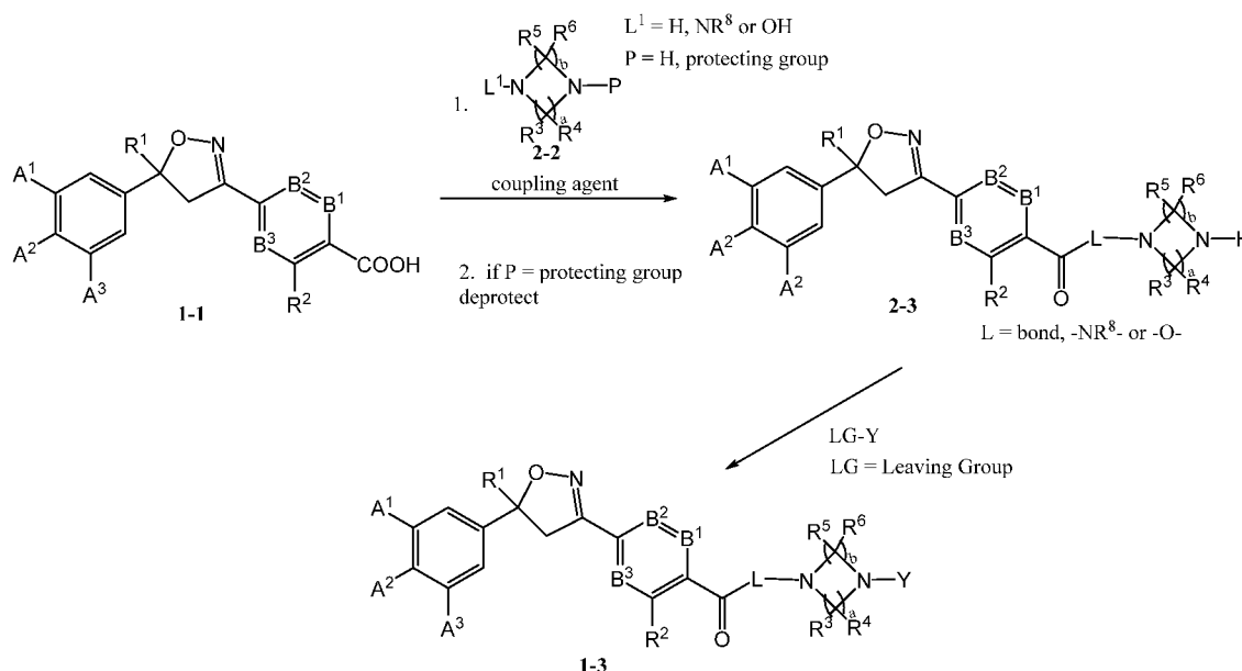
15 Scheme 2
