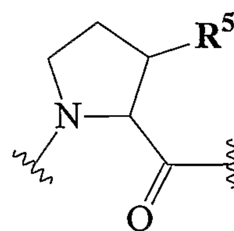
IIc
