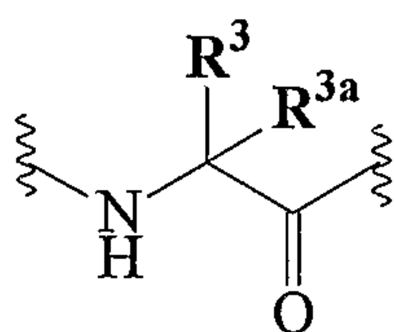
IIa
