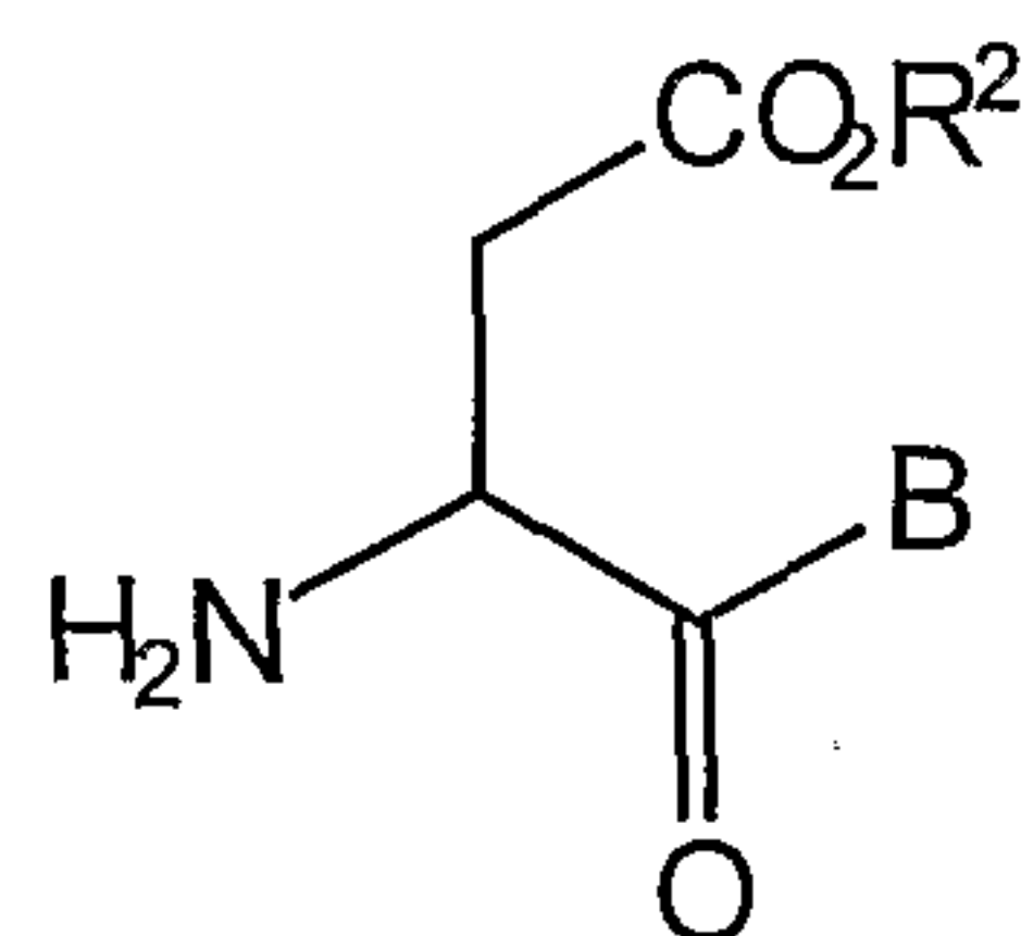
Formula Vd.
