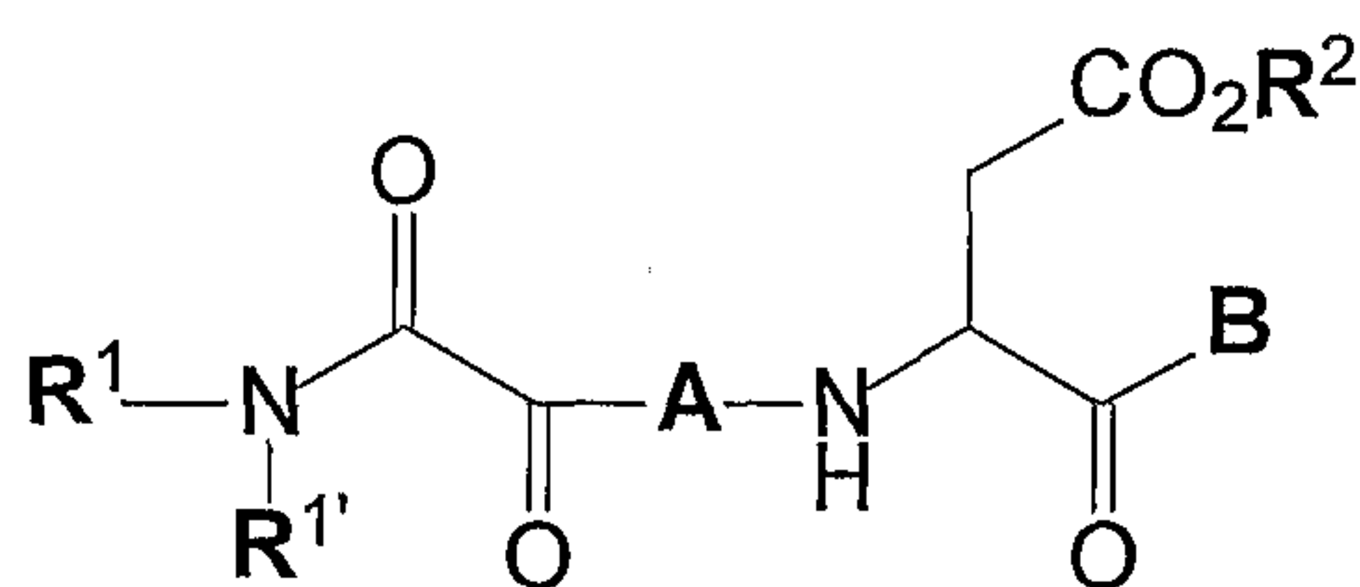
Formula I
