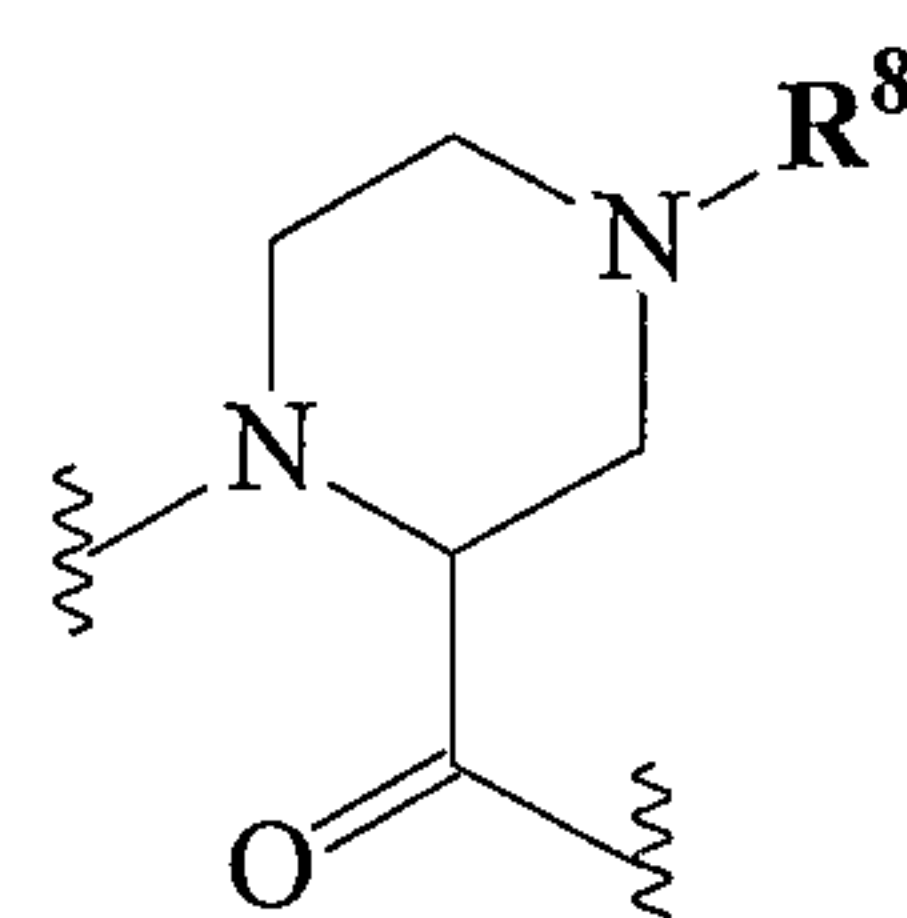
IIIf
