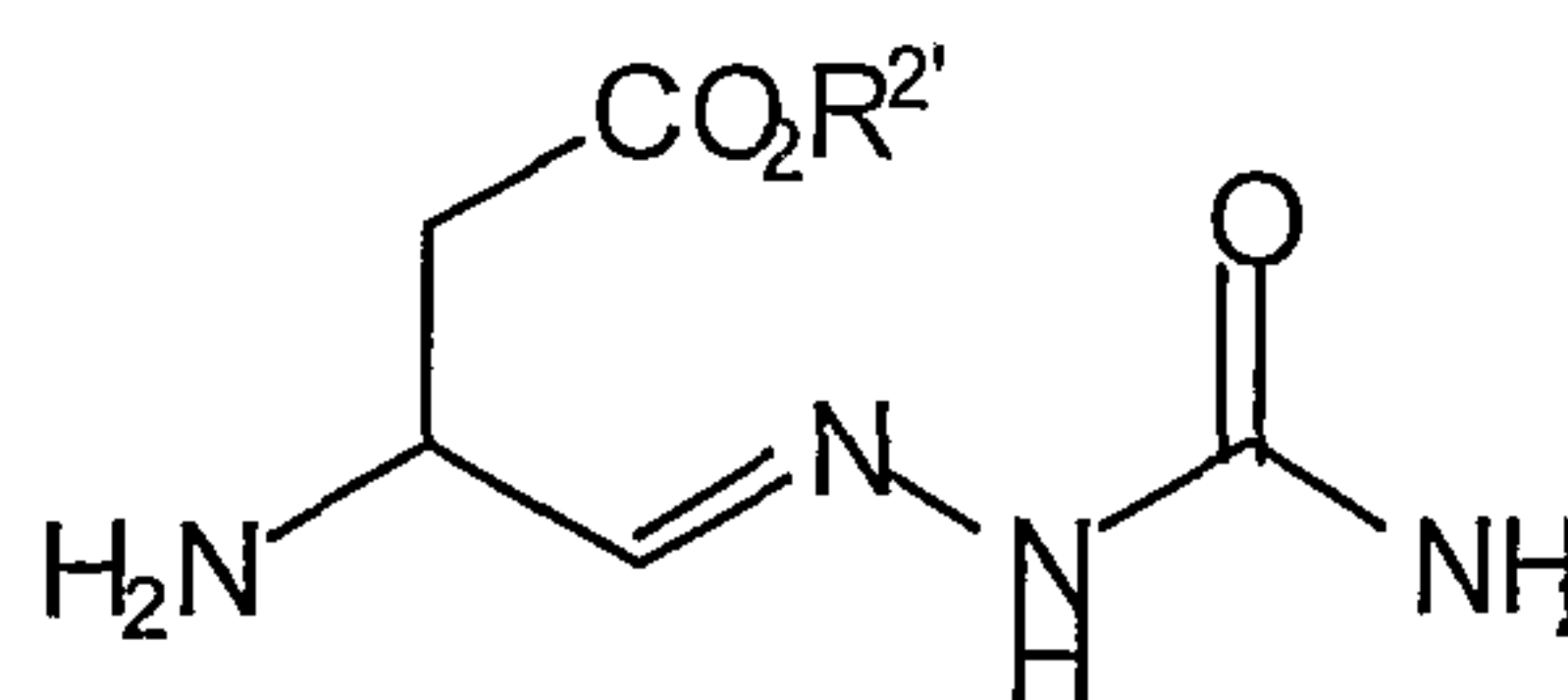
Formula Vb;
