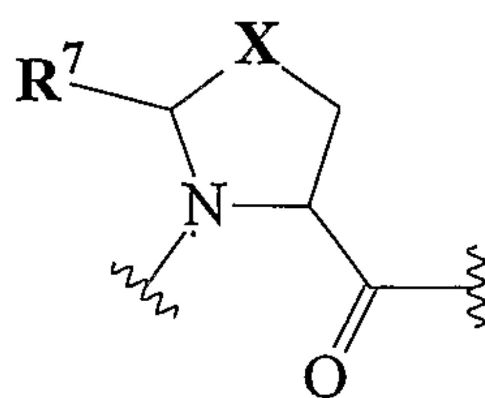
IIe
