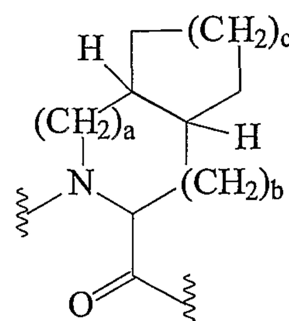
IIi
