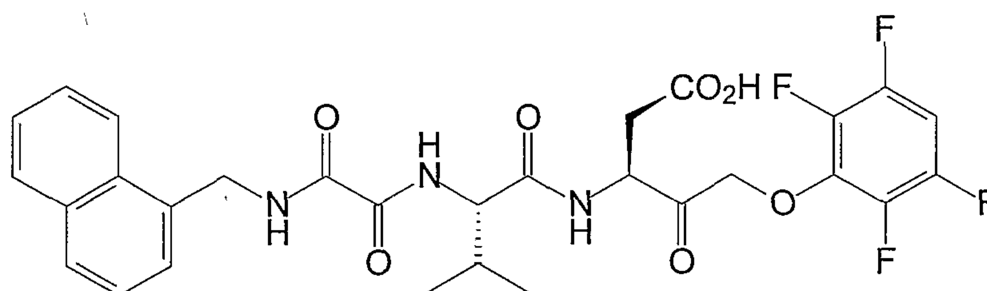
(3S)-3-[N-(N'-(1-NAPHTHYLMETHYL)OXAMYL)VALINYL]
