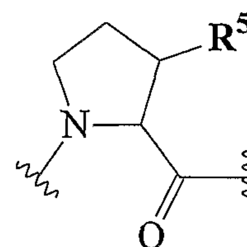
IIc
