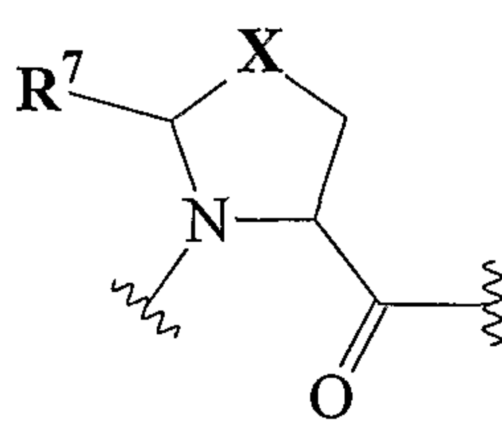
IIe
