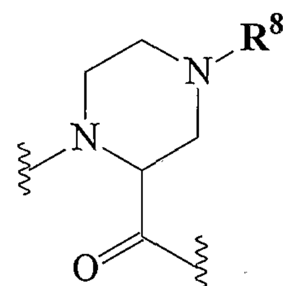
IIIf
