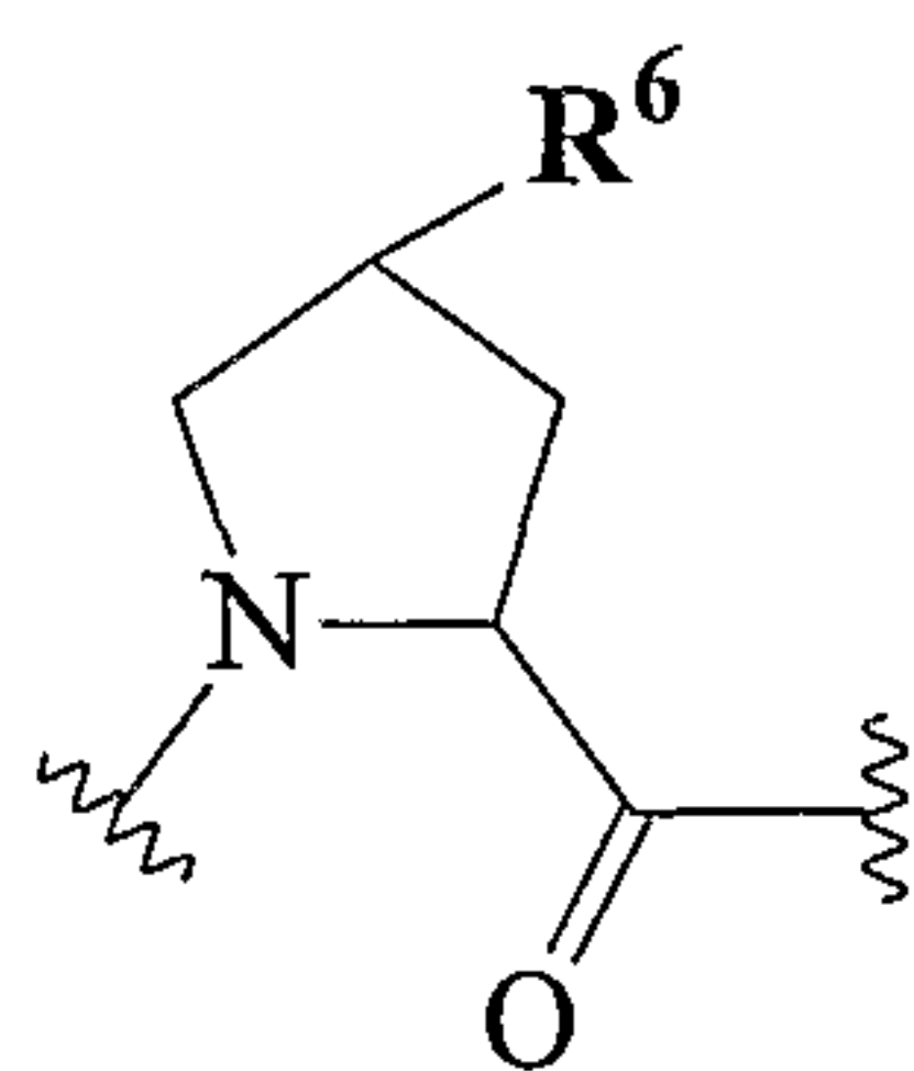
IIId
