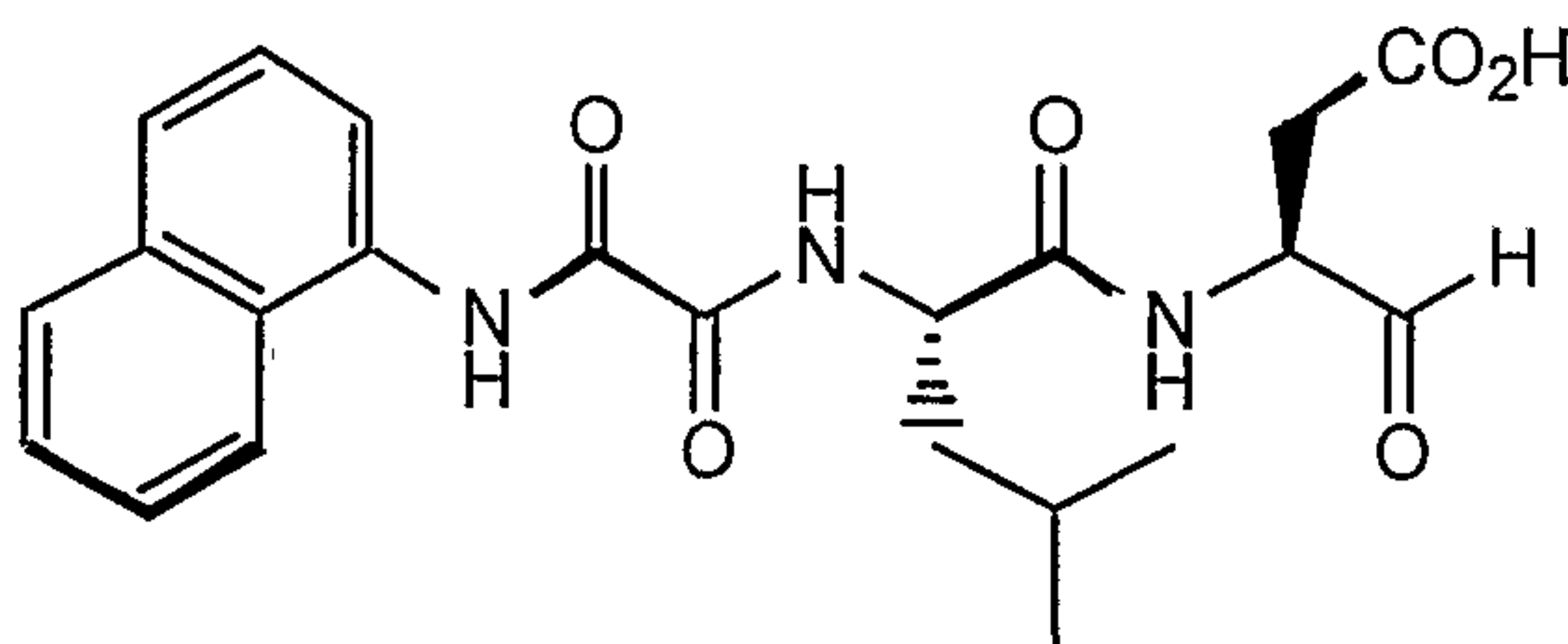
(3S)-3-[N-(N'-(1-NAPHTHYL)OXAMYL)LEUCINY]AMINO-4-OXOBUTANOIC ACID
