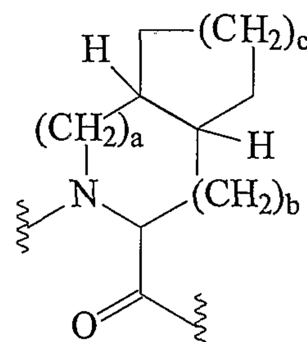
IIi
