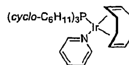
7, Crabtree's catalyst
