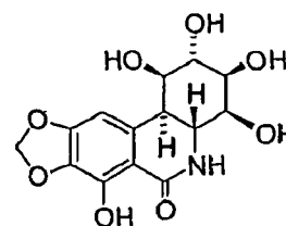
5, (+)-Pancratistatin
