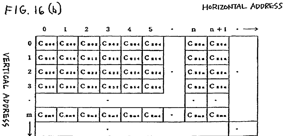
STORAGE ADDRESS OF C B AND C R SIGNAL (C MEMORY)
