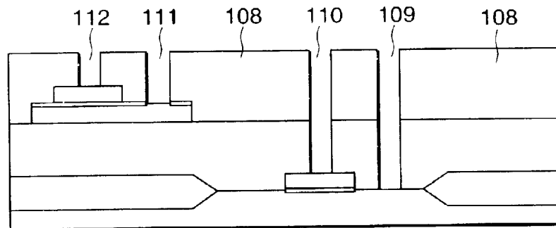
FIG. 1C (PRIOR ART)
