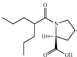
(2-propylpentanoyl)-L-proline
