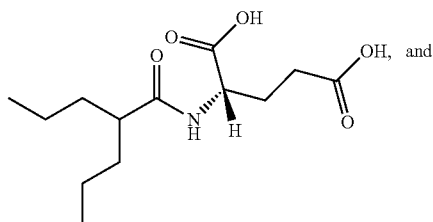
(2-propylpentanoyl)-L-glutamic acid
