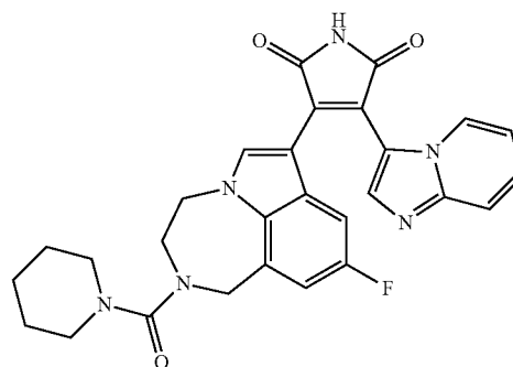
Formula III
