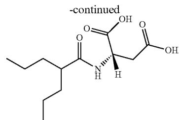
(2-propylpentanoyl)-L-aspartic acid
