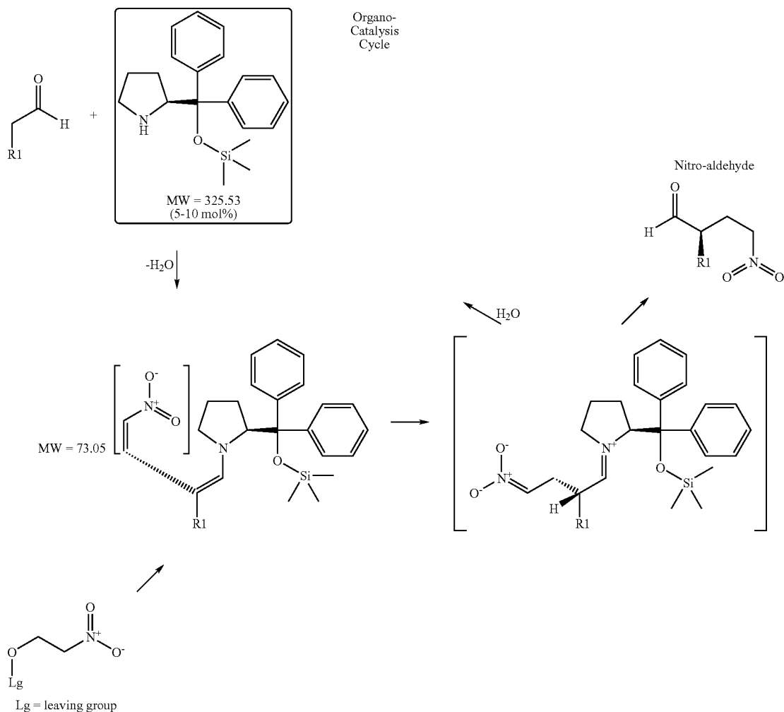
Scheme 1: Organocatalysis cycle with specific catalyst as an example
