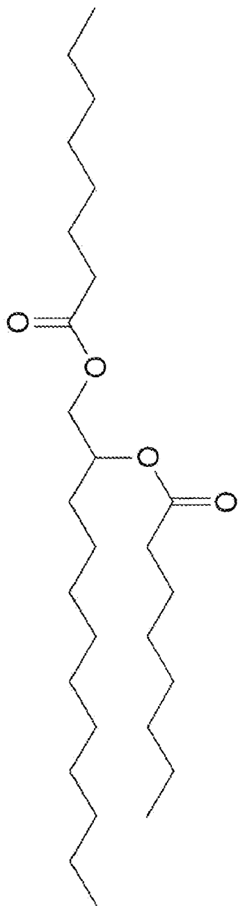
Octanoic acid 2-octanoyloxy-dodecyl ester (8)
