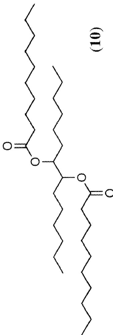
Hexanoic acid 2-hexanoyloxy-1-hexyl-octyl ester
