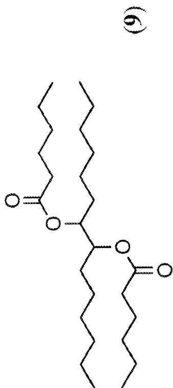
Hexanoic acid 2-hexanoyloxy-1-hexyl-octyl ester
