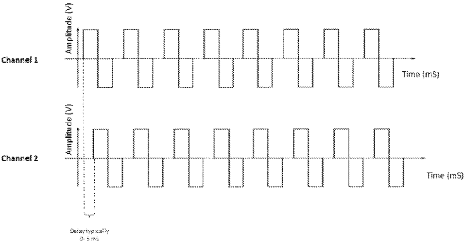
Dual channels ATP – Pacing with time delay between channels
