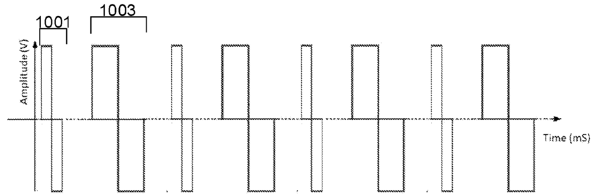
ATP with combination of regular and enhance pulses (alternating sequence)
