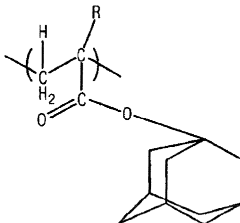
[Chemical Formula 24]
