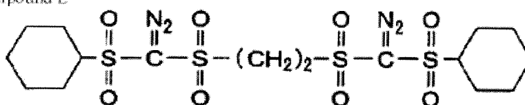
Compound F
