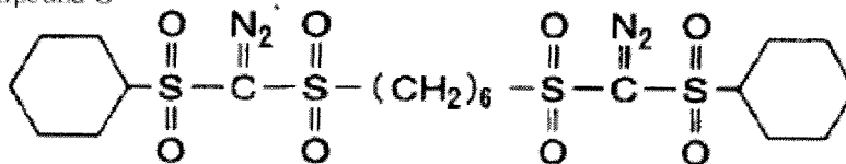
Compound H
