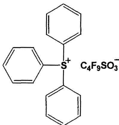
[Chemical Formula 30]
