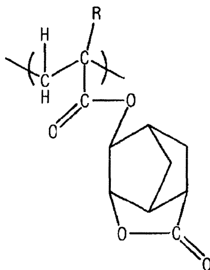
[Chemical Formula 18]
