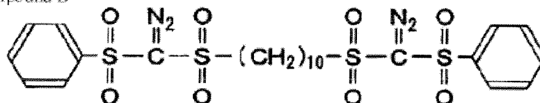
Compound E
