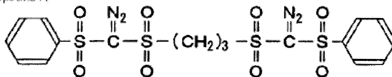
Compound B
