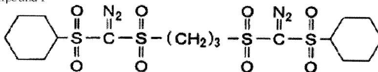
Compound G
