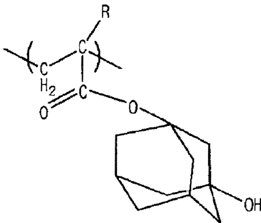
[Chemical Formula 22]
