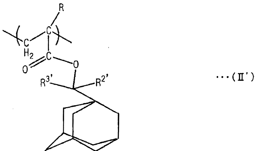
[Chemical Formula 14]
