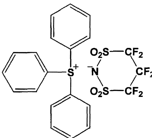
[Chemical Formula 28]
