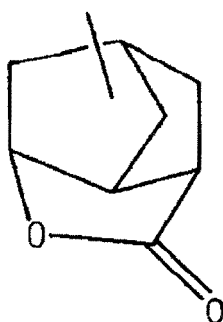
[Chemical Formula 17]
