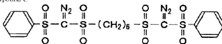
Compound D
