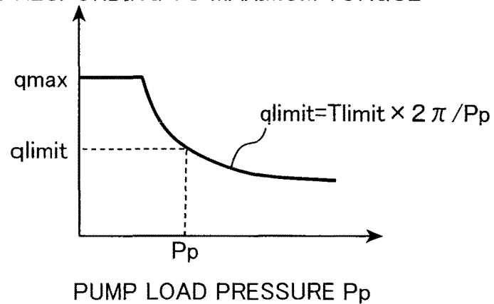
PUMP DISPLACEMENT VOLUME CORRESPONDING TO MAXIMUM TORQUE
