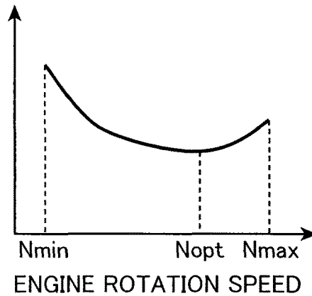
FIG. 8 ENGINE FUEL CONSUMPTION RATE
