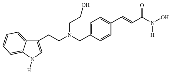
Dacinostat
