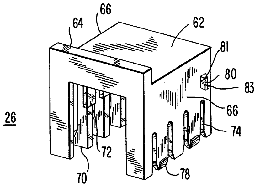
FIG. 5 PRIOR ART
