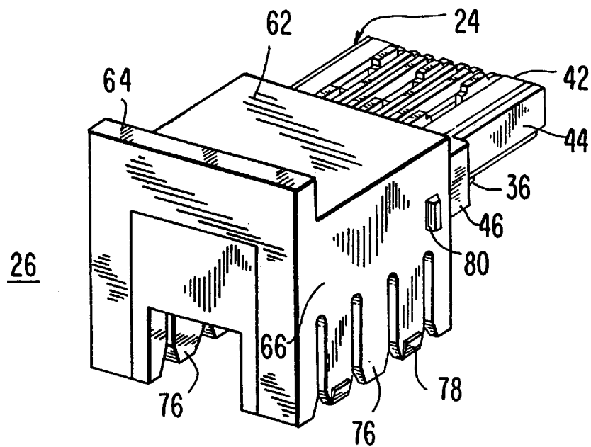
FIG. 6 PRIOR ART
