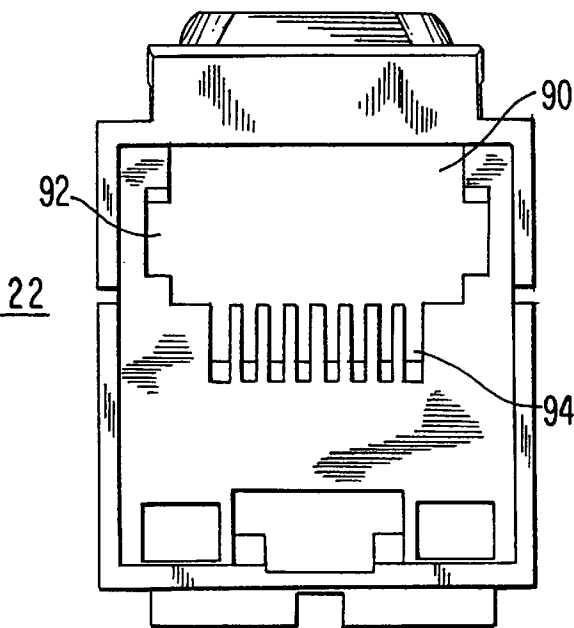
FIG. 15 PRIOR ART
