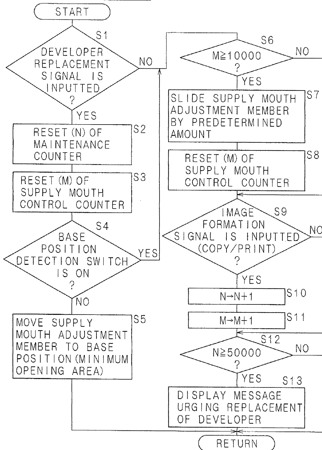
FIG. 9 CONTROL OF CONVEYANCE OF DEVELOPER
