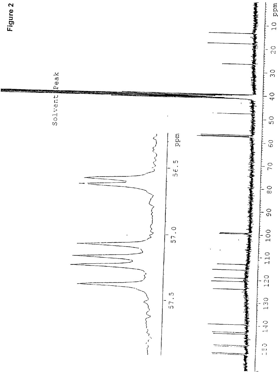
13 C NMR spectra of 3-ethyl-2-methyl-3-(2'',4'',5''-trimethoxy)phenyl-1-(2',4',5'-trimethoxy)phenyl-1-propene
