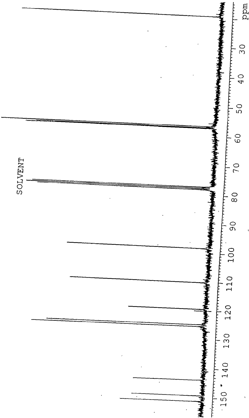
^{13}\text{C} NMR (75.4 MHz) spectra of \alpha -asarone in \text{CDCl}_3
