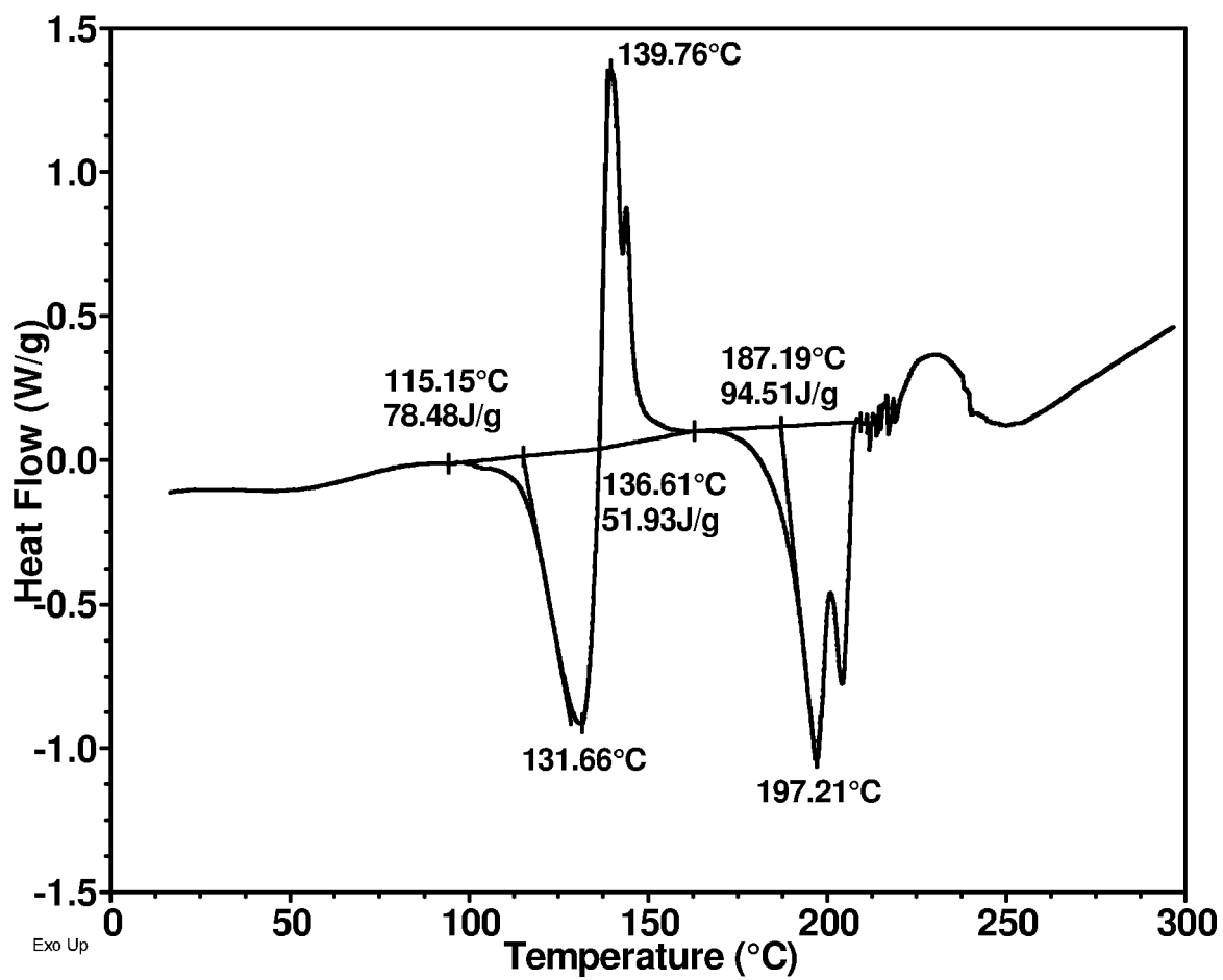
DSC thermogram of Compound 15 HCl salt Form I
