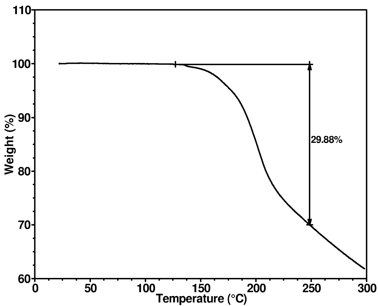
TGA thermogram of Compound 15 HCl salt Material C
