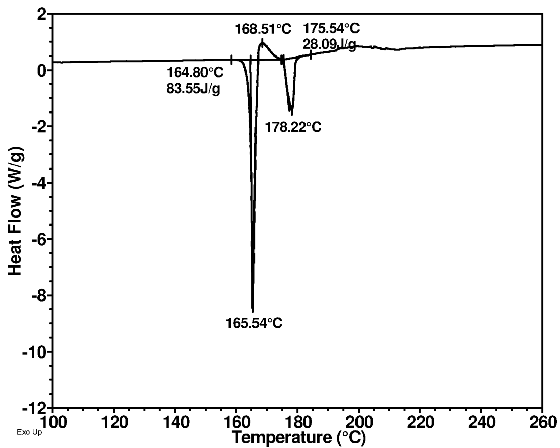
DSC thermogram of Compound 15 freebase Form II
