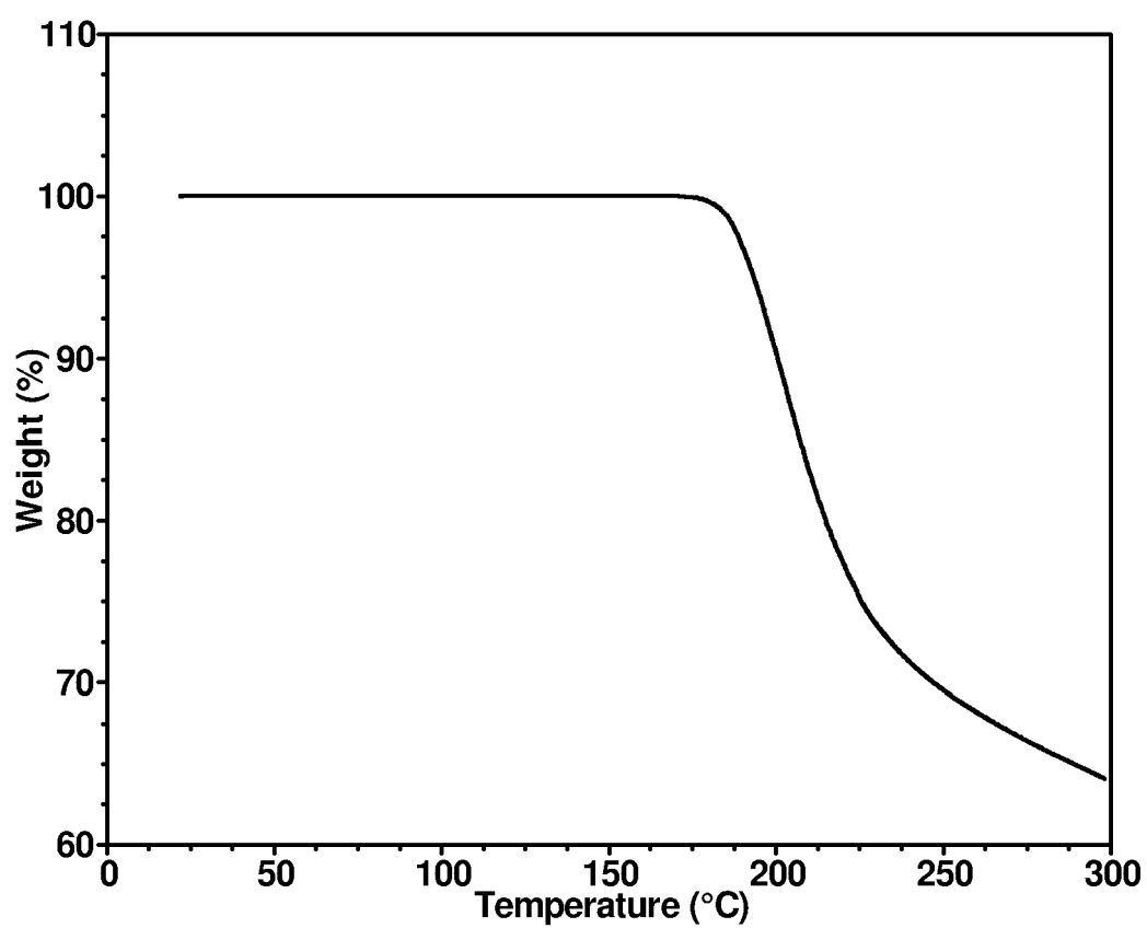
TGA thermogram of Compound 15 freebase Form I
