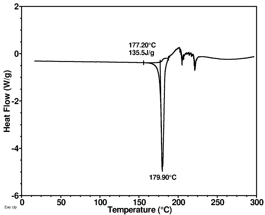
DSC thermogram of Compound 15 freebase Form III
