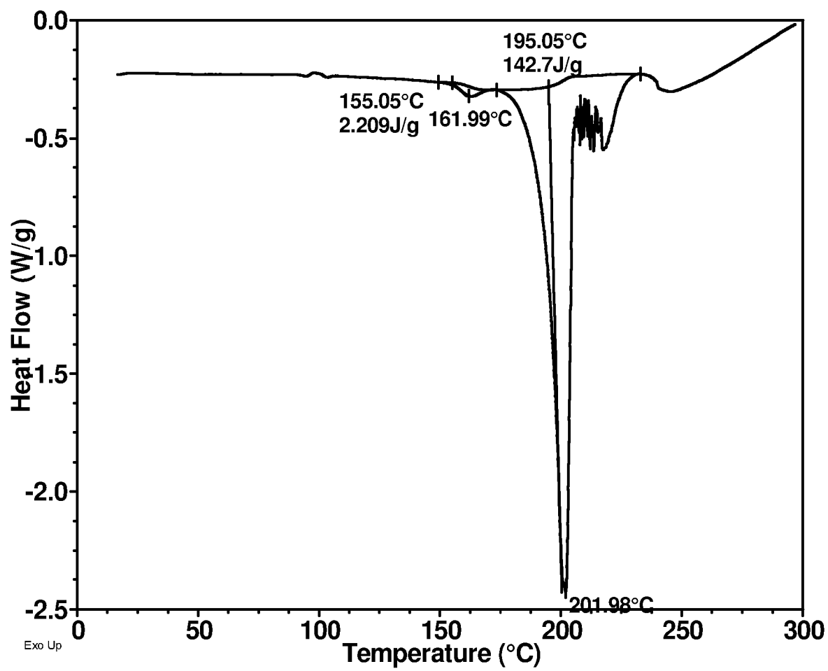
DSC thermogram of Compound 15 HCl salt Material A
