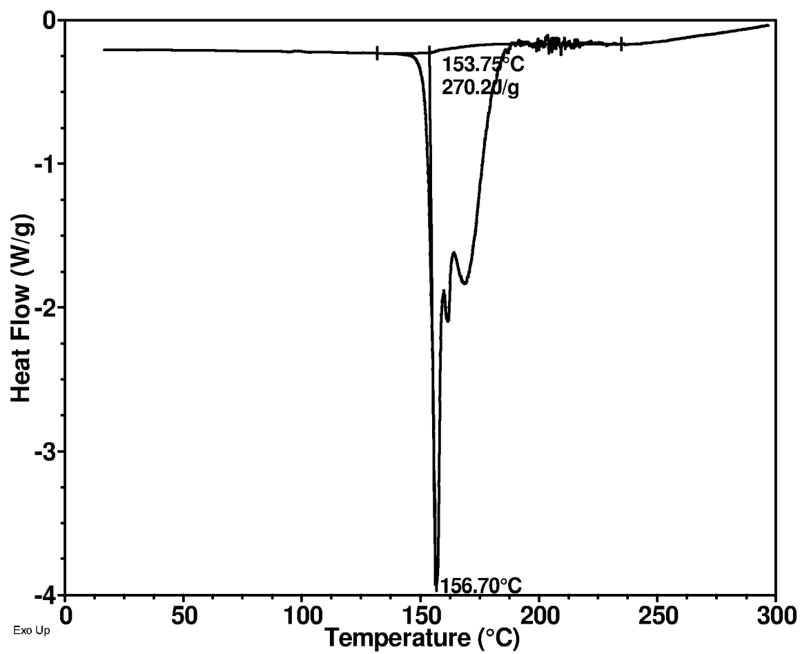
DSC thermogram of Compound 15 xinafoate Material A
