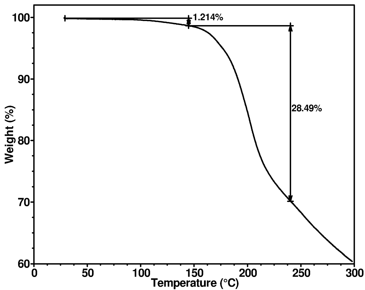
TGA thermogram of Compound 15 HCl salt Material B
