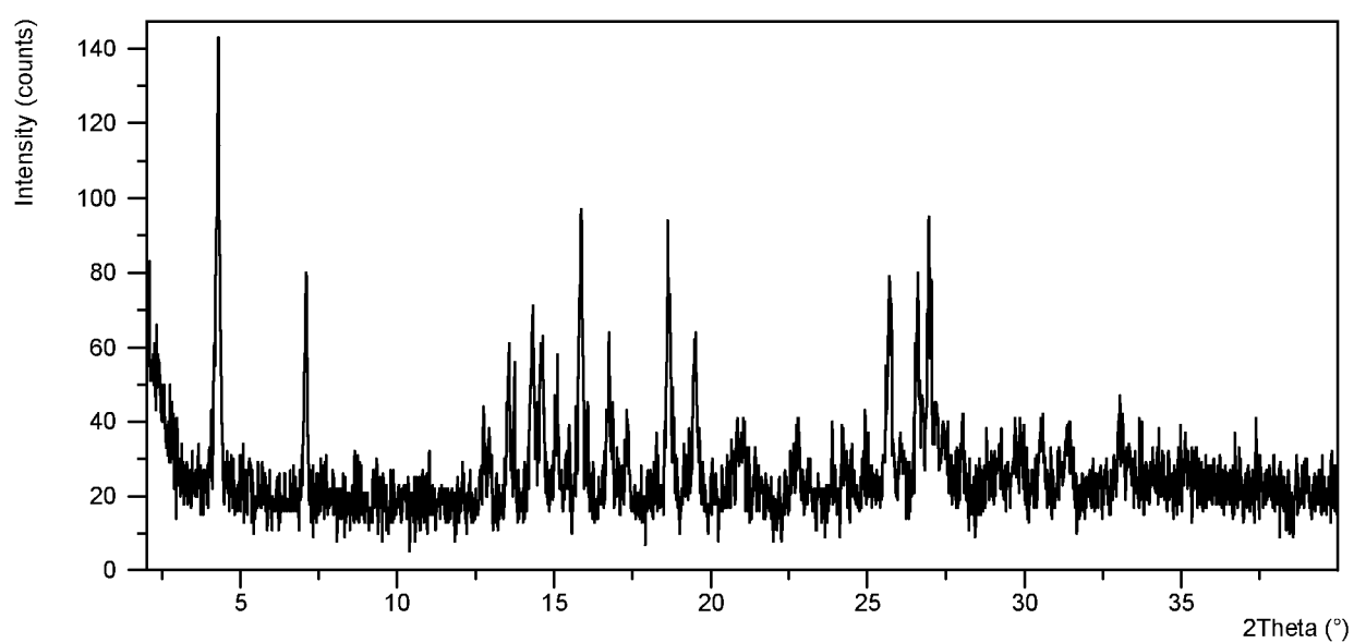
XRPD pattern of Compound 15 HCl salt Material B
