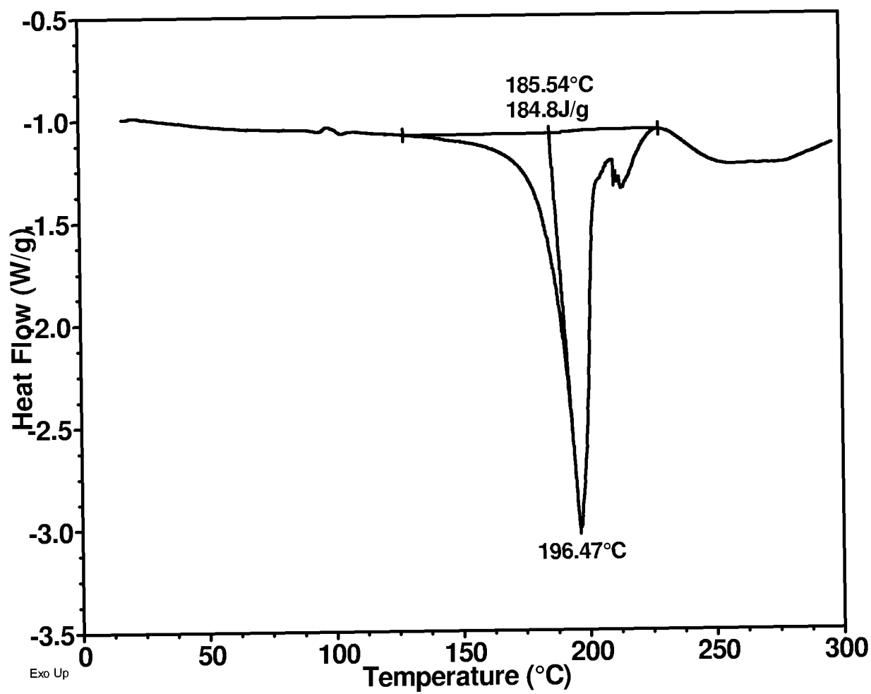
DSC thermogram of Compound 15 HCl salt Material C
