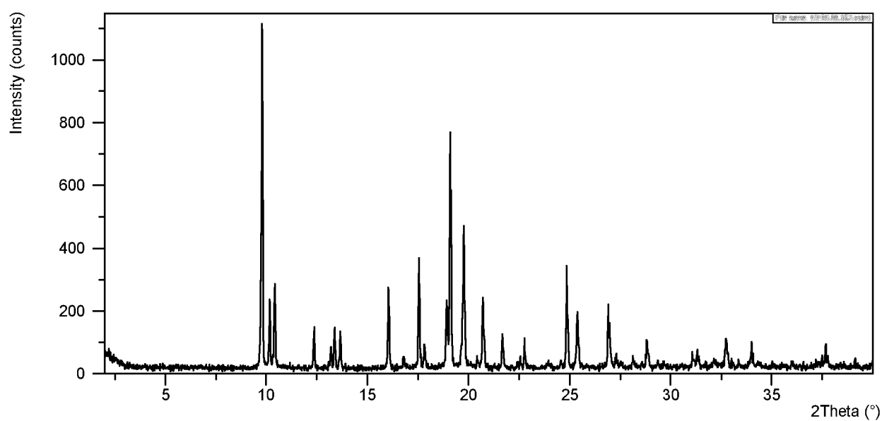
XRPD pattern of Compound 15 freebase Form III
