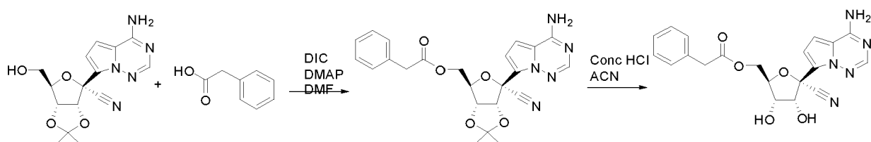
Compound 22
