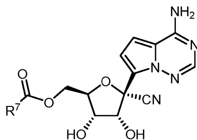
Formula Ib
