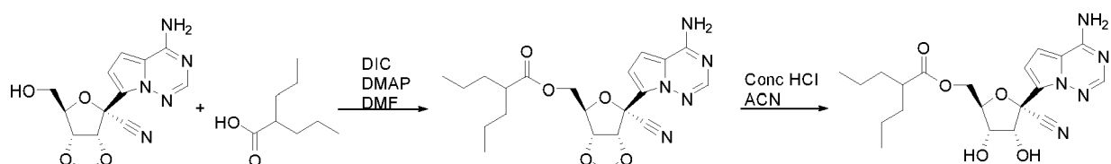
Compound 18
