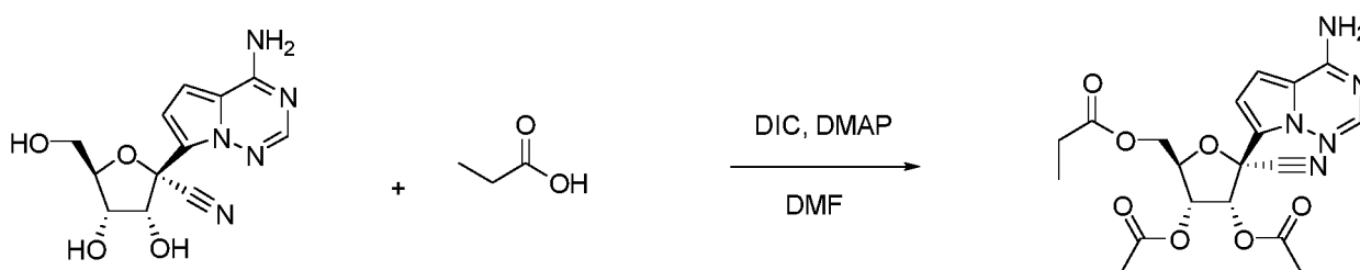
Compound 3
