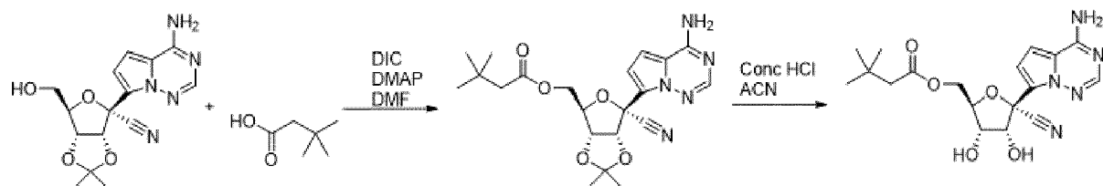
Compound 21
