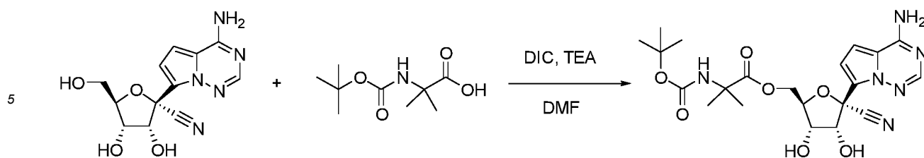
Intermediate A
