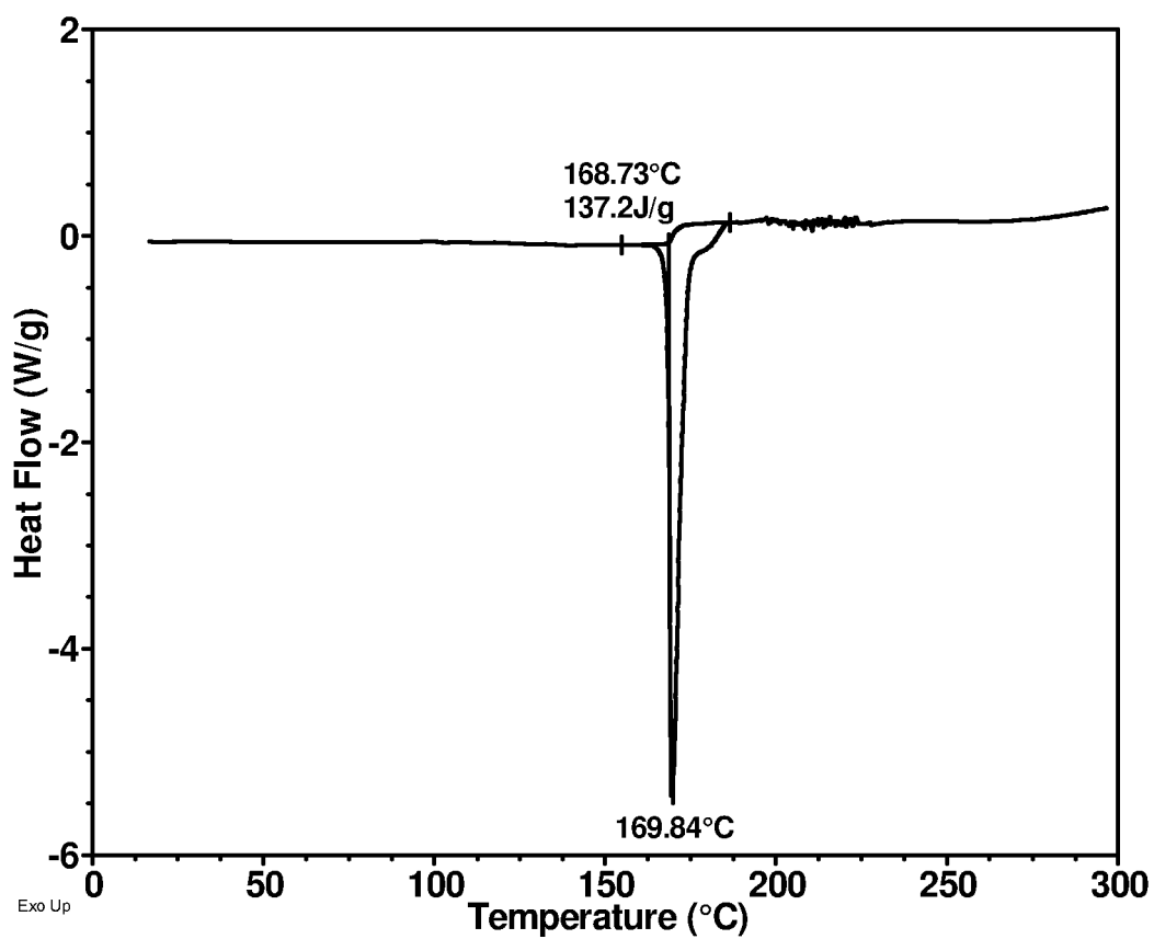
DSC thermogram of Compound 15 freebase Form I
