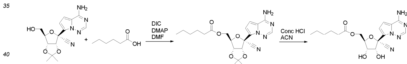
Compound 31
