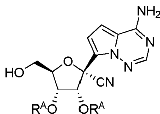
Formula A ;
