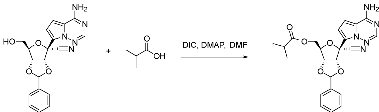
Compound 4
