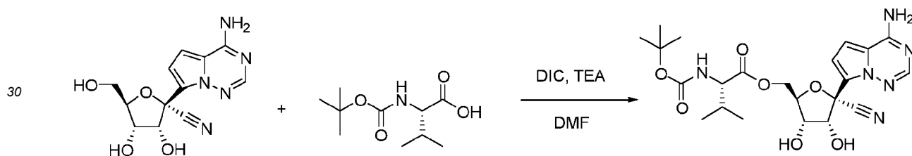
Intermediate B
