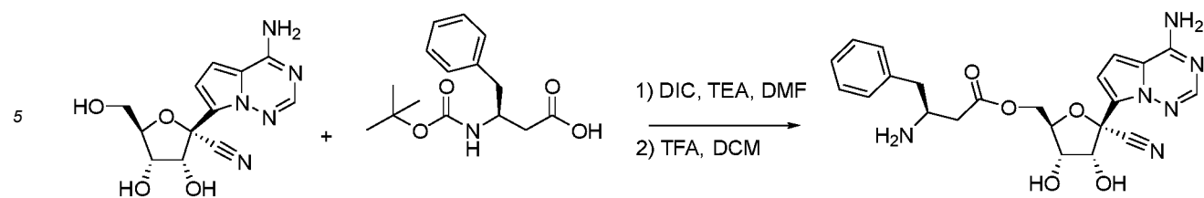
Compound 14
