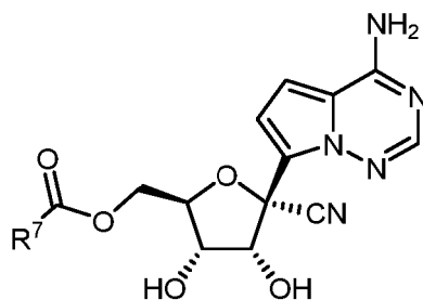
Formula Ib
