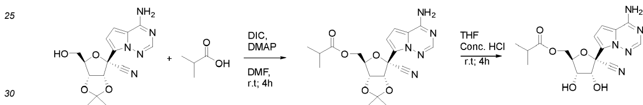
Compound 15
