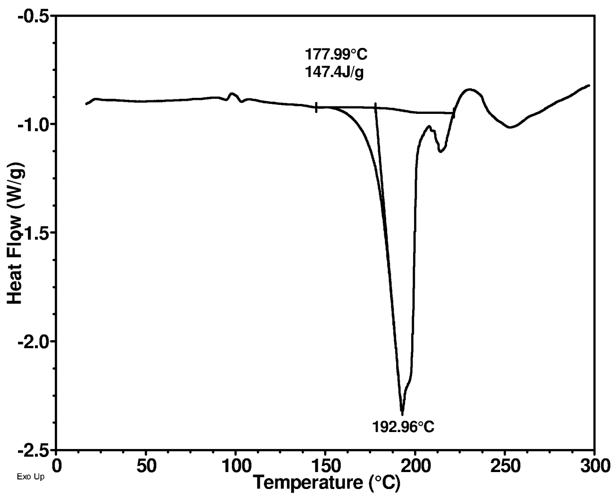
DSC thermogram of Compound 15 HCl salt Material B
