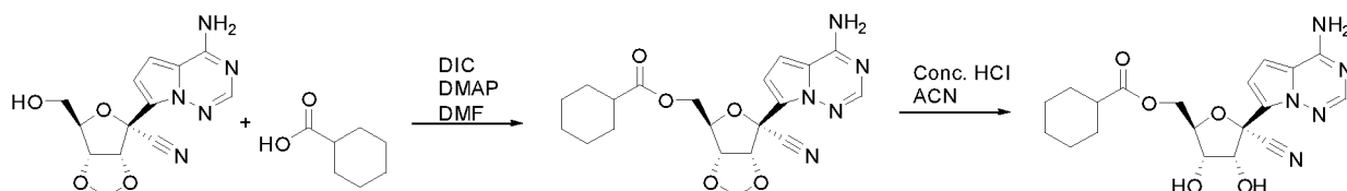
Compound 17
