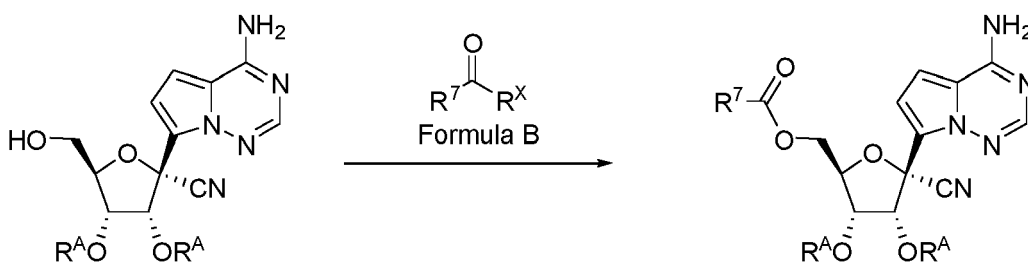
Formula A
