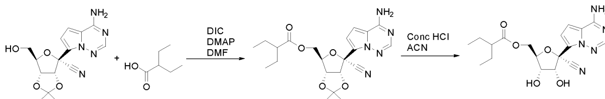
Compound 19
