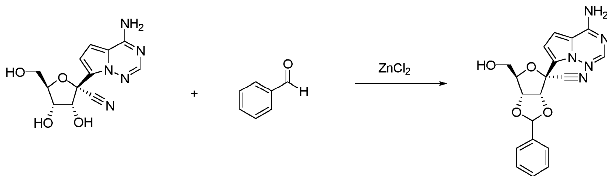
Compound 4
