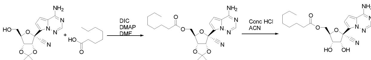
Compound 20
