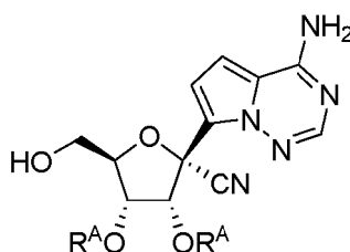
Formula A ;
