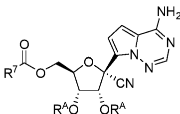
Formula C ;
