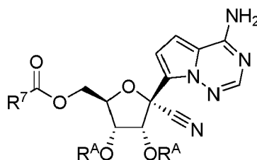
Formula C
