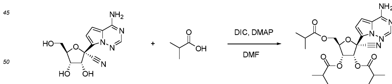
Compound 1
