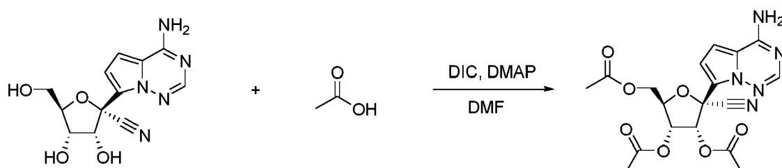
Compound 2
