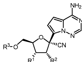
Formula Ia
