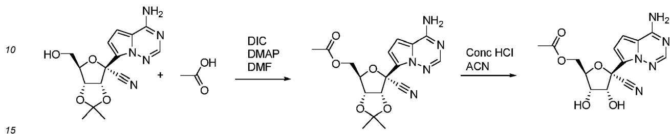
Compound 30
