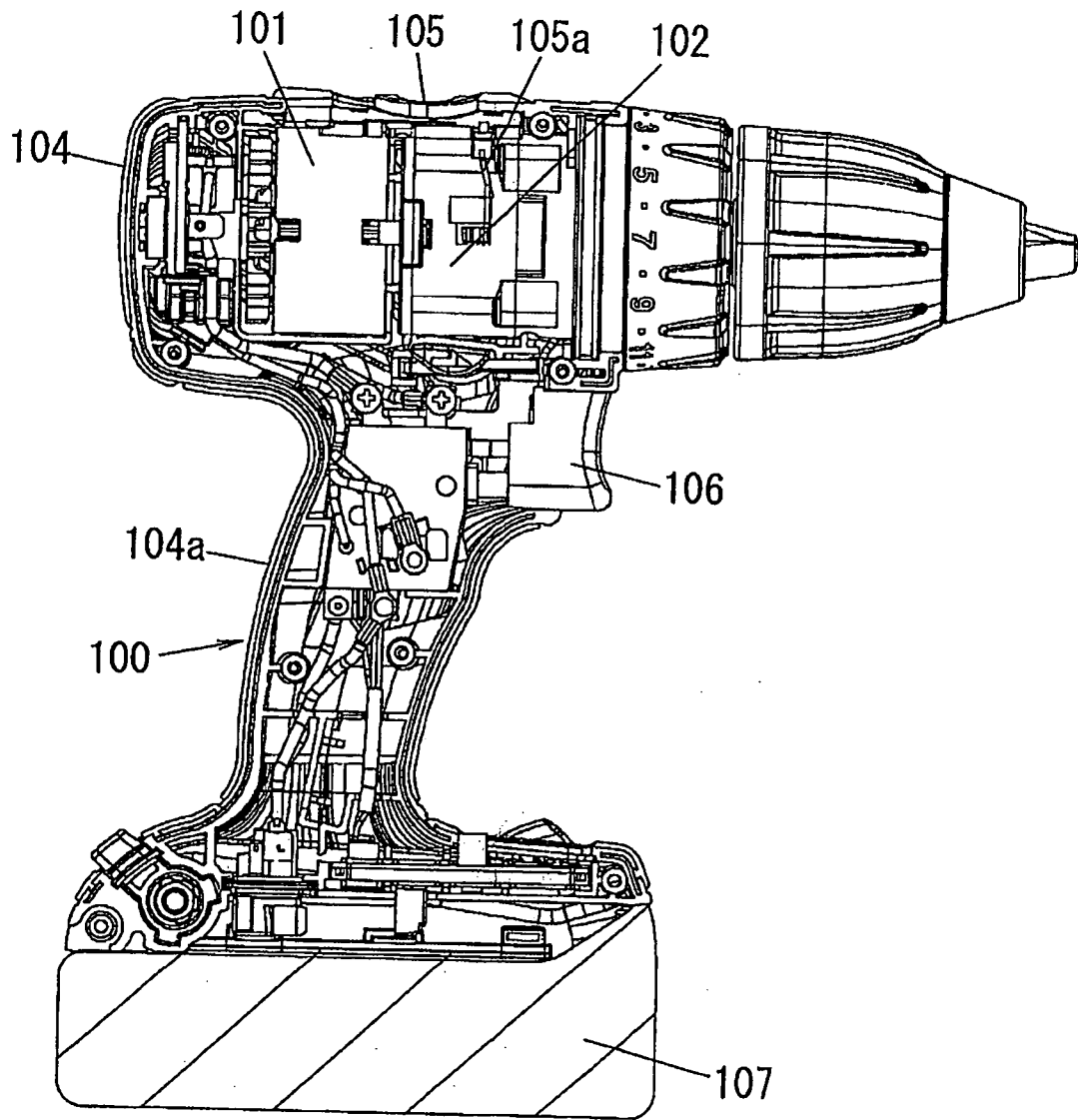
FIG. 15 (PRIOR ART)
