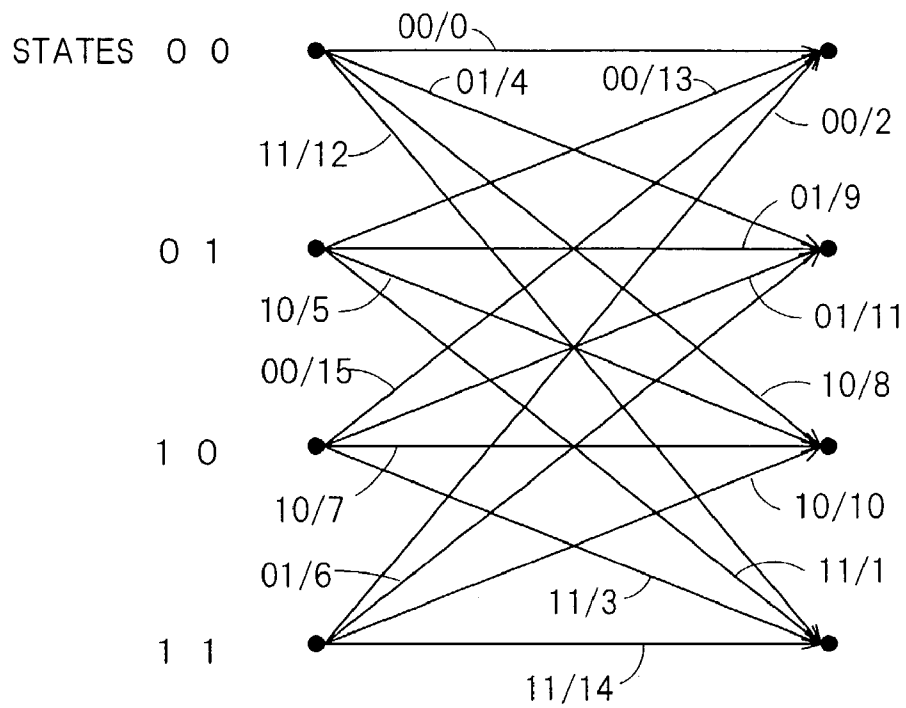
TRELLIS DIAGRAM OF TRELLIS ENCODER 701a2
