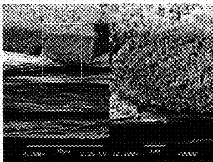
Figure 19. SEM Micrograph Additional View of Cross Section Views of Example 2 at magnification of 4,380x (left image) and 12,100x (Right image)
