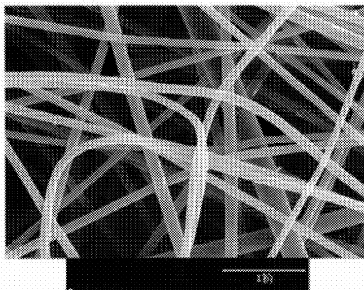
Figure 22. SEM Micrograph of PBI Electrospun Coating at 20,000x Magnification.
