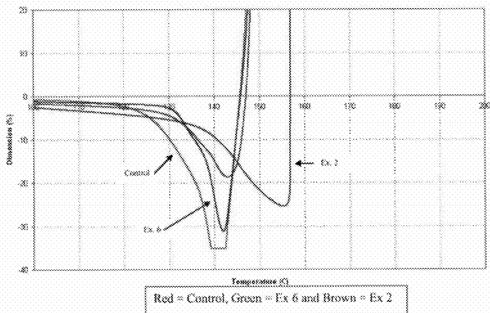
Figure 12. e-TMA of Control Sample and Examples 6 and 2.
