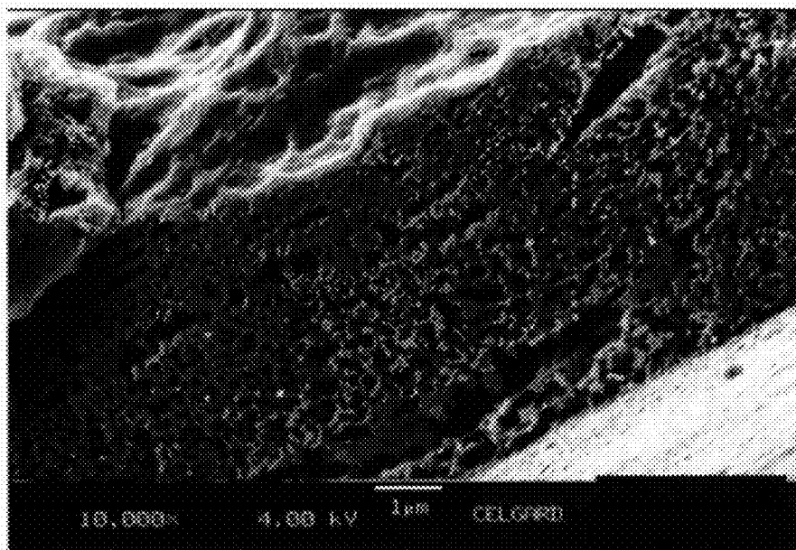
Figure 8. SEM Micrograph Showing Cross Sectional View at 10,000x magnification of Example 4.
