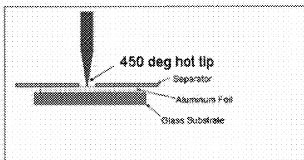
Figure 3. Diagram of Hot Tip Hole Propagation Test.
