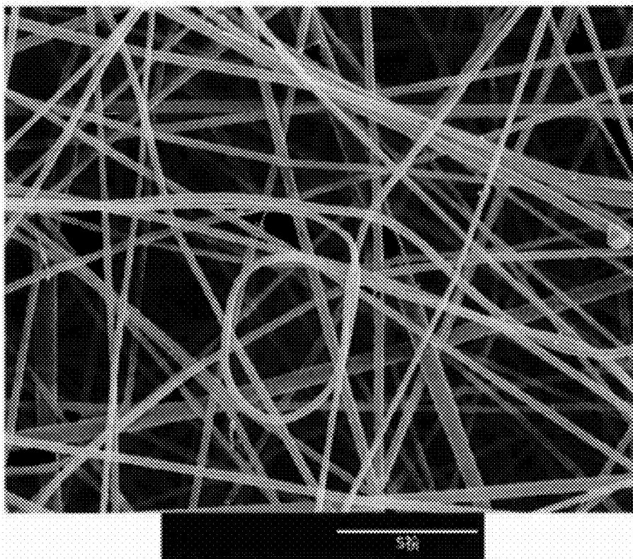
Figure 21. SEM Micrograph of PBI Electrospun Coating at 5,000x Magnification.
