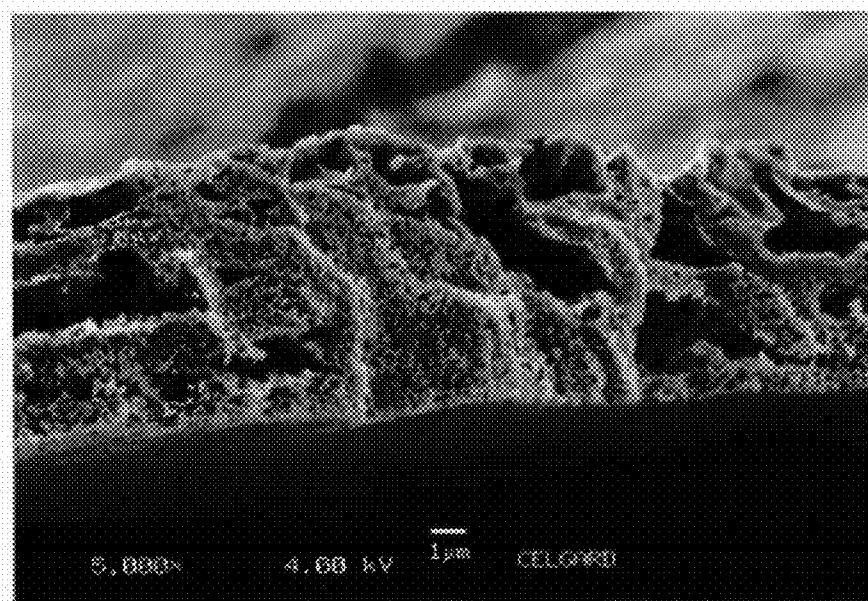
Figure 10. SEM Micrograph Showing Cross Sectional View at 5,000x Magnification of Example 3.
