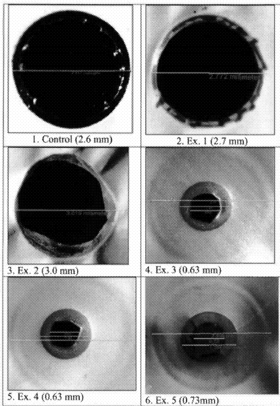
Figure 6. Hot Tip Hole Propagation Test Digital Images for Control Sample and Examples 1-5.
