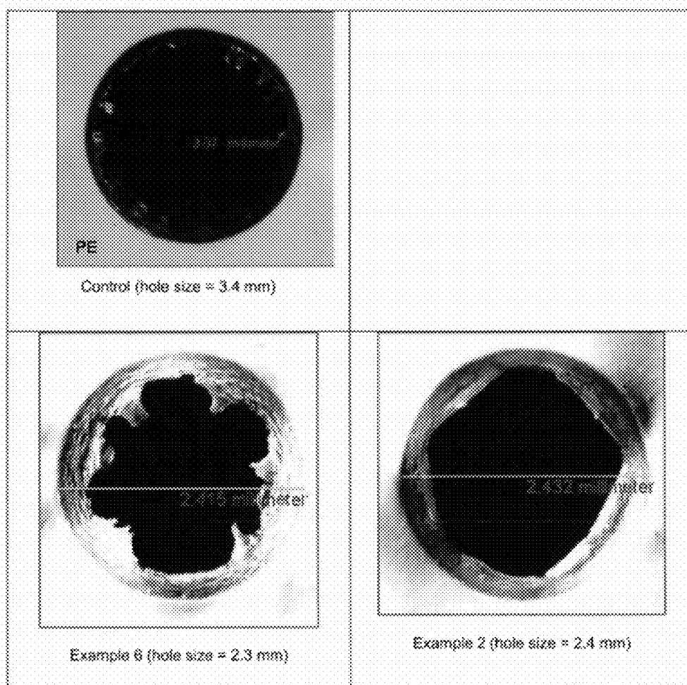
Figure 14. Hot Tip Digital Images of 16 \mu m Control Sample and Examples 6 and 2
