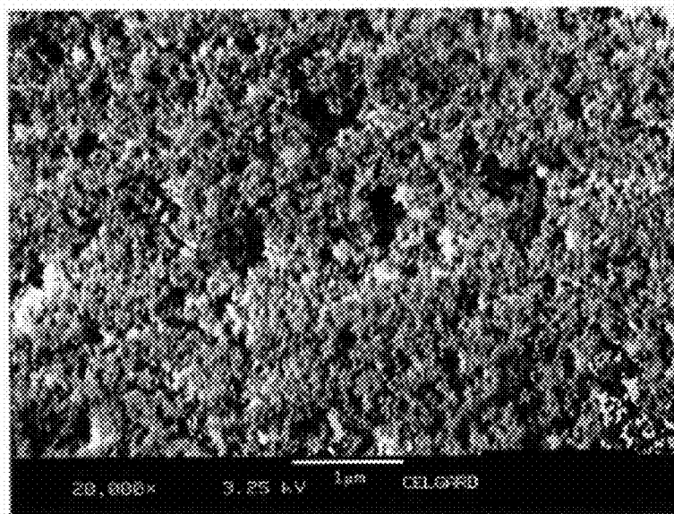
Figure 17. SEM Micrograph of Surface View at 20,000x magnification of Example 2.
