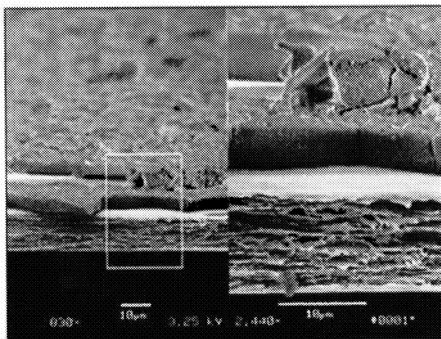
Figure 16. SEM micrograph of Cross Section Views of Example 6. at Magnification of 830x (left image) and 2,440x (right image)
