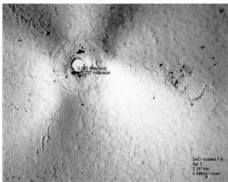
Figure 31. Hot Tip Hole Propagation 2-side PBI Coated Celgard® 3401. Hole Diameter = 0.596 mm.
