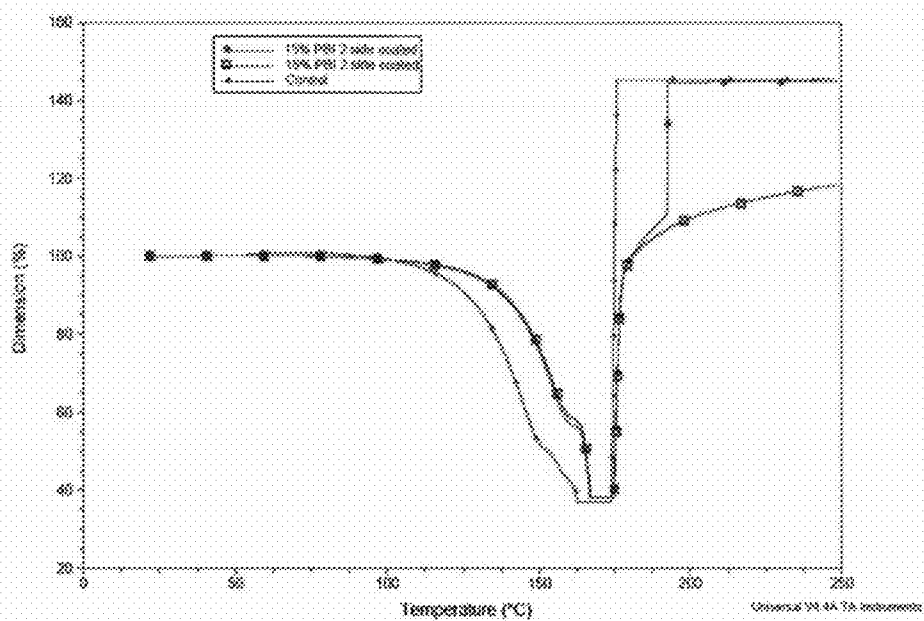
Figure 29. e-TMA of 1-sided and 2-sided Electrospun PBI Coated Celgard® 3401.
