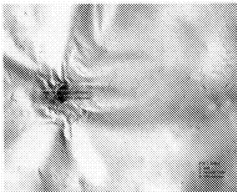
Figure 25. Hot Tip Hole Propagation 2-side PBI Coated. Hole Diameter = 0.595 mm.
