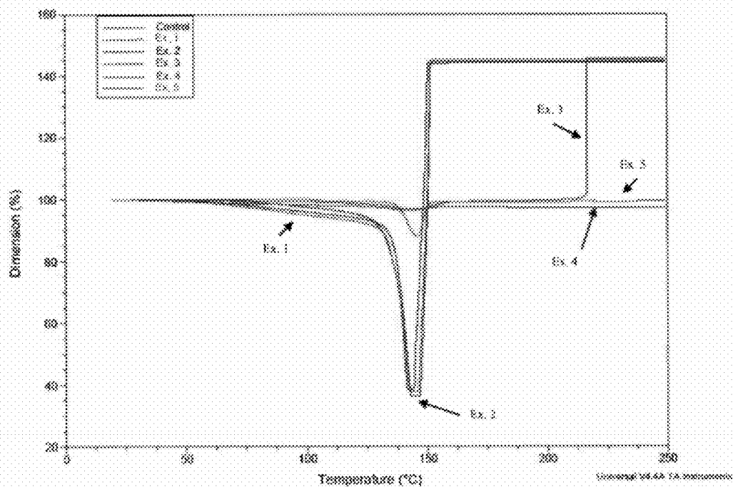
Figure 4. e-TMA Thermogram of Control Sample and Examples 1-5
