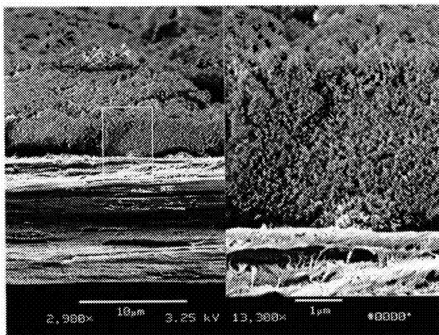
Figure 18. SEM Micrograph of Cross Section Views of Example 2 at magnification of 2,980x (left image) and 13,300x (right image)
