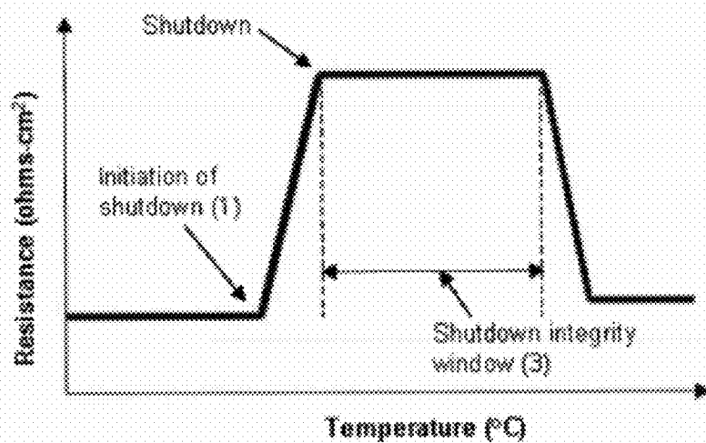
Figure 2. Hot ER Thermogram Schematic
