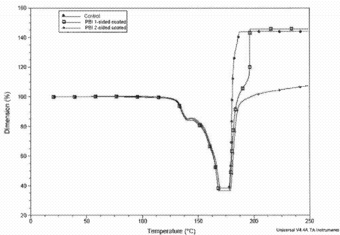
Figure 27. e-TMA of 1-sided and 2-sided Electrospun PBI Coated Celgard® M824.
