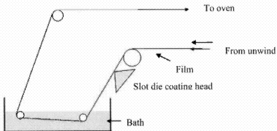
Figure 1. Schematic of Coating Process and Film Path.
