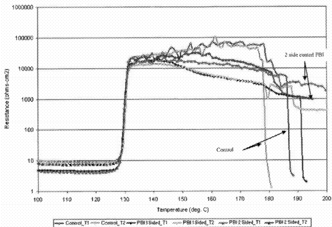
Figure 26. Hot ER Thermogram of 1-sided and 2-sided Electrospun Coated Celgard® M824.
