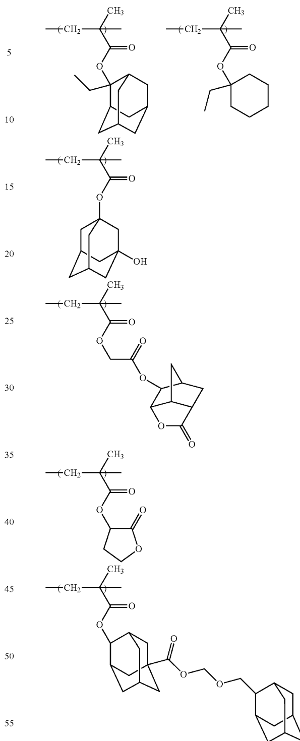
Example 8
