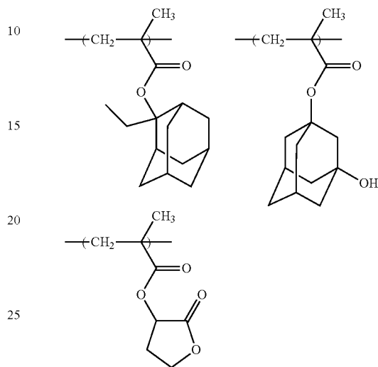
Example 9
