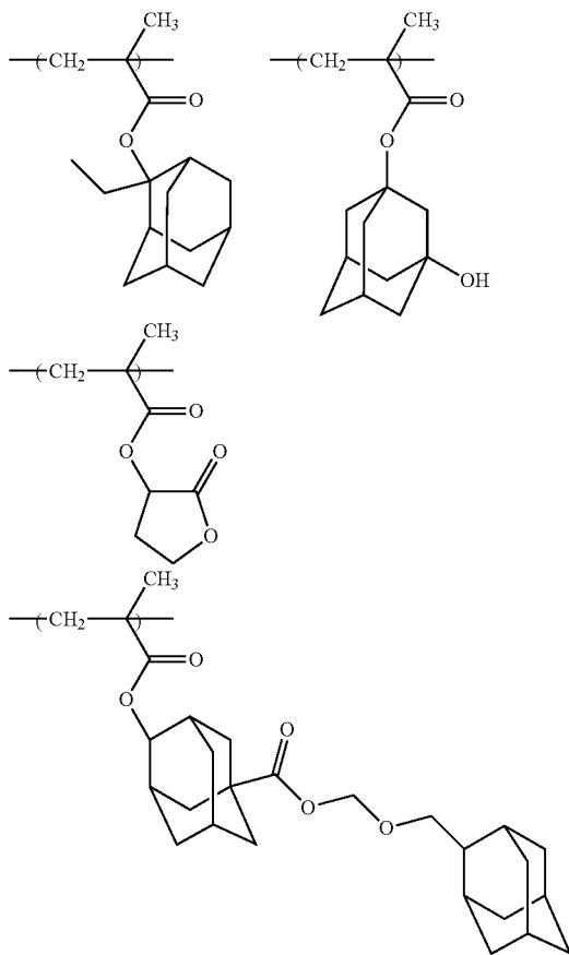
Synthesis Example 1
