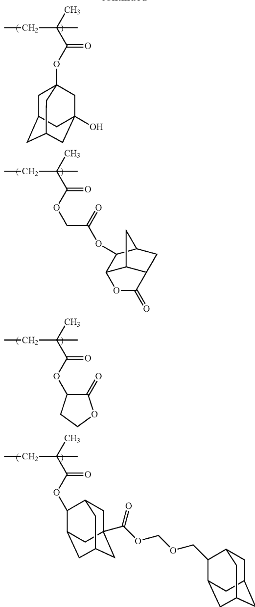
Example 10
