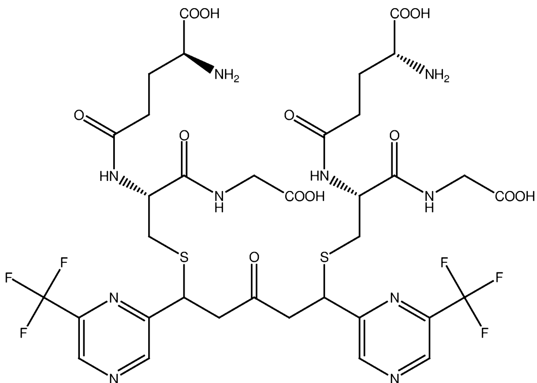
PB243 (glutathione adduct of PB240)
