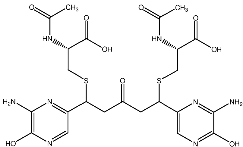
PB205 (NAC adduct of PB204)
