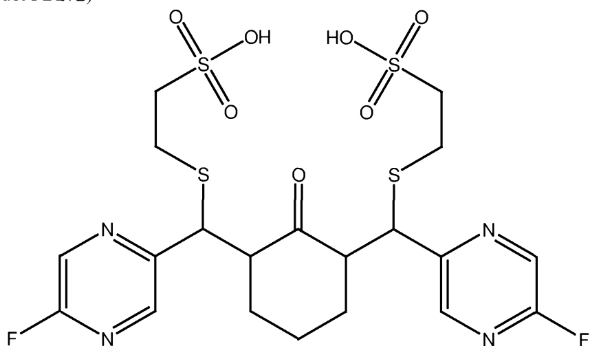
PB273 (NAC adduct PB272)
