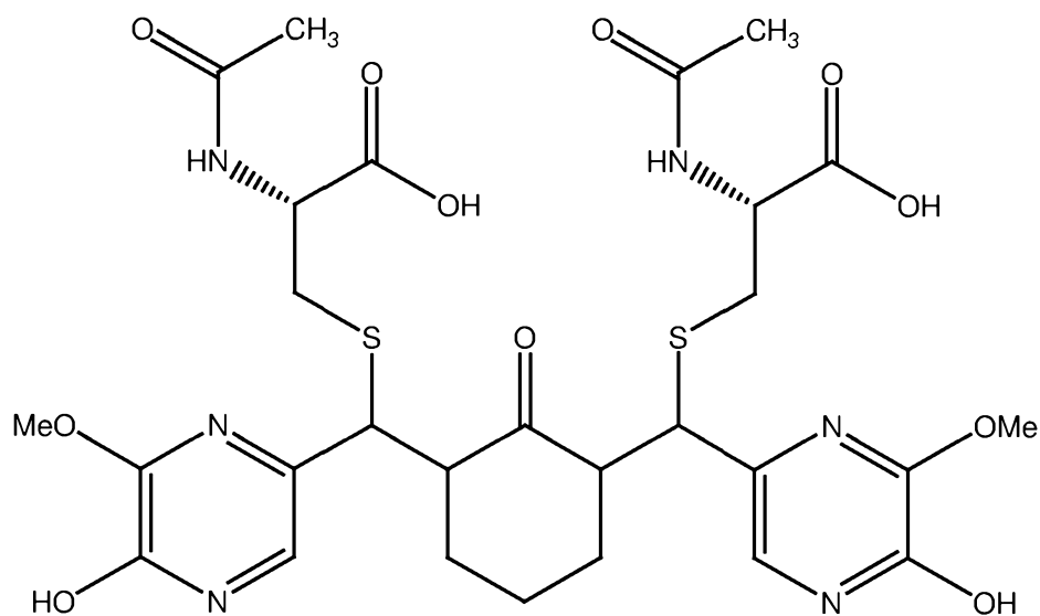
PB253 (NAC adduct of PB252)
