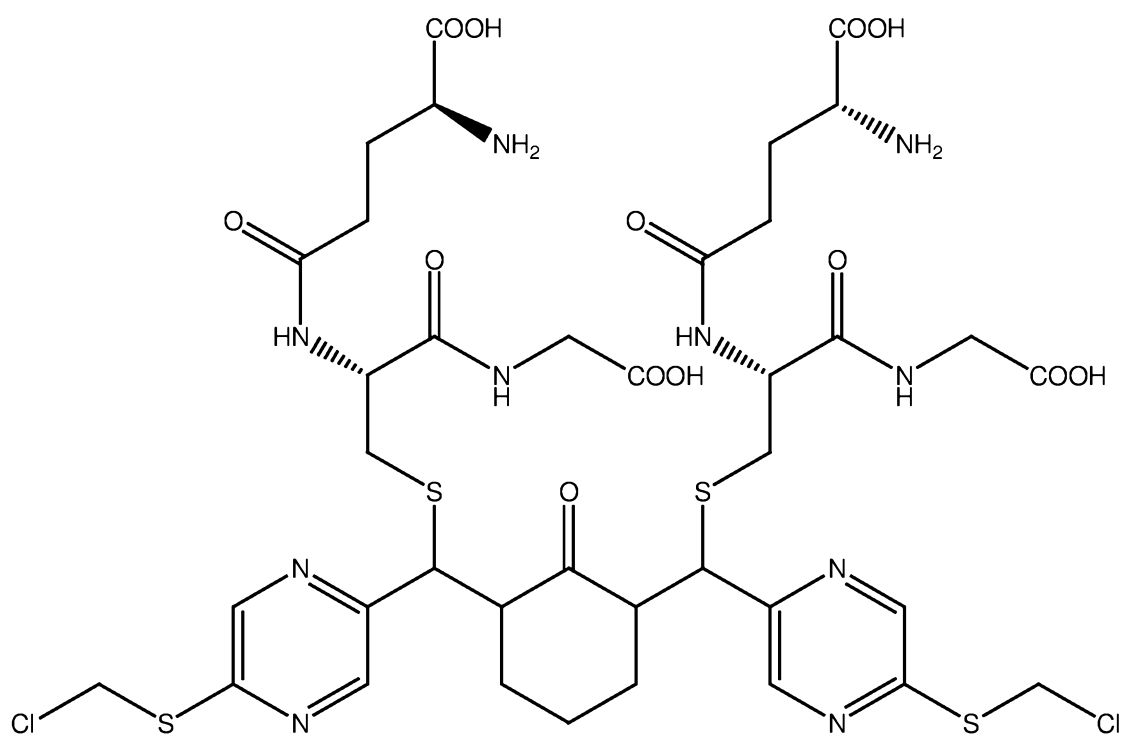
PB263 (glutathione adduct of PB260)
