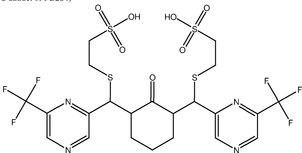
PB285 (NAC adduct of PB284)
