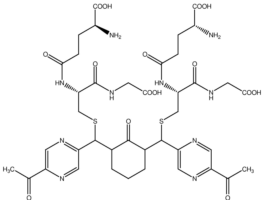
PB267 (glutathione adduct of PB264)
