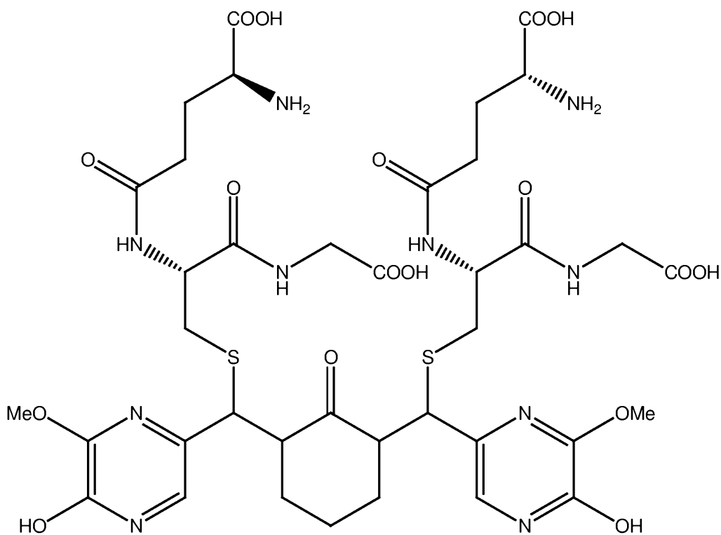
PB255 (glutathione adduct of PB252)
