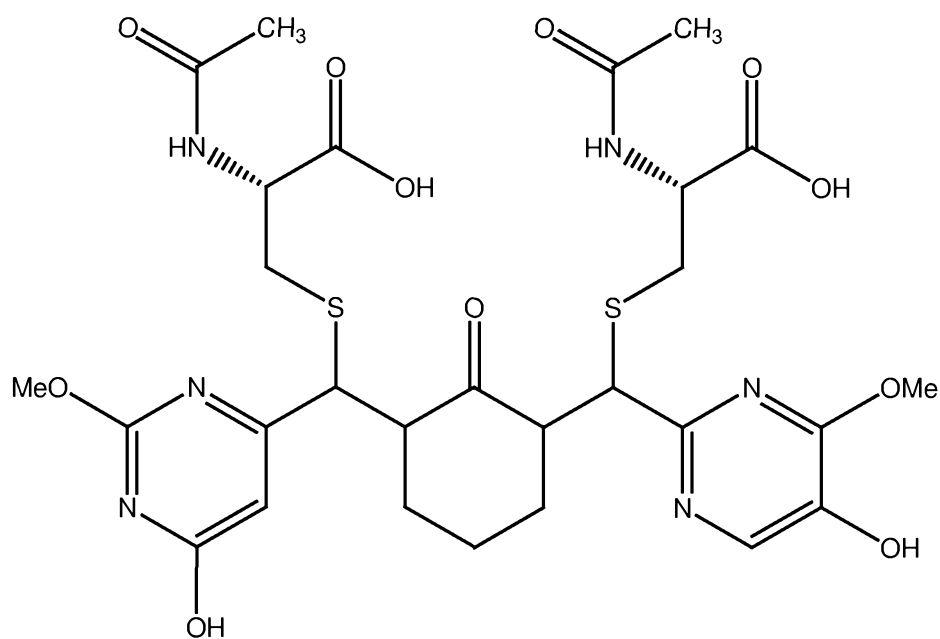
PB341 (NAC adduct of PB340)
