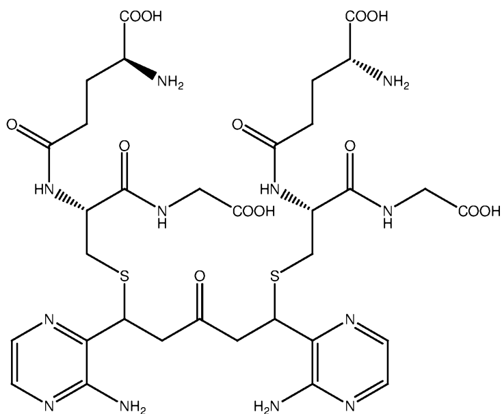
PB203 (glutathione adduct of PB200)
