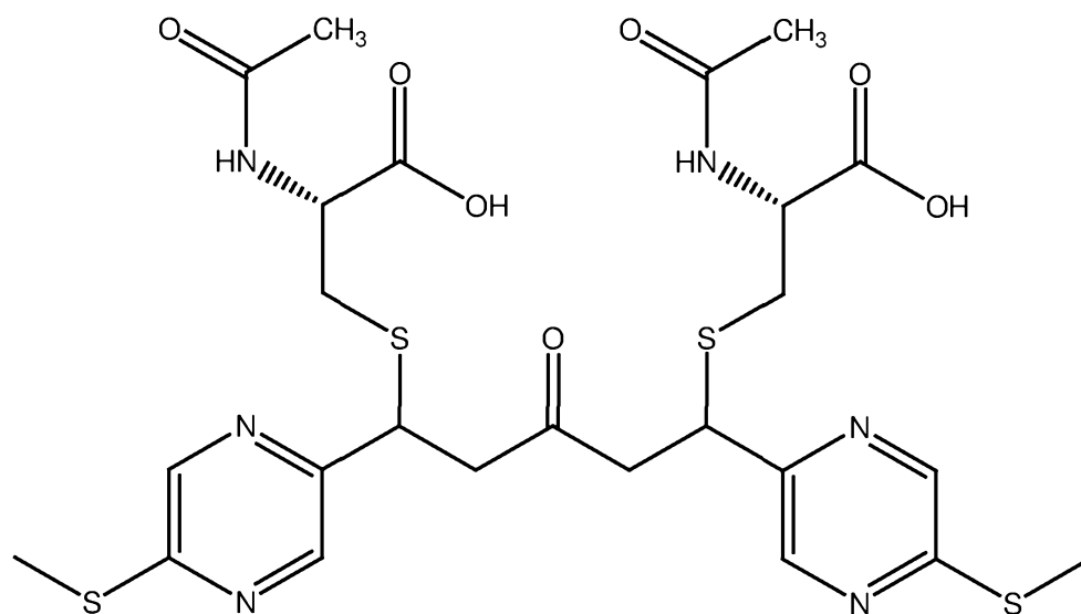
PB233 (NAC adduct of PB232)
