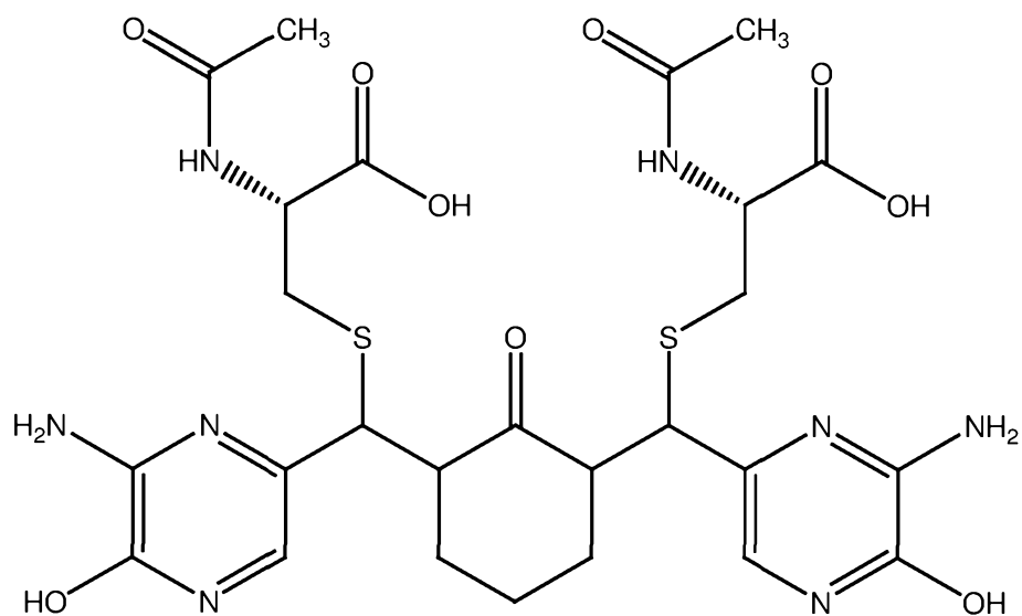
PB249 (NAC adduct of PB248)
