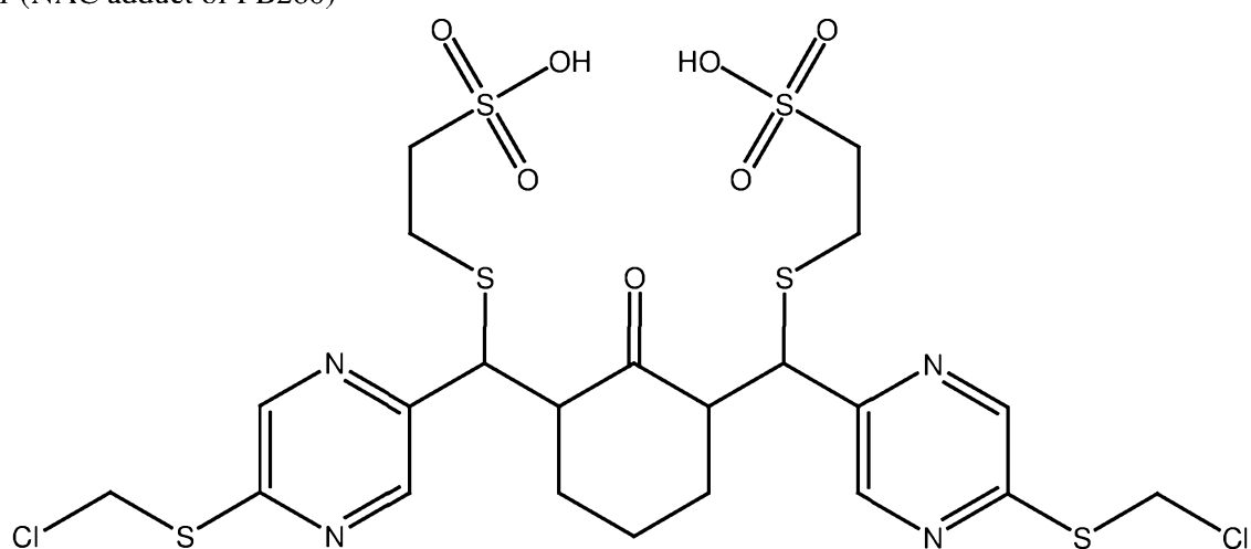
PB261 (NAC adduct of PB260)
