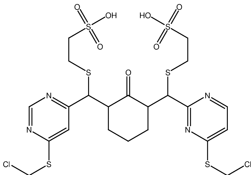
PB350 (mercaptoethanesulfonate adduct of PB348)
