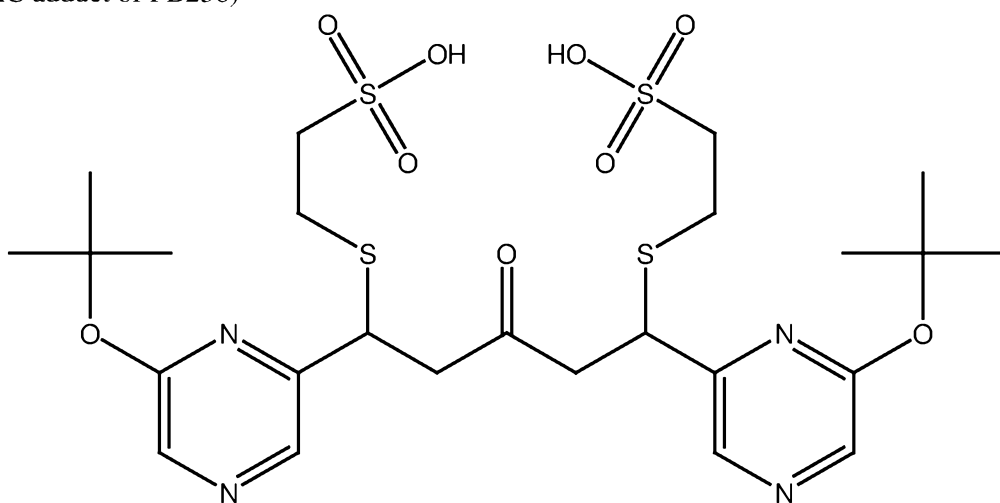
PB238 (mercaptoethanesulfonate adduct of PB236)
