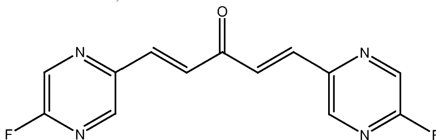
10 PB227 (glutathione adduct of PB224)
