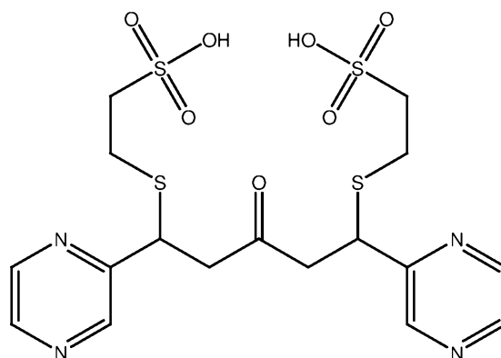
PB142 (mercaptoethane sulfonate adduct of PB137)
