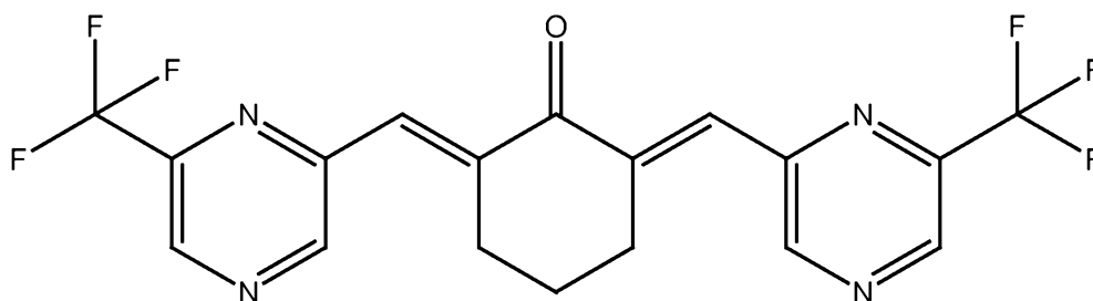
PB283 (glutathione adduct of PB280)
