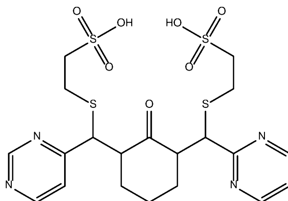
PB178 (mercaptoethanesulfonate adduct of PB171)
