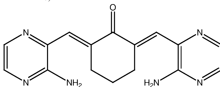
PB243 (glutathione adduct of PB240)
