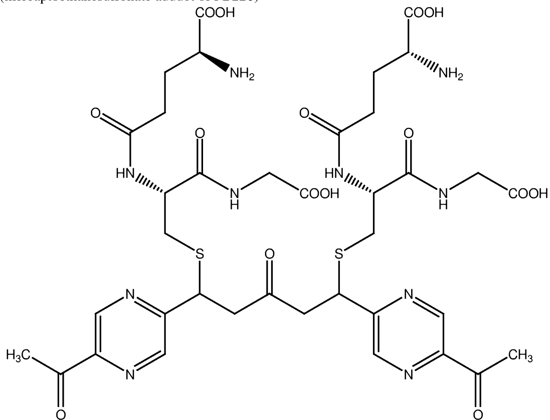
PB222 (mercaptoethanesulfonate adduct of PB220)
