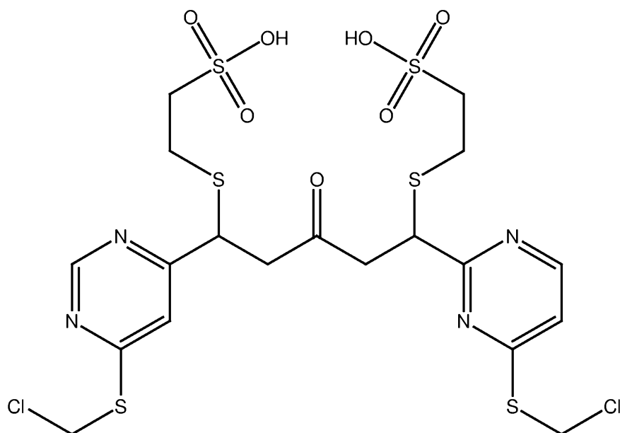
PB306 (mercaptoethanesulfonate adduct of PB304)
