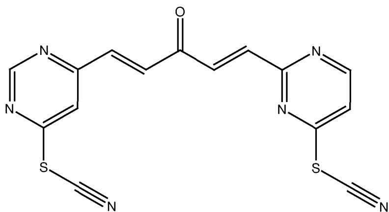
PB299 (glutathione adduct of PB296)
