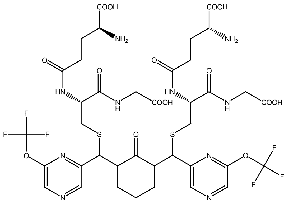
PB271 (glutathione adduct of PB268)
