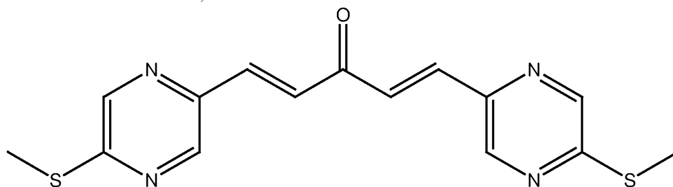
PB231 (glutathione adduct of PB228)
