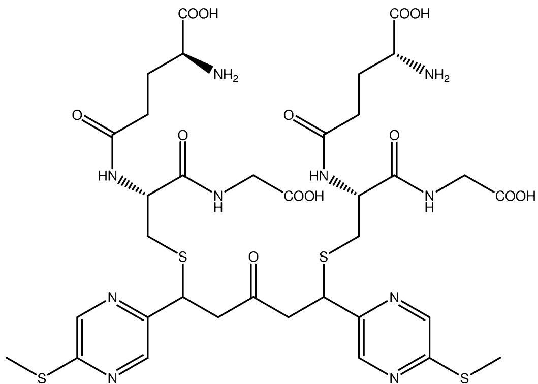
PB235 (glutathione adduct of PB 232)
