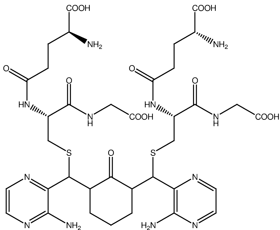
PB247 (glutathione adduct of PB244)
