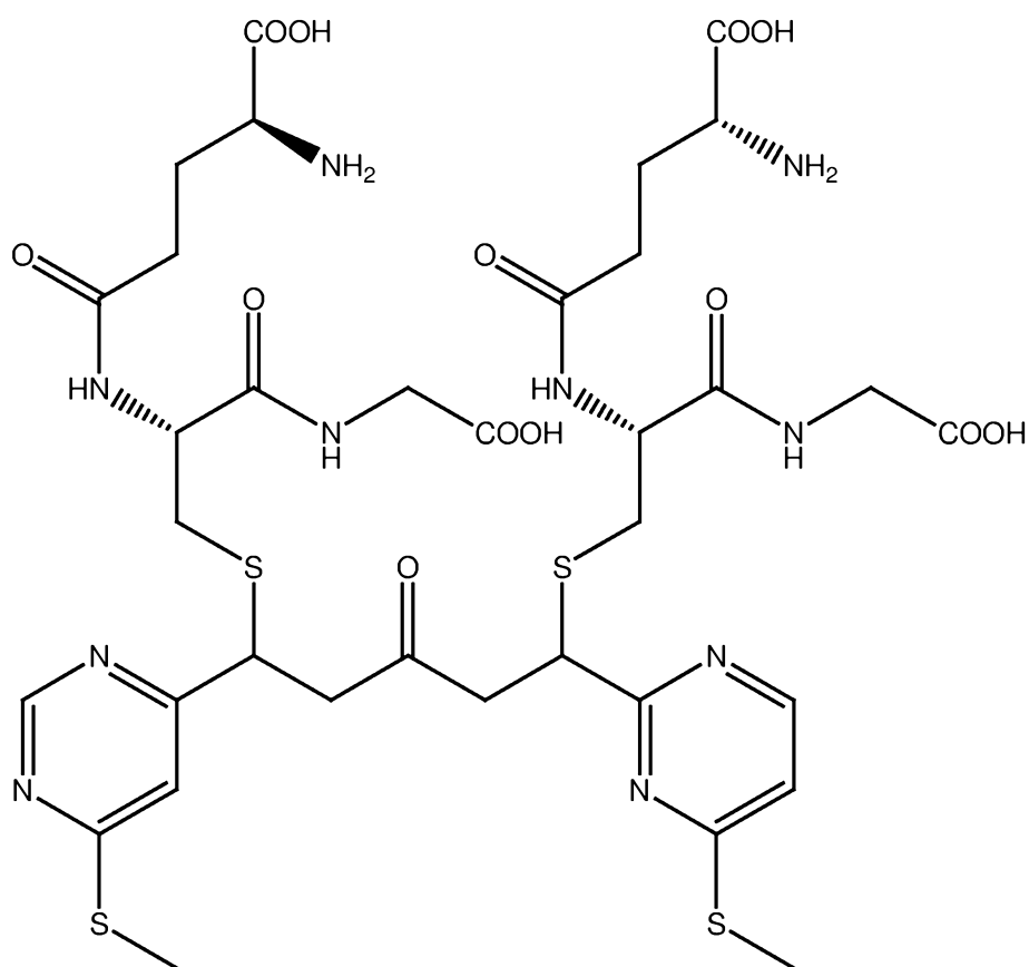
PB322 (mercaptoethanesulfonate adduct of PB320)
