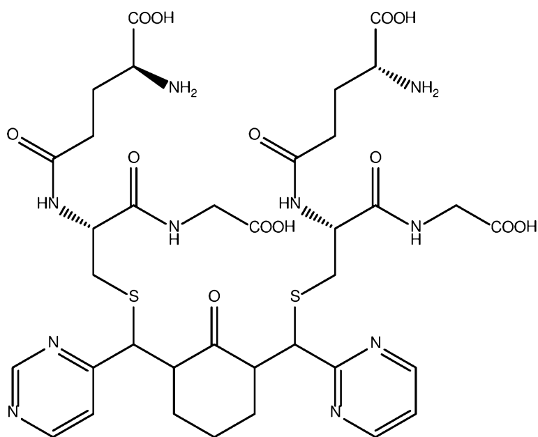
PB179 (glutathione adduct of PB171)
