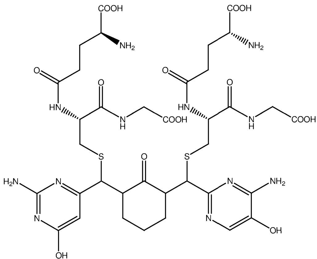
PB339 (glutathione adduct of PB336)
