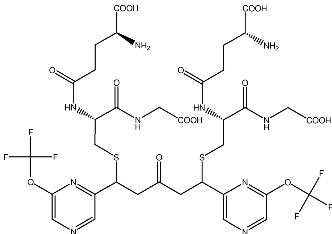
10 PB227 (glutathione adduct of PB224)
