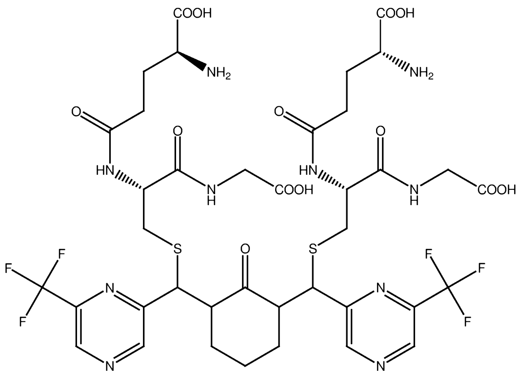
PB287 (glutathione adduct of PB284)
