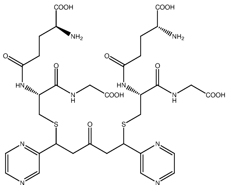
PB143 (glutathione adduct to PB137)
