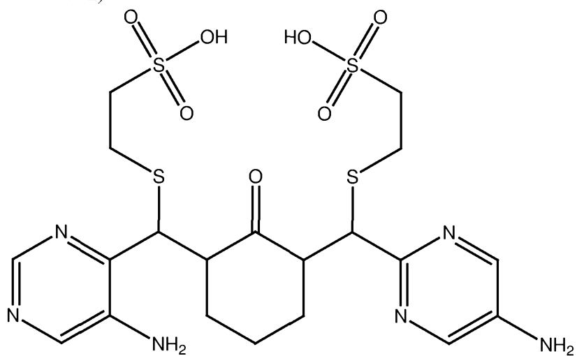
PB334 (mercaptoethanesulfonate adduct of PB332)
