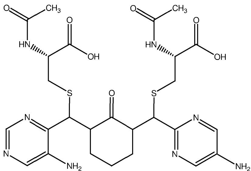
PB333 (NAC adduct of PB332)
