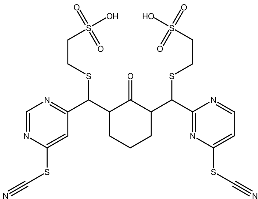
PB346 (mercaptoethanesulfonate adduct of PB344)
