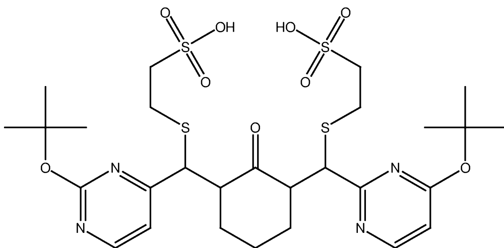
PB370 (mercaptoethanesulfonate adduct of PB368)
