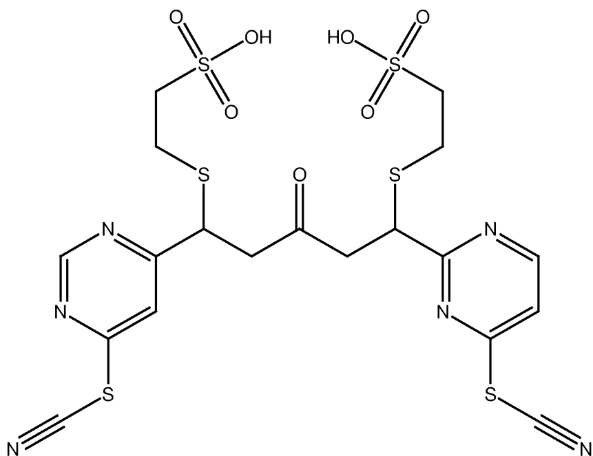
PB302 (mercaptoethanesulfonate adduct of PB300)
