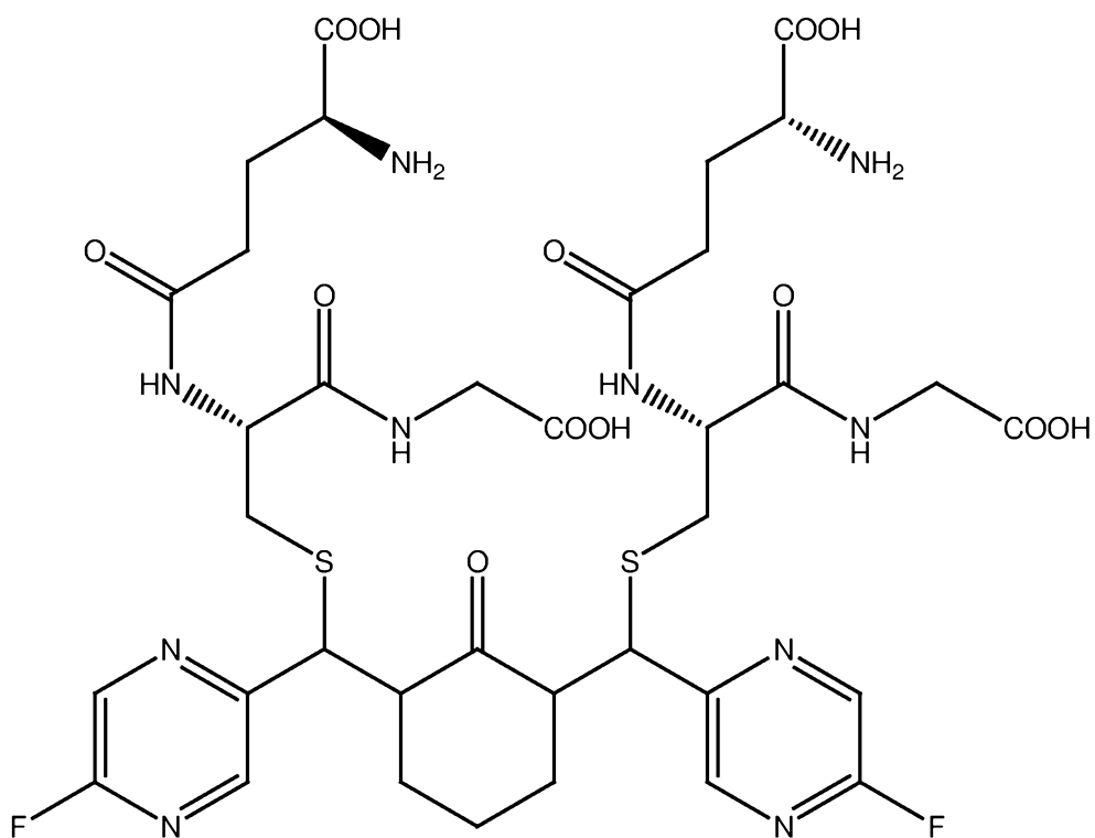
PB275 (glutathione adduct of PB272)
