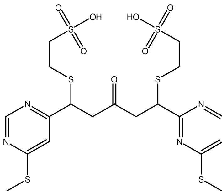
PB322 (mercaptoethanesulfonate adduct of PB320)
