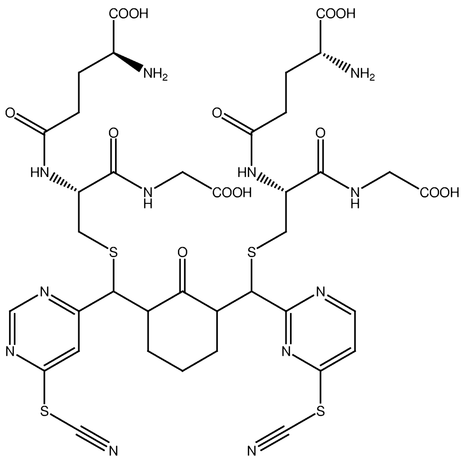
PB347 (glutathione adduct of PB344)
