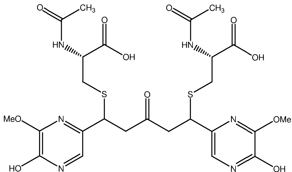
PB209 (NAC adduct of PB208)
