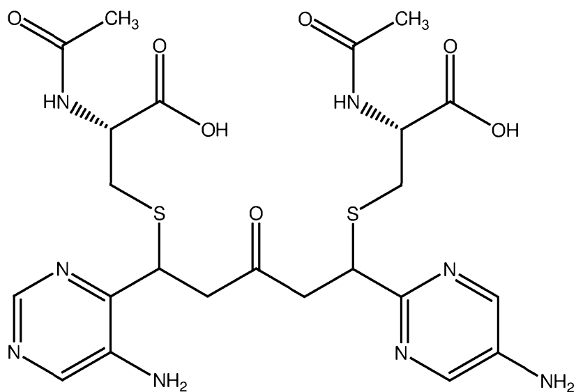
PB289 (NAC adduct of PB288)
