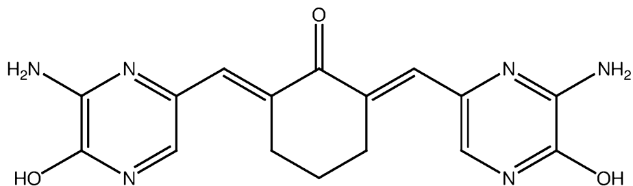
PB247 (glutathione adduct of PB244)
