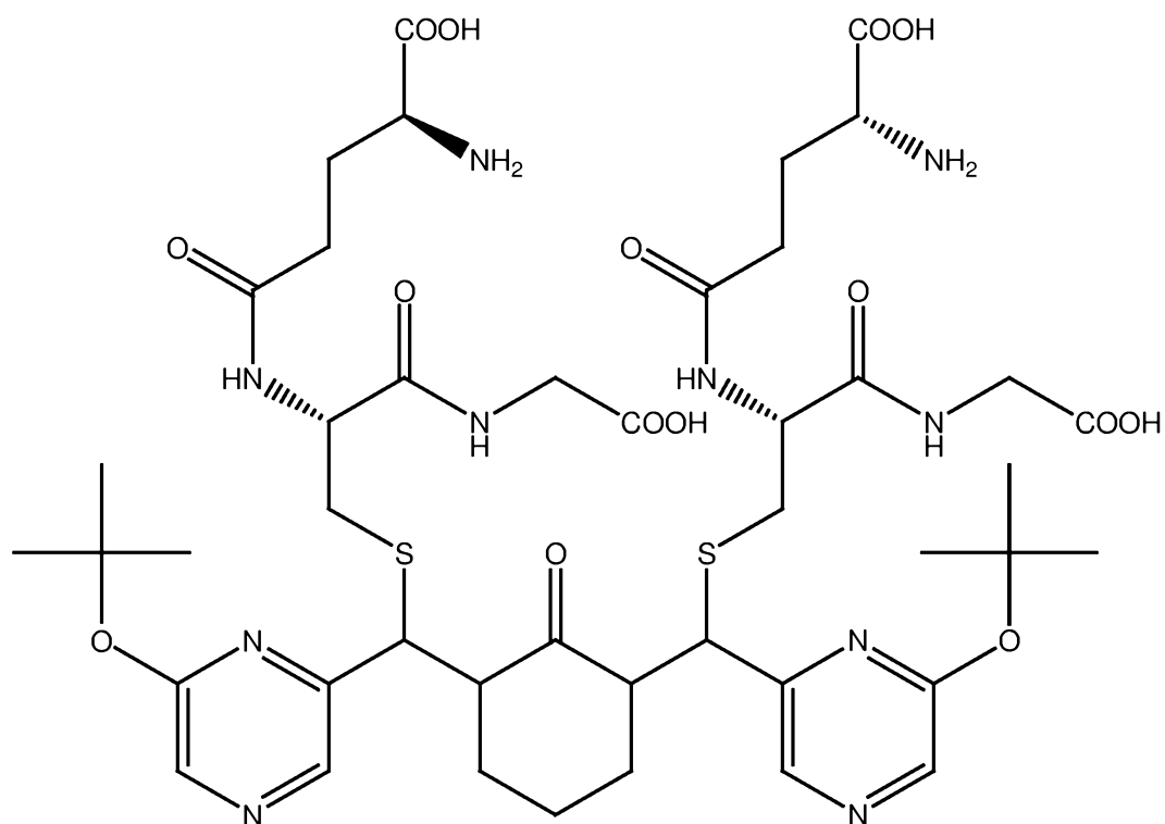
PB283 (glutathione adduct of PB280)
