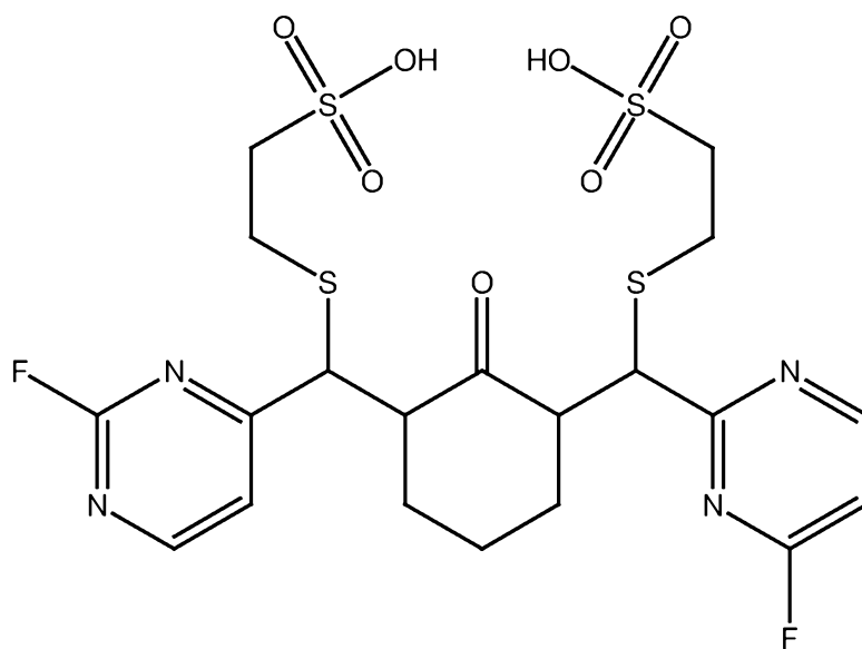
PB362 (mercaptoethanesulfonate adduct of PB360)
