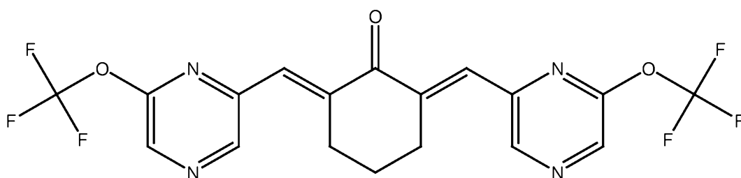
PB267 (glutathione adduct of PB264)
