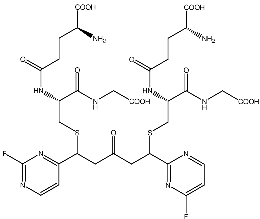
PB319 (glutathione adduct of PB316)
