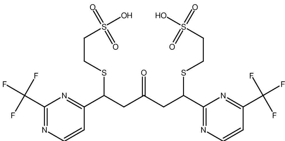
PB329 (NAC adduct of PB328)
