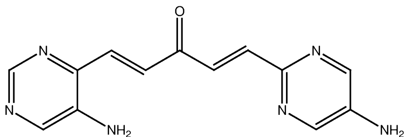
PB287 (glutathione adduct of PB284)
