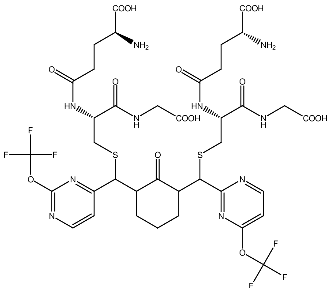
5 PB359 (glutathione adduct of PB356)
