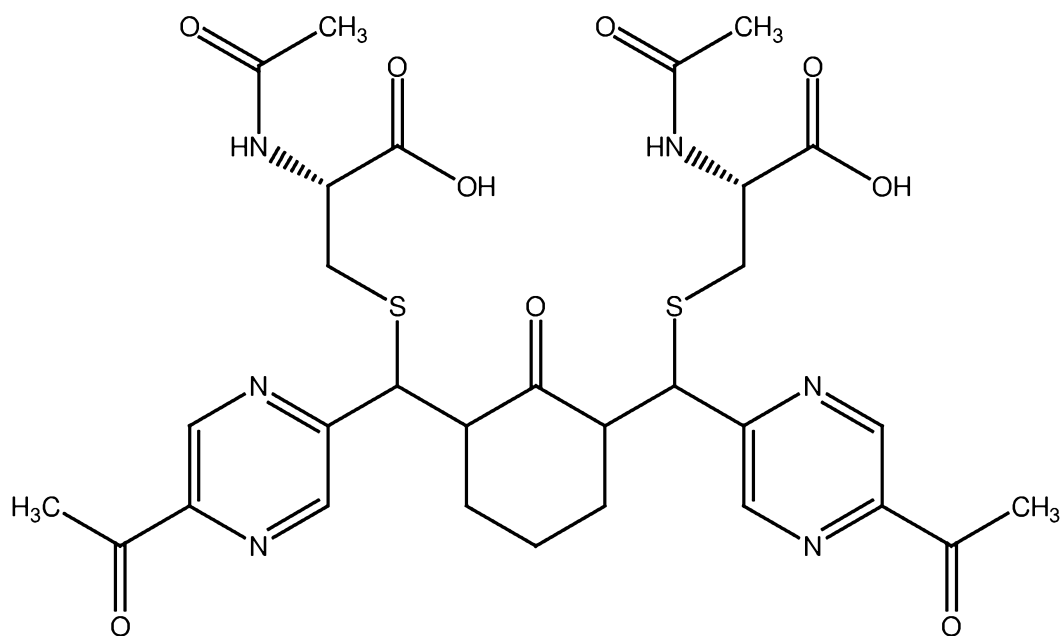
PB265 (NAC adduct of PB264)
