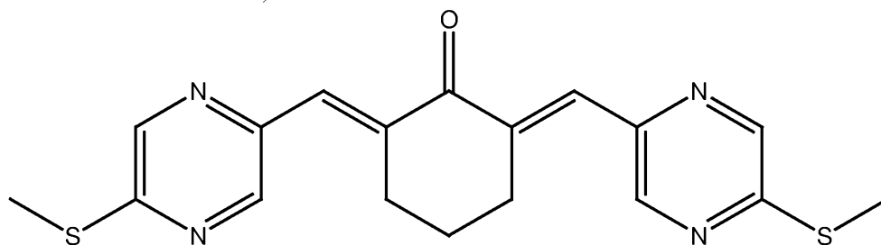
PB275 (glutathione adduct of PB272)
