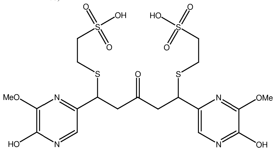
PB209 (NAC adduct of PB208)
