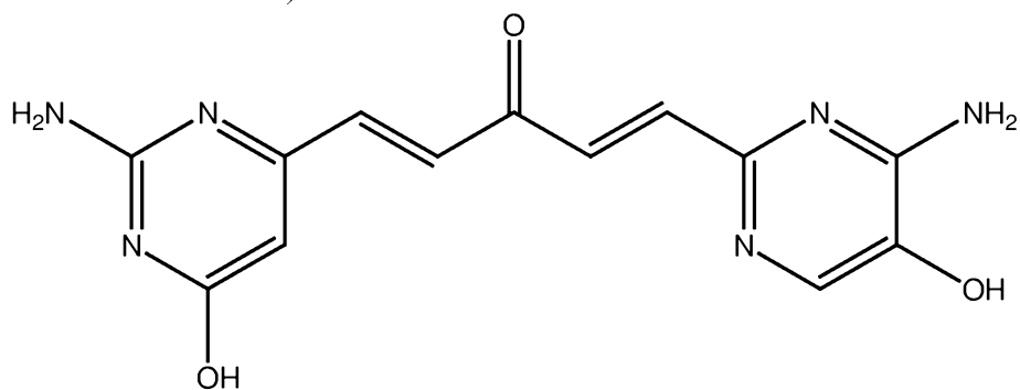
PB291 (glutathione adduct of PB288)
