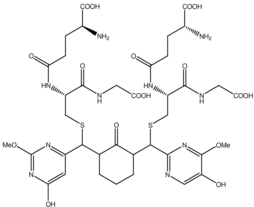
PB343 (glutathione adduct of PB340)
