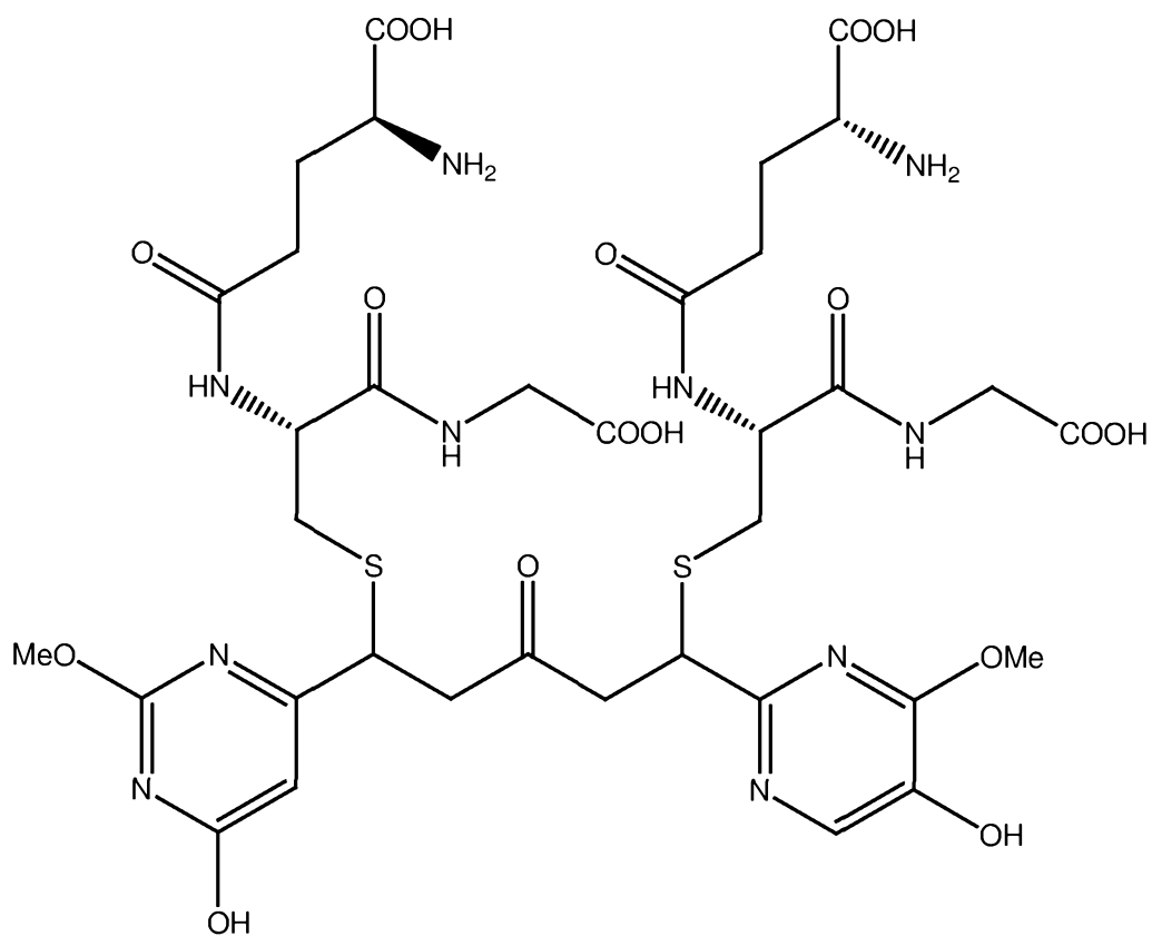
PB299 (glutathione adduct of PB296)
