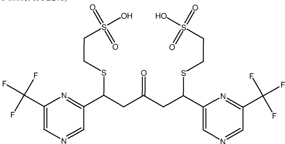
PB242 (mercaptoethanesulfonate adduct of PB240)
