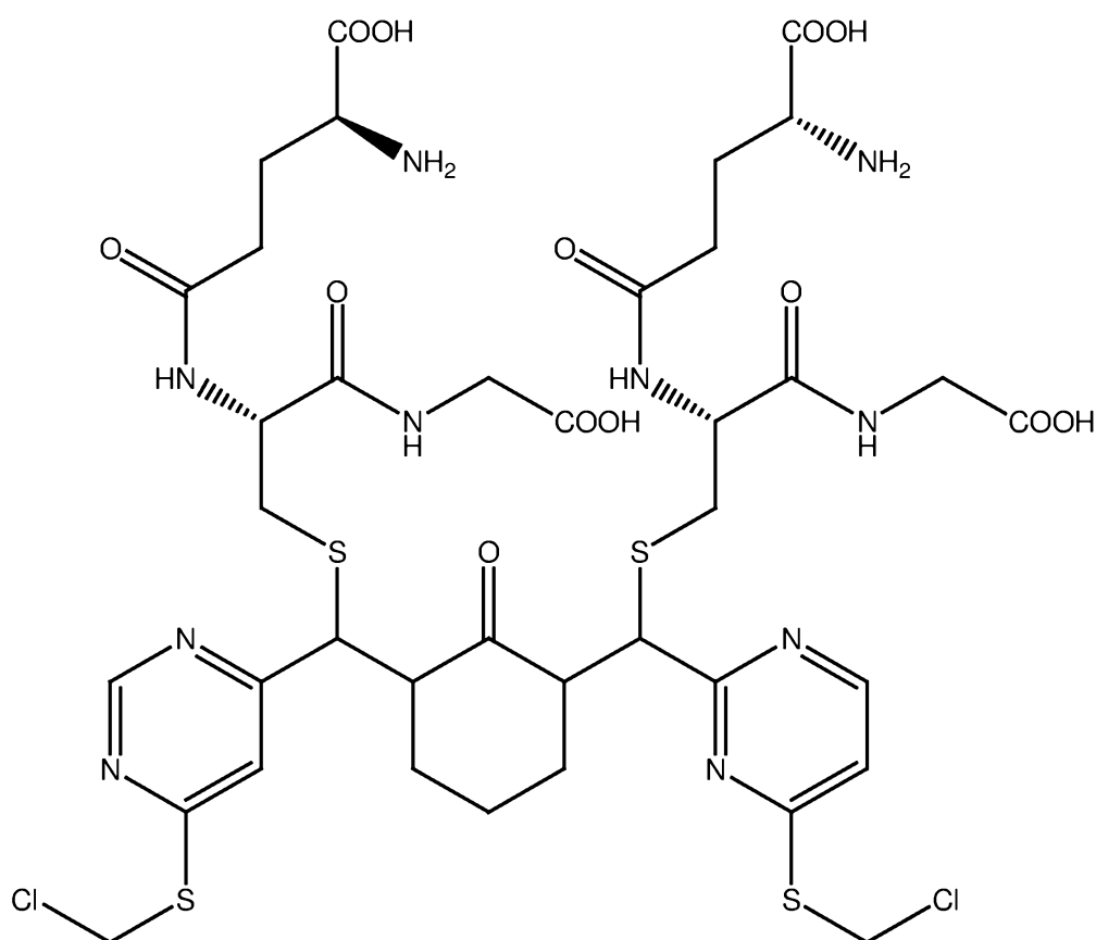
PB350 (mercaptoethanesulfonate adduct of PB348)
