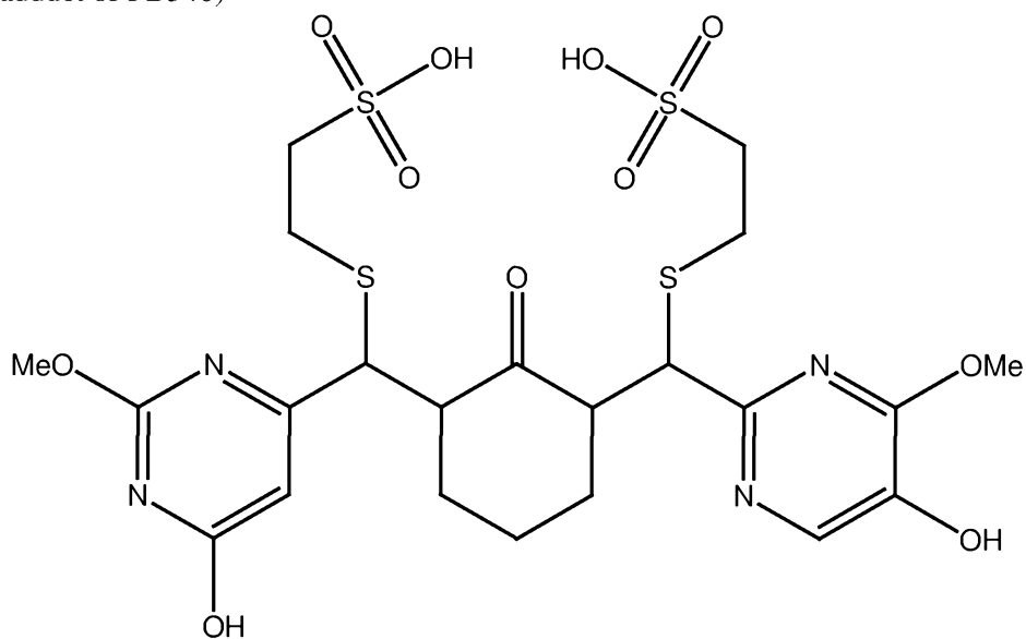
PB342 (mercaptoethanesulfonate adduct of PB340)
