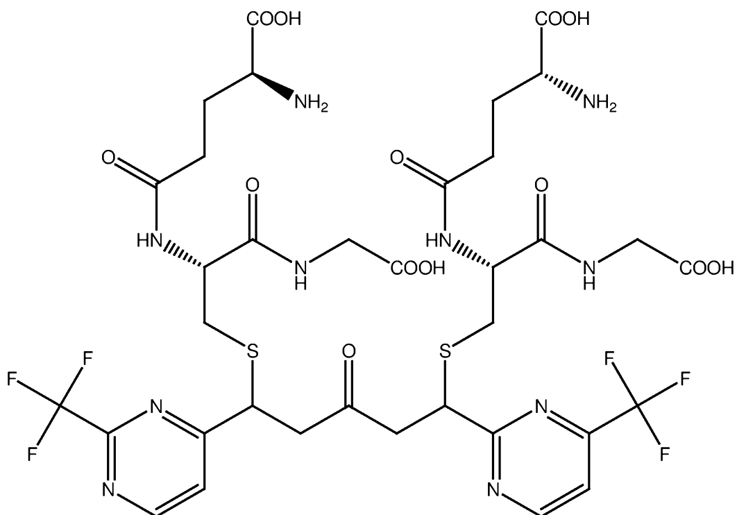
PB331 (glutathione adduct of PB328)
