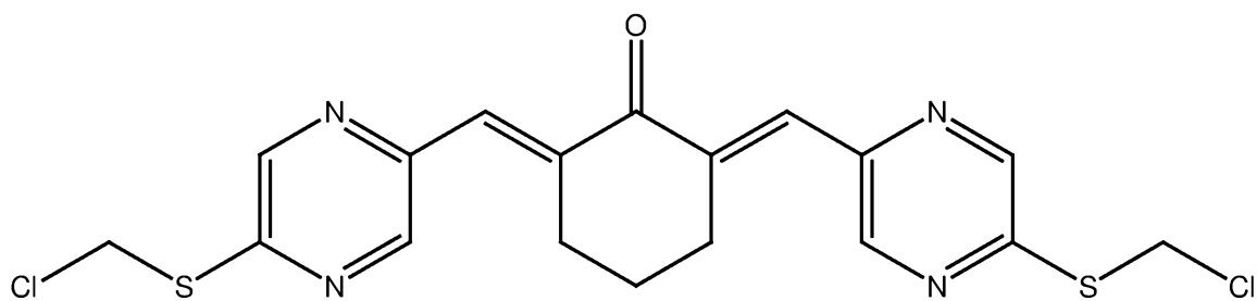
PB259 (glutathione adduct of PB256)
