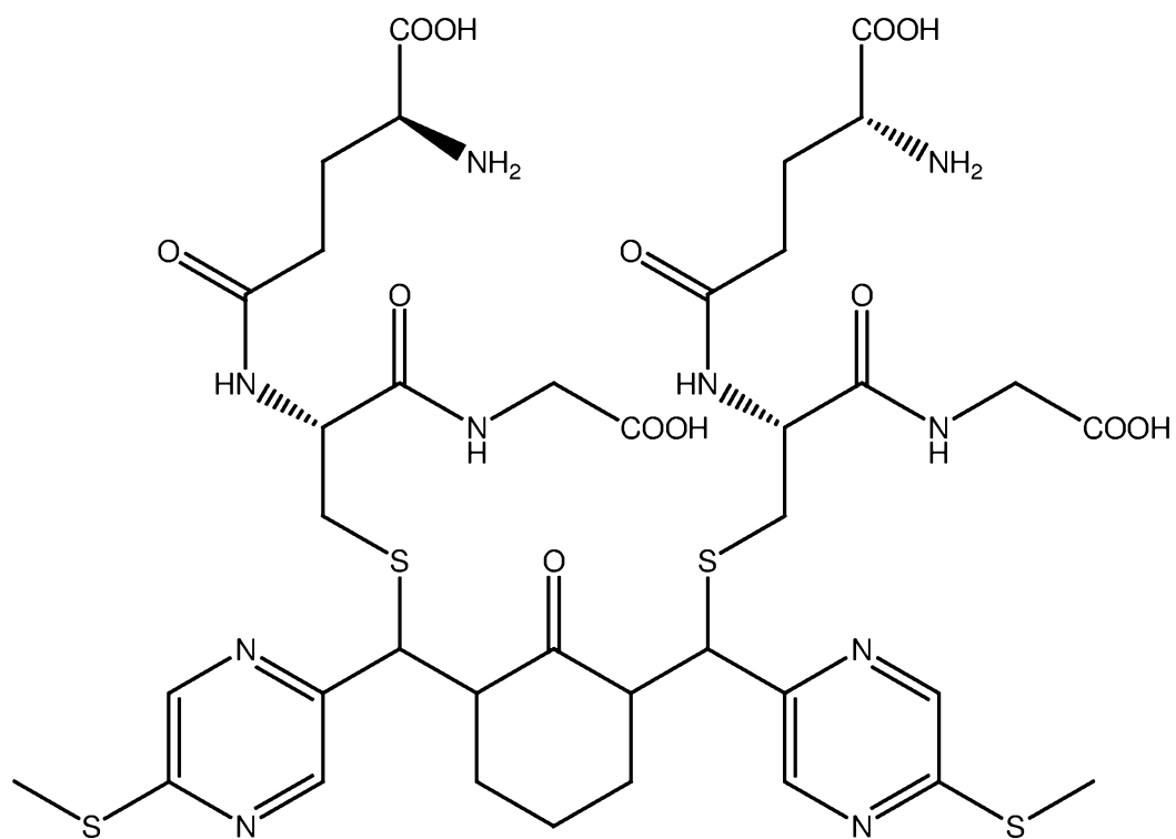
PB279 (glutathione adduct of PB276)
