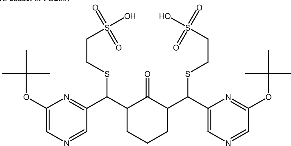
PB281 (NAC adduct of PB280)
