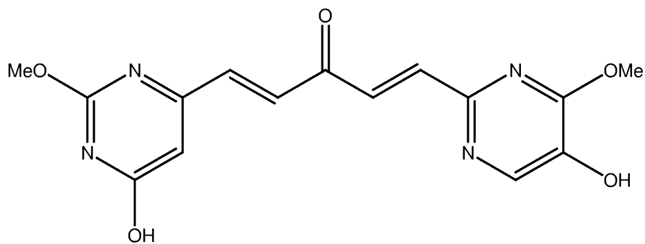
PB295 (glutathione adduct of PB292)
