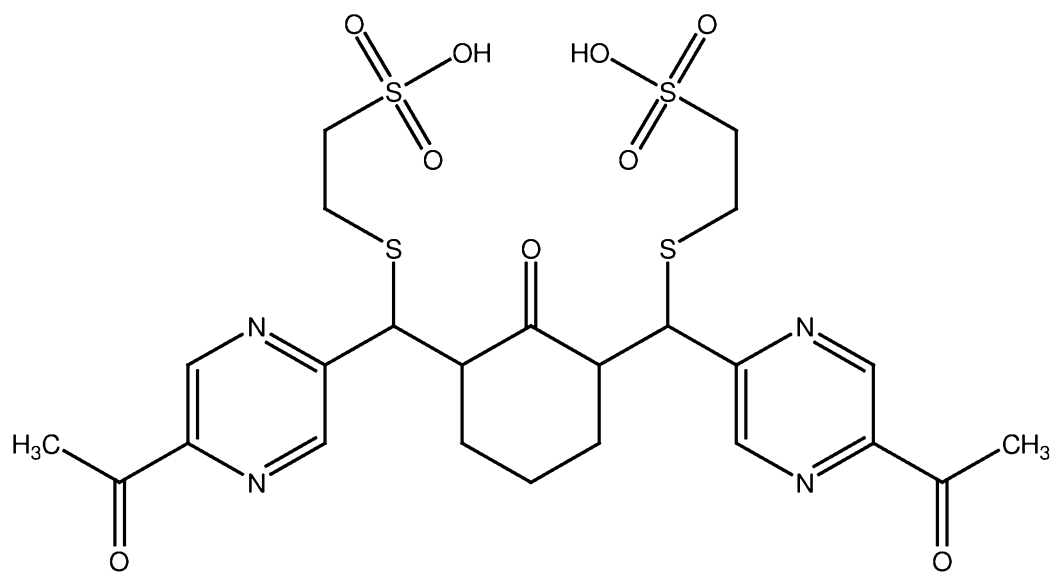
PB266 (mercaptoethanesulfonate adduct of PB264)
