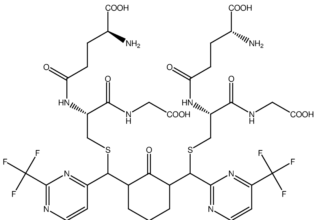
PB375 (glutathione adduct of PB372)
