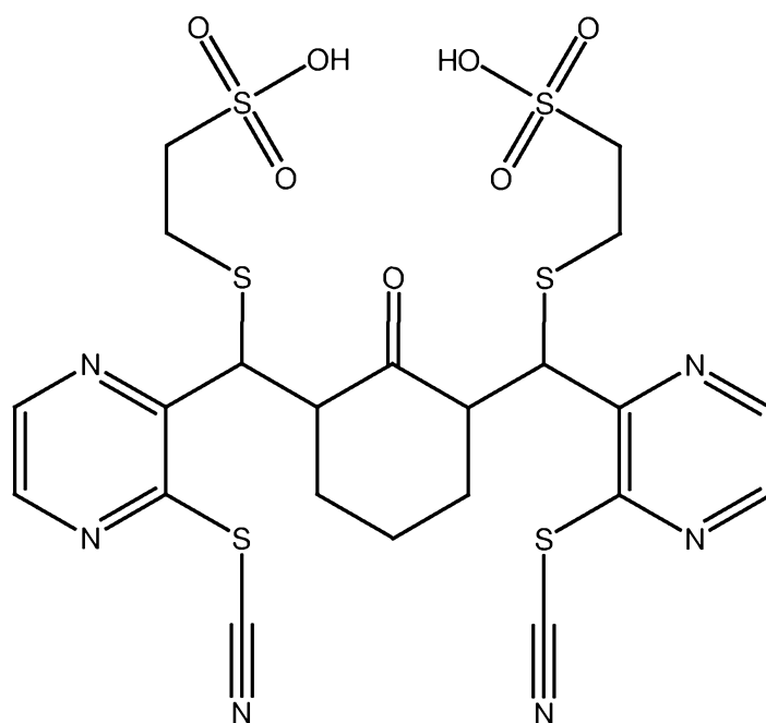
PB258 (mercaptoethanesulfonate adduct of PB256)
