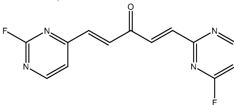
PB315 (glutathione adduct of PB312)
