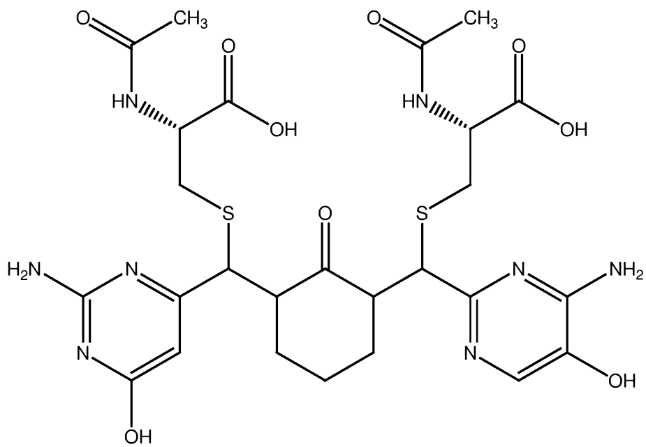
PB337 (NAC adduct of PB336)
