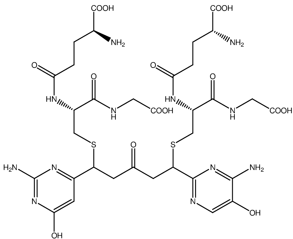
PB295 (glutathione adduct of PB292)
