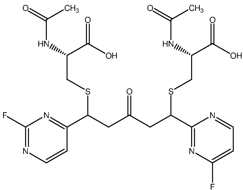
PB317 (NAC adduct of PB316)
