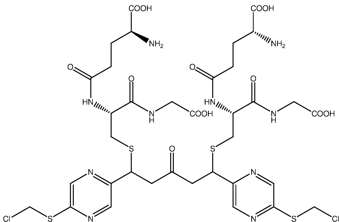
10 PB219 (glutathione adduct of PB216)
