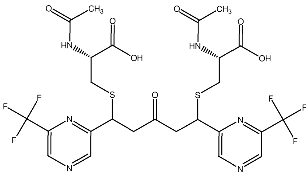
PB241 (NAC adduct of PB240)
