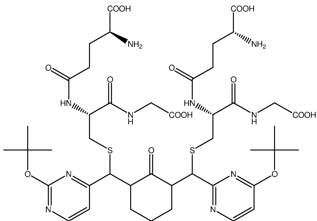
10 PB371 (glutathione adduct of PB368)
