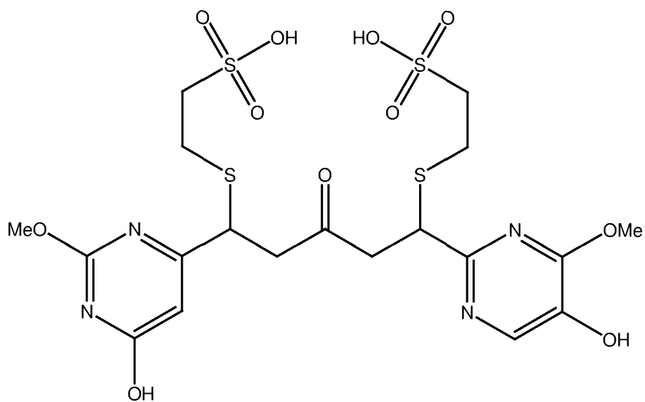
PB298 (mercaptoethanesulfonate adduct of PB296)
