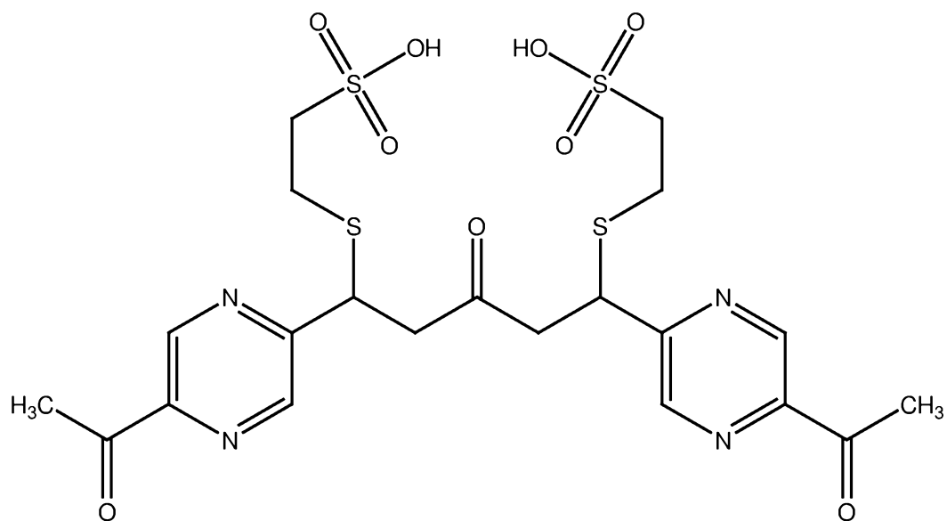
PB222 (mercaptoethanesulfonate adduct of PB220)
