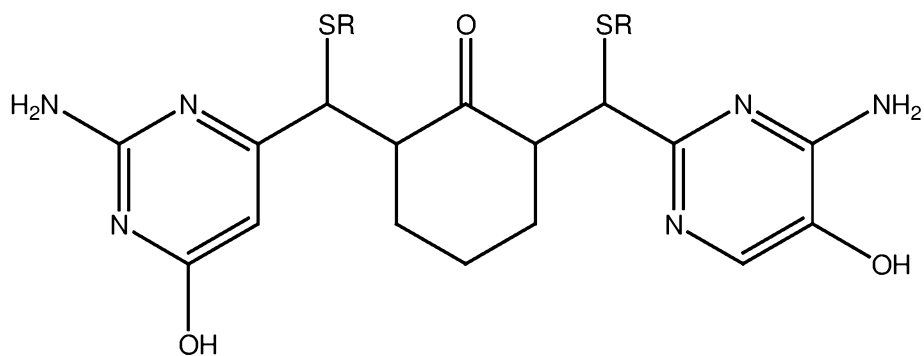
Thiol adduct of PB336, wherein -SR may be derived from N-acetylcysteine, 2-mercaptoethane sulfonate, glutathione, or another suitable thiol compound
