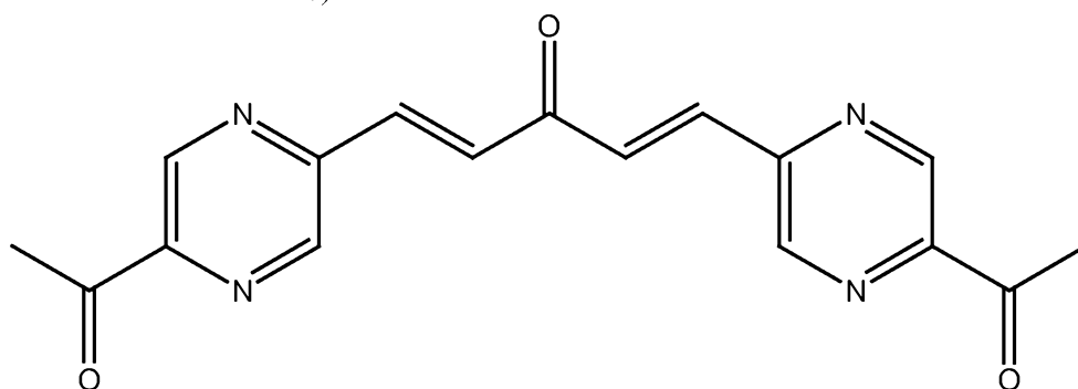
10 PB219 (glutathione adduct of PB216)
