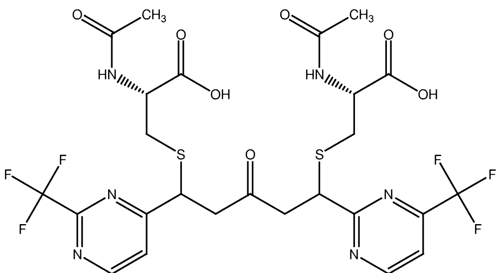
PB329 (NAC adduct of PB328)
