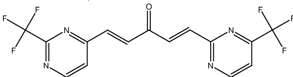
PB327 (glutathione adduct of PB324)
