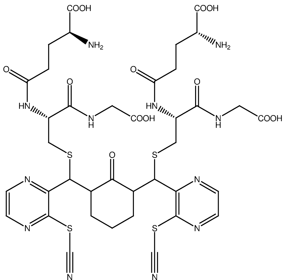
PB259 (glutathione adduct of PB256)
