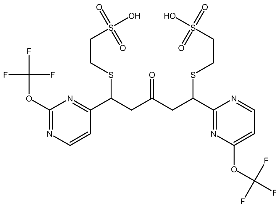
PB314 (mercaptoethanesulfonate adduct of PB312)
