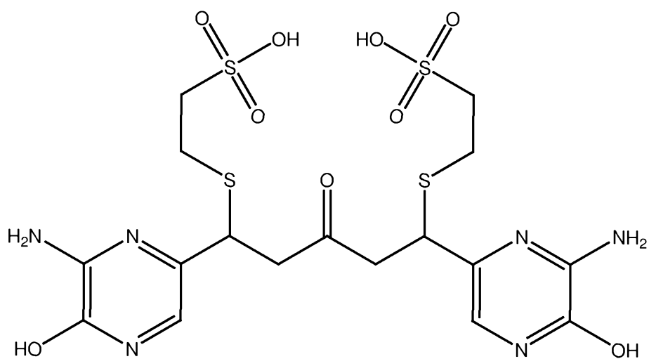
PB205 (NAC adduct of PB204)
