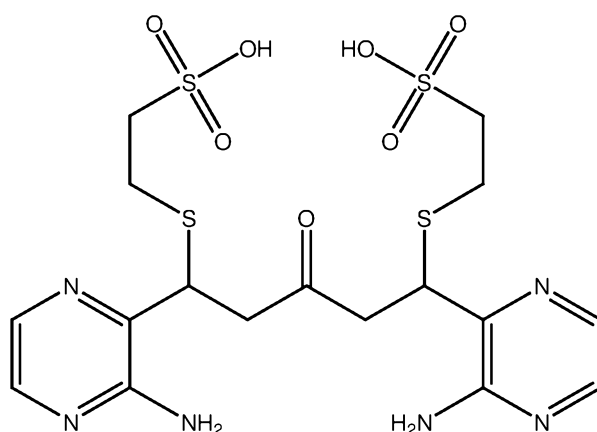
PB202 (mercaptoethanesulfonate adduct of PB200)
