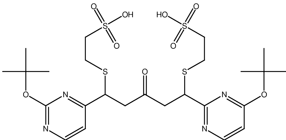
PB326 (mercaptoethanesulfonate adduct of PB324)
