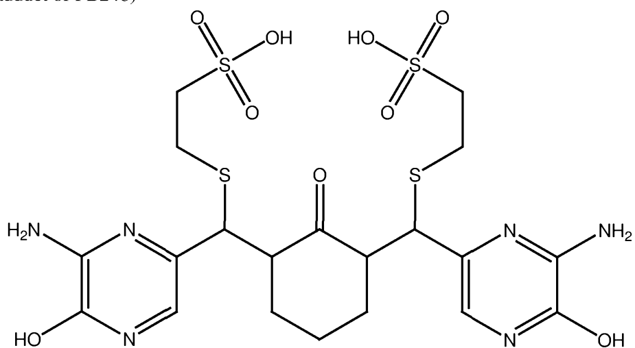
PB249 (NAC adduct of PB248)
