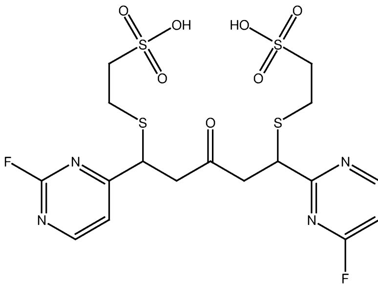
PB318 (mercaptoethanesulfonate adduct of PB316)
