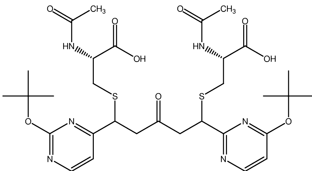
PB325 (NAC adduct of PB324)
