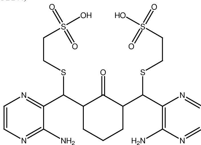
PB246 (mercaptoethanesulfonate adduct of PB244)
