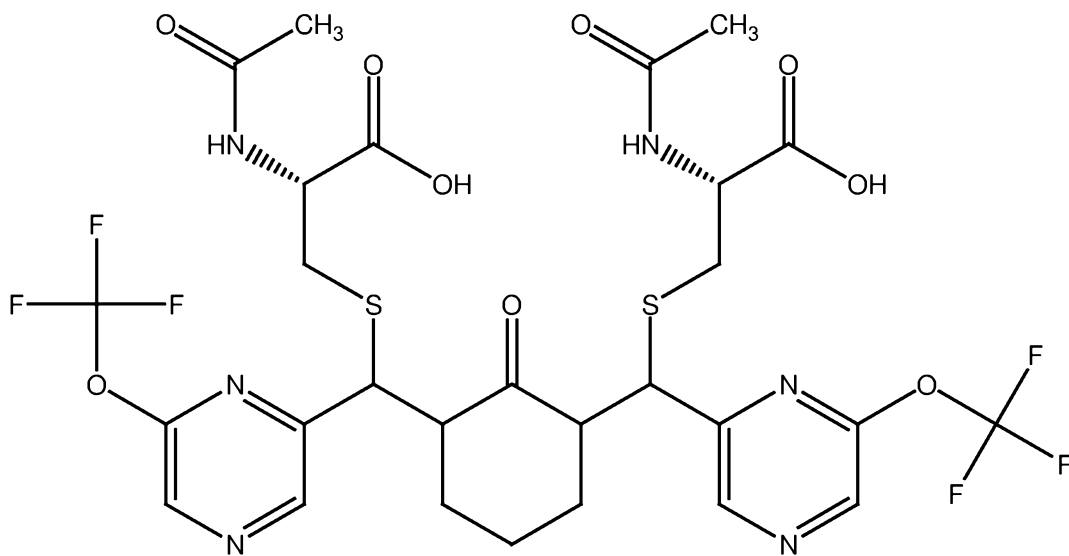
PB269 (NAC adduct of PB268)
