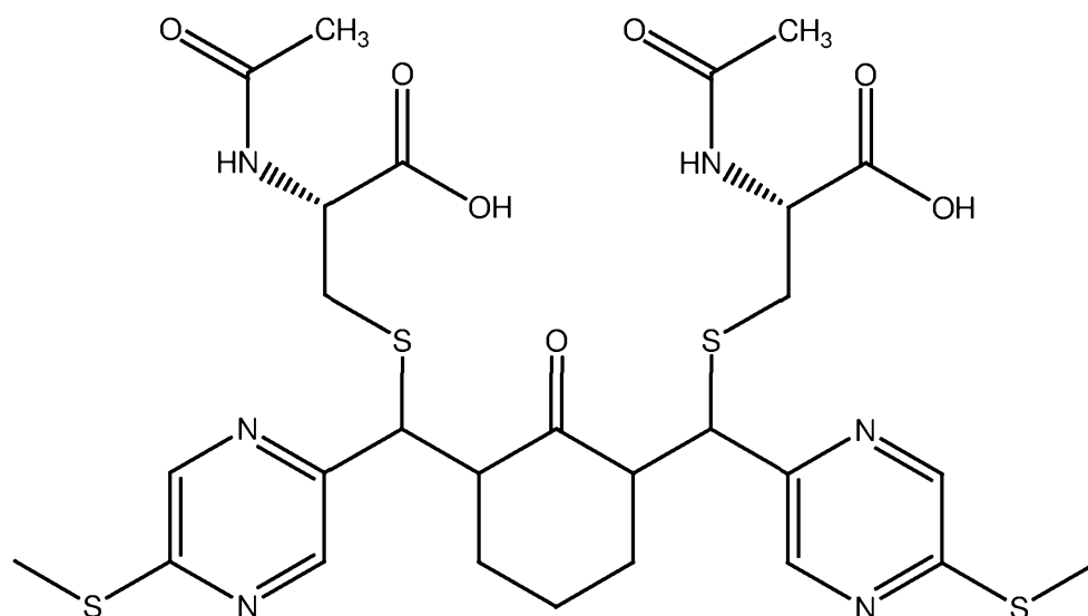
PB277 (NAC adduct of PB276)
