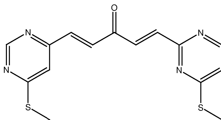
PB319 (glutathione adduct of PB316)
