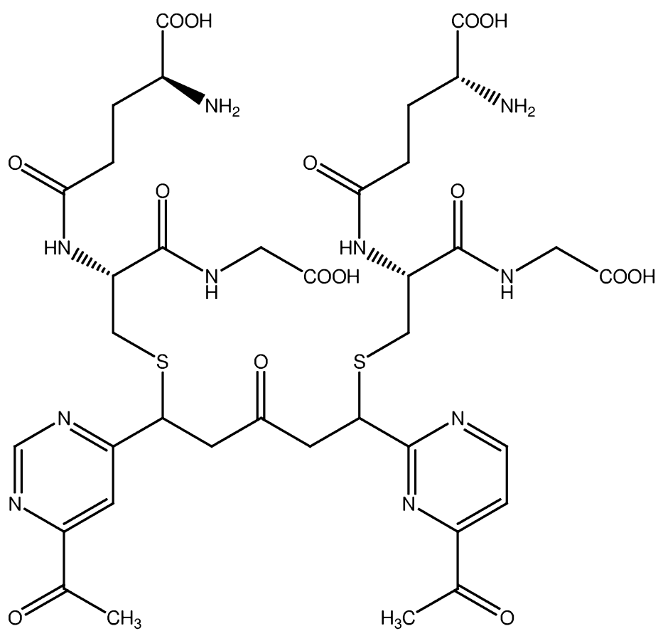
PB311 (glutathione adduct of PB308)
