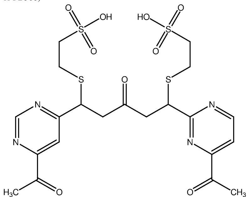
PB309 (NAC adduct of PB308)
