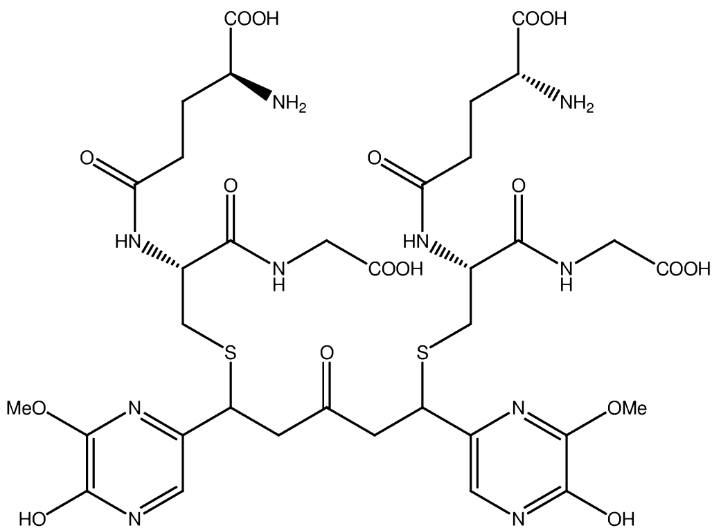
PB211 (glutathione adduct of PB208)
