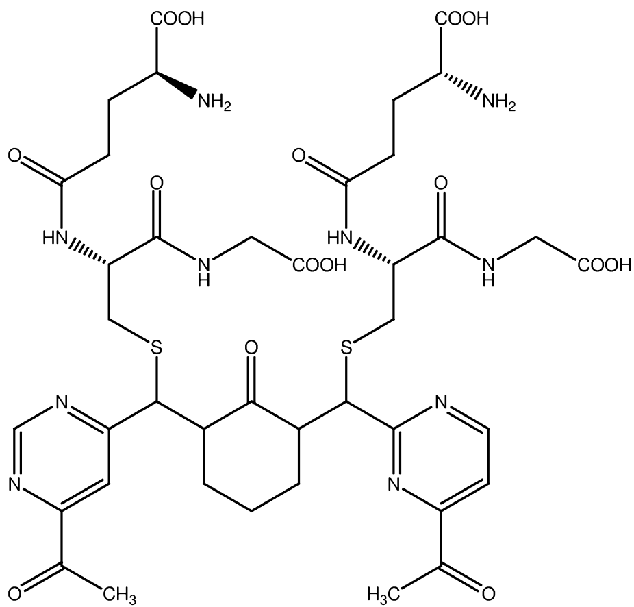
PB355 (glutathione adduct of PB352)
