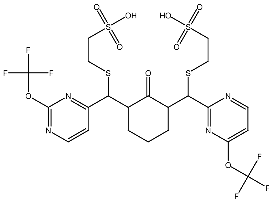
PB358 (mercaptoethanesulfonate adduct of PB356)
