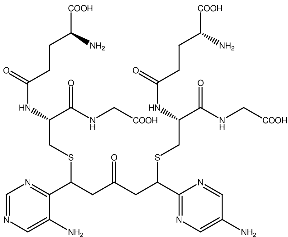
PB291 (glutathione adduct of PB288)
