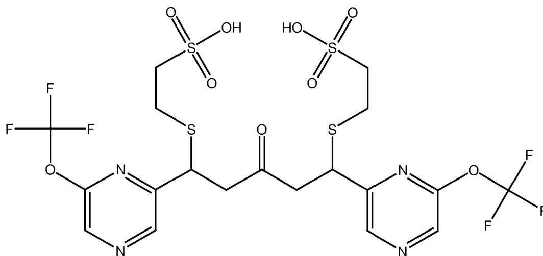
PB226 (mercaptoethanesulfonate adduct of PB224)
