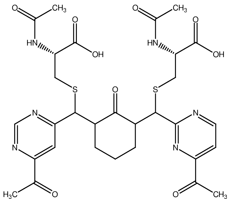
PB353 (NAC adduct of PB352)
