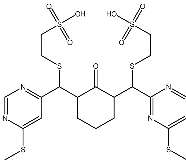
PB366 (mercaptoethanesulfonate adduct of PB364)
