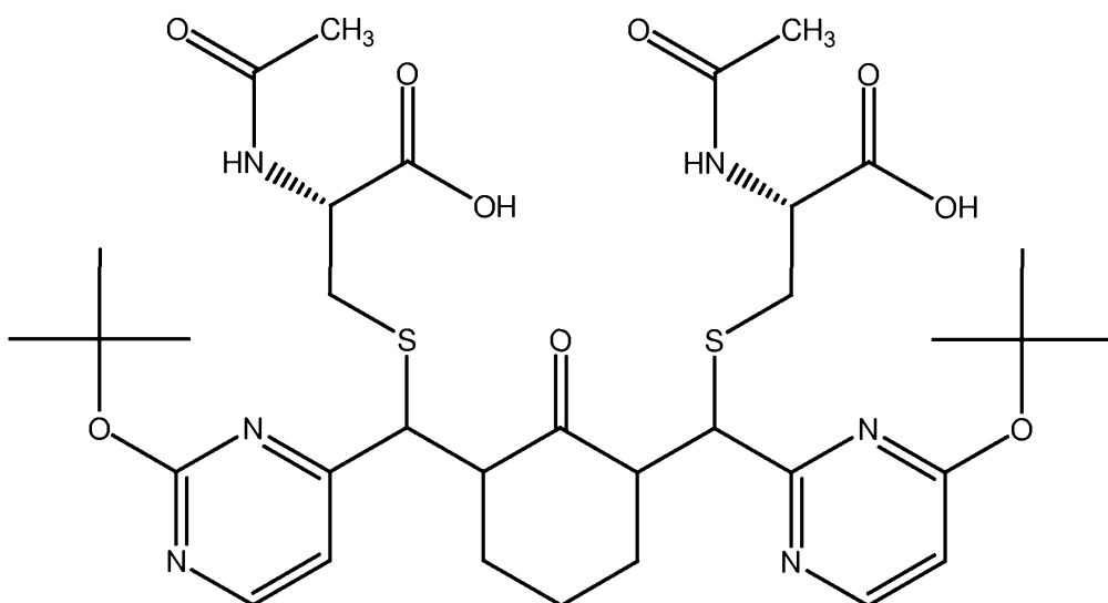
15 PB369 (NAC adduct of PB368)
