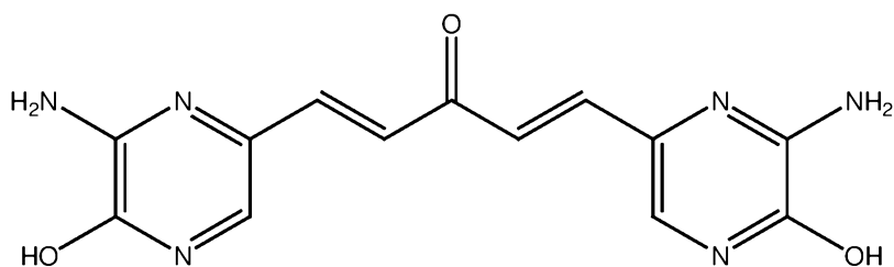
PB203 (glutathione adduct of PB200)
