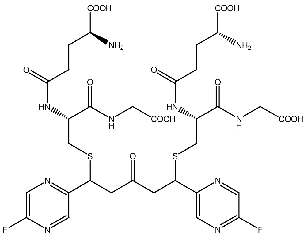
PB231 (glutathione adduct of PB228)
