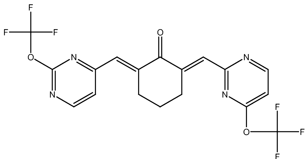
PB355 (glutathione adduct of PB352)
