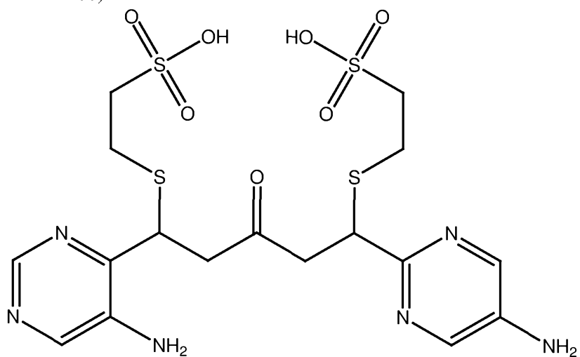
PB290 (mercaptoethanesulfonate adduct of PB288)
