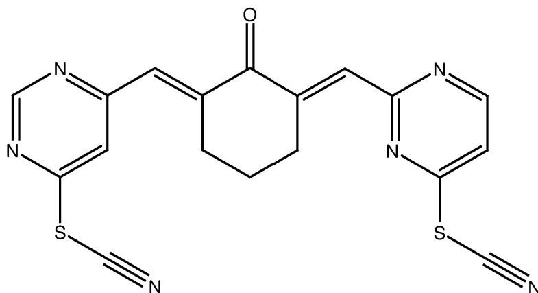
PB343 (glutathione adduct of PB340)
