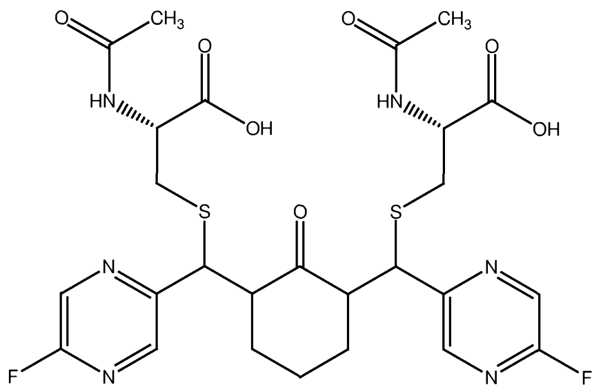
PB273 (NAC adduct PB272)
