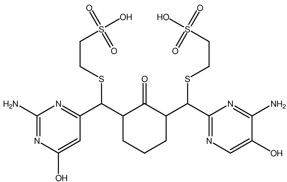
PB338 (mercaptoethanesulfonate adduct of PB336)
