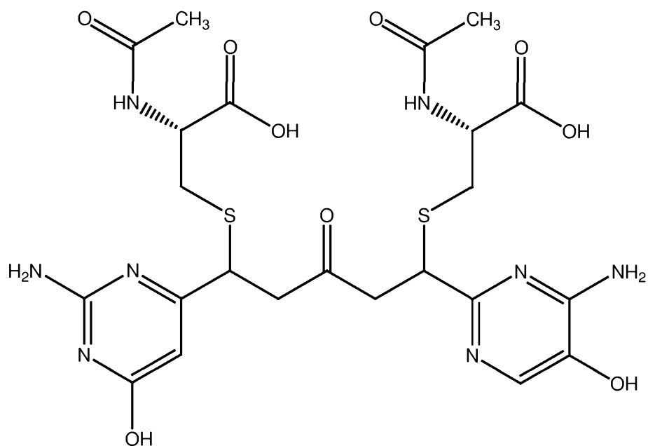
PB293 (NAC adduct of PB292)
