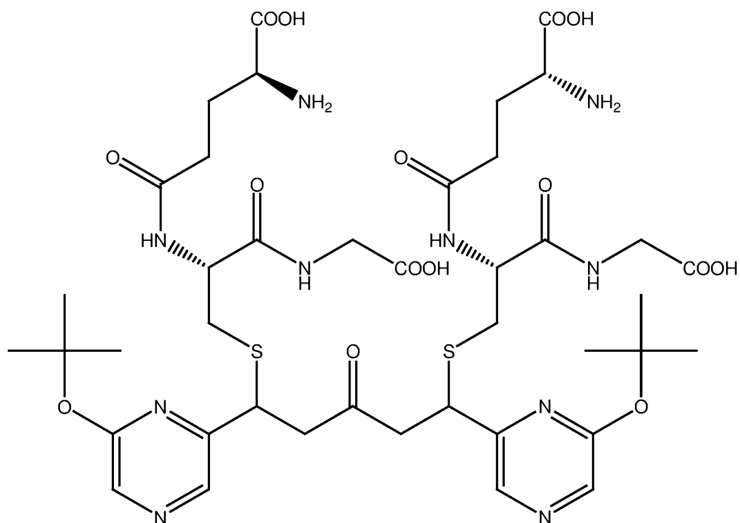
PB239 (glutathione adduct of PB236)
