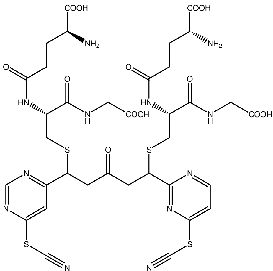
PB303 (glutathione adduct of PB300)
