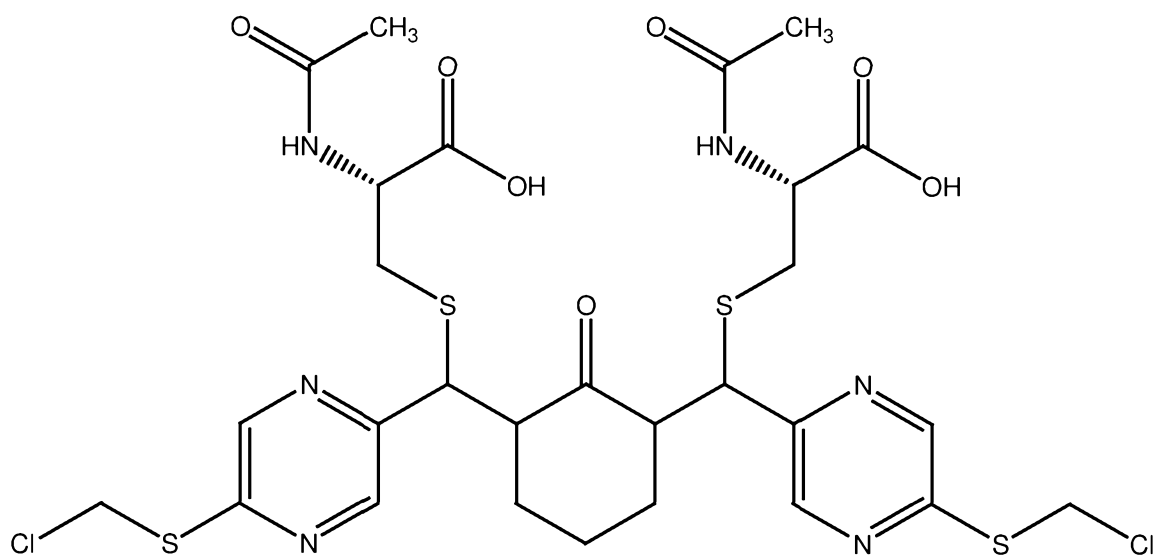
PB261 (NAC adduct of PB260)
