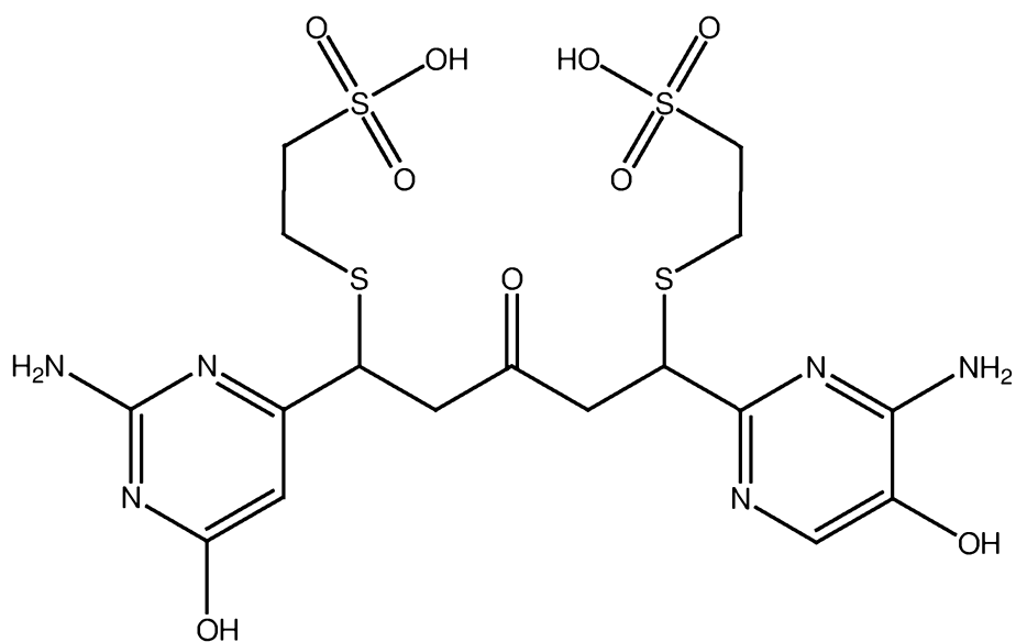
PB294 (mercaptoethanesulfonate adduct of PB292)
