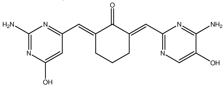
PB335 (glutathione adduct of PB332)
