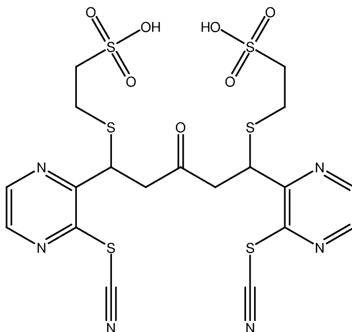
PB214 (mercaptoethanesulfonate adduct of PB212)
