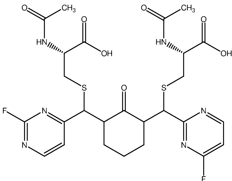
PB361 (NAC adduct of PB360)
