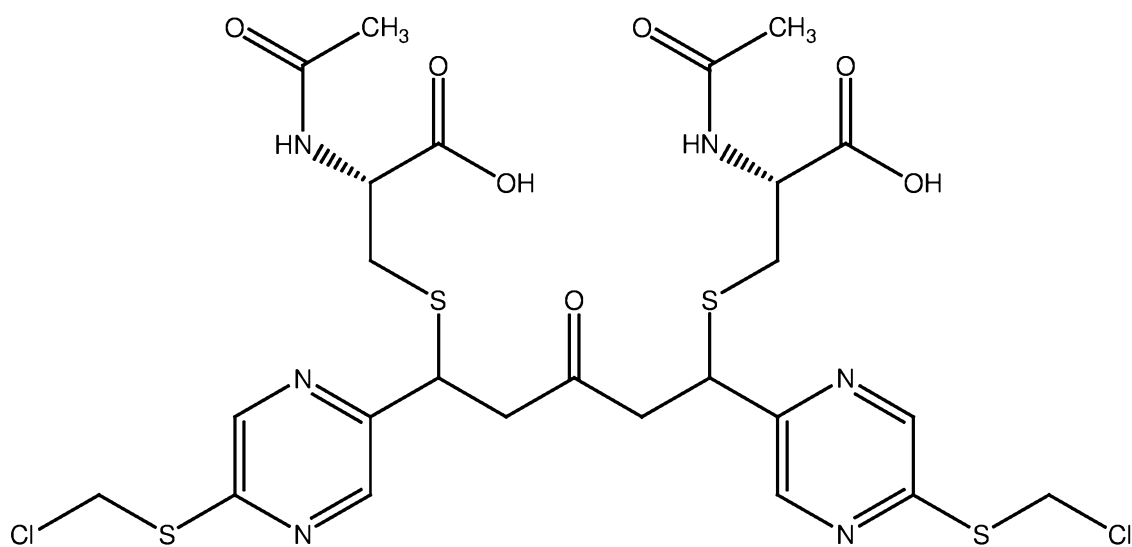
15 PB217 (NAC adduct of PB216)
