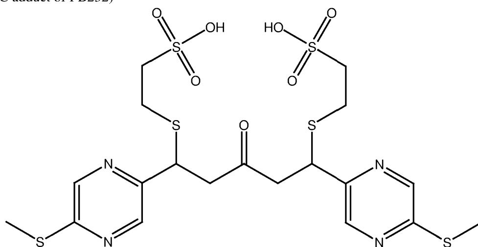
PB233 (NAC adduct of PB232)
