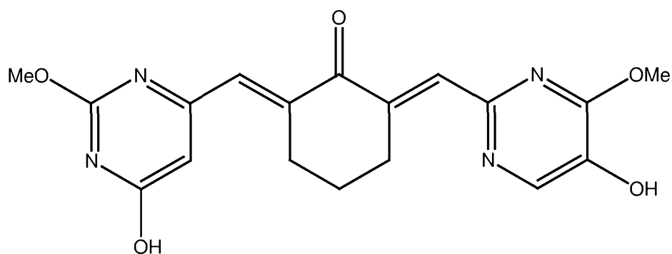
PB339 (glutathione adduct of PB336)
