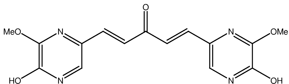
PB207 (glutathione adduct of PB204)
