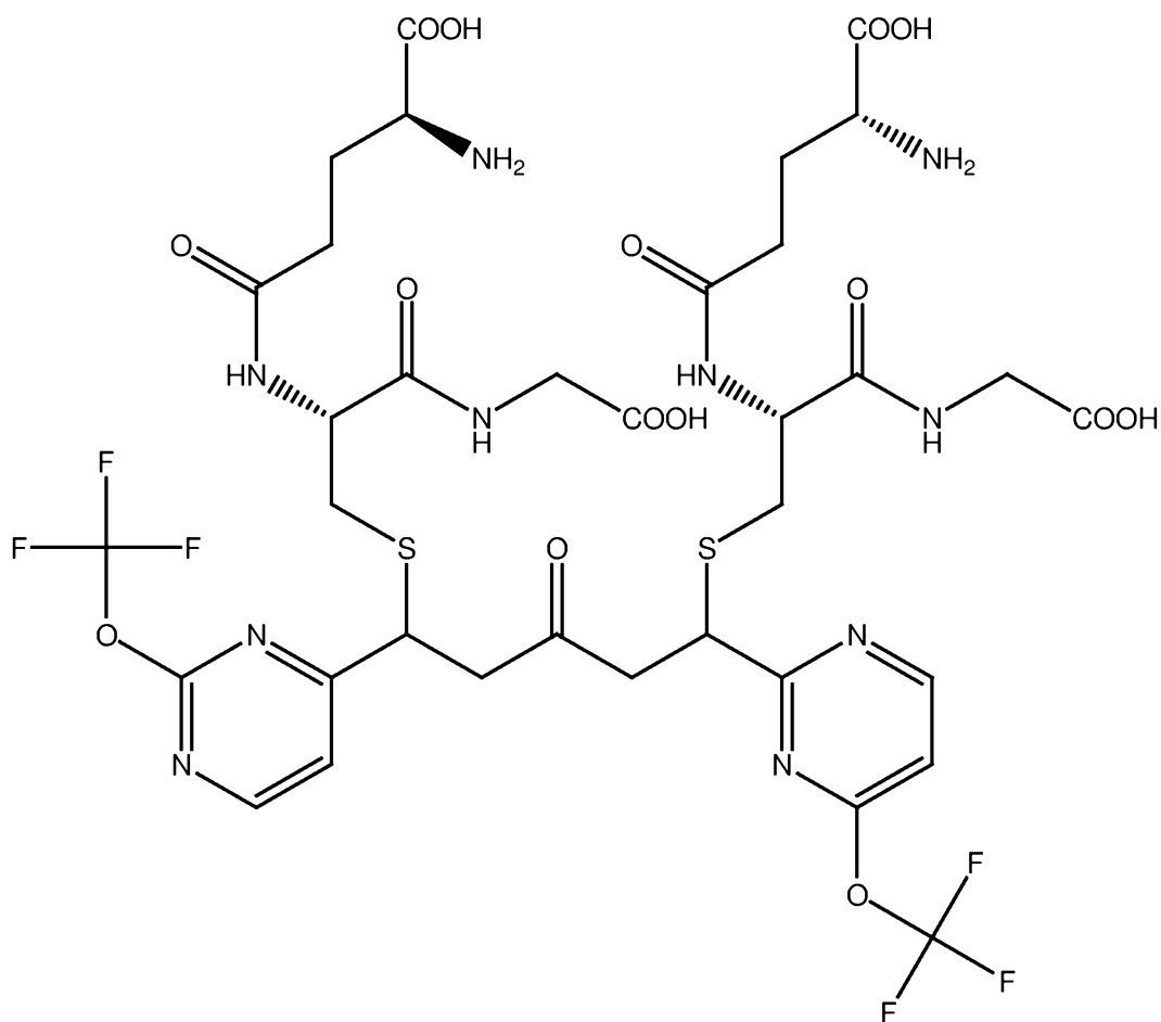
PB315 (glutathione adduct of PB312)
