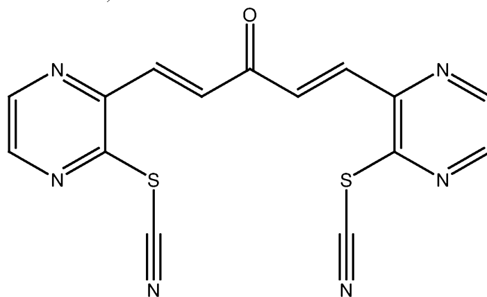
PB211 (glutathione adduct of PB208)
