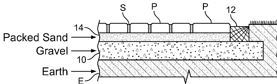
FIG. 8 (Prior Art)
