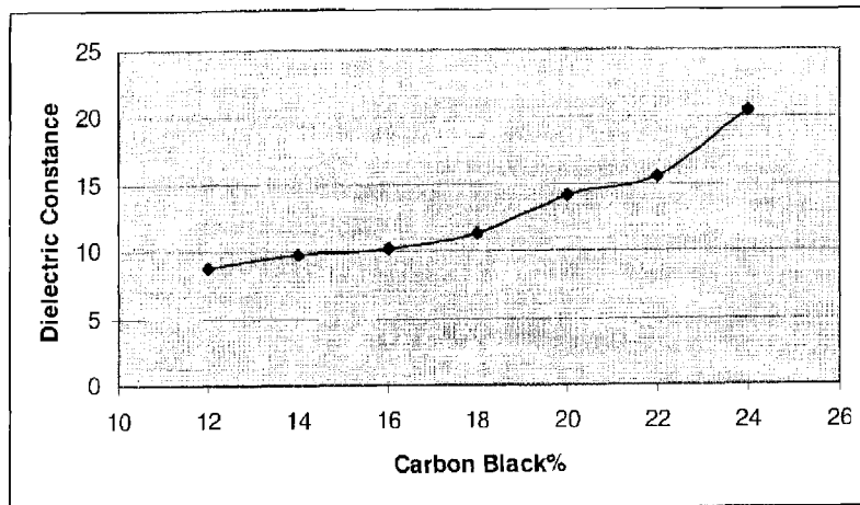
Dielectric Constance vs. Carbon Black Percent
