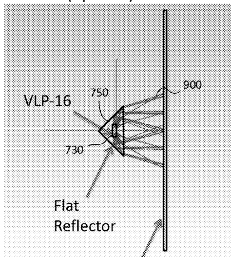
Analysis Plane FIG. 9B
