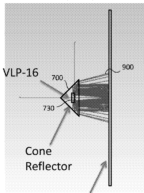
Analysis Plane FIG. 9A
