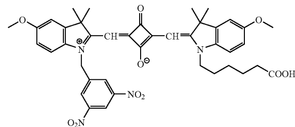
Compound (6)
