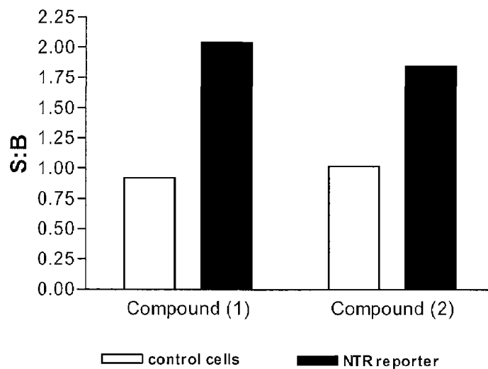
Figure 3b Signal:Background
