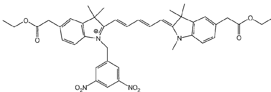
Compound (i)
