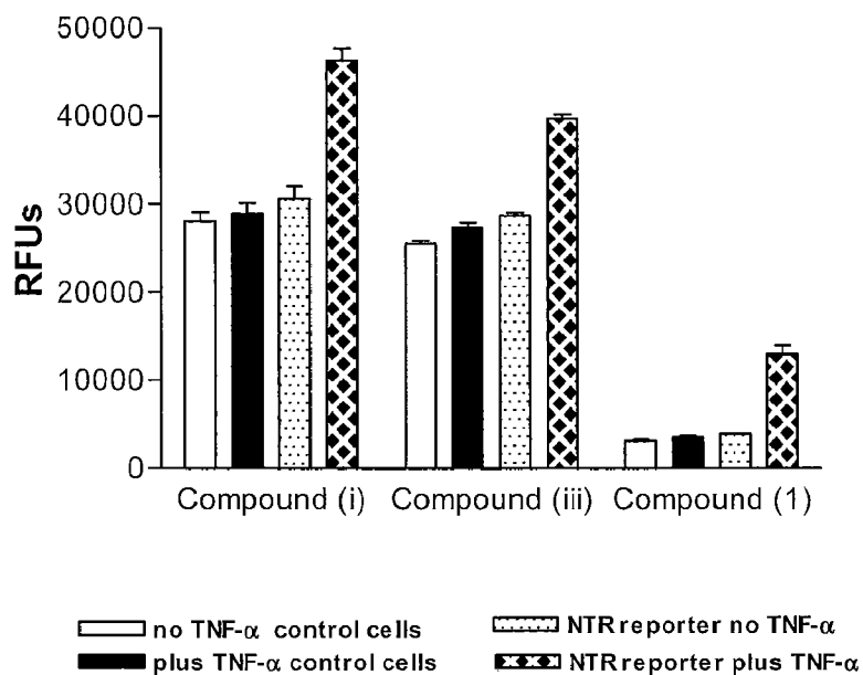
Figure 2b Signal:Background
