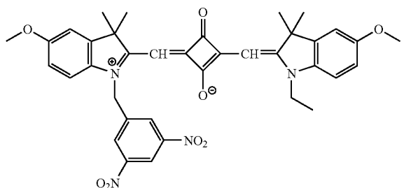
Compound (5)
