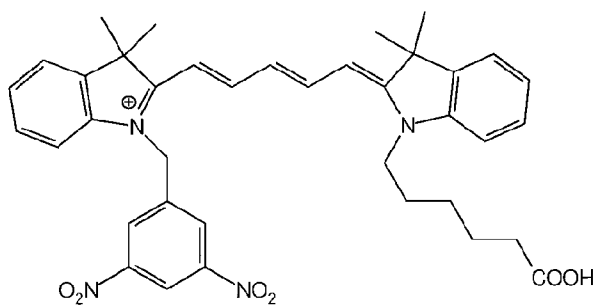
Compound (iii)
