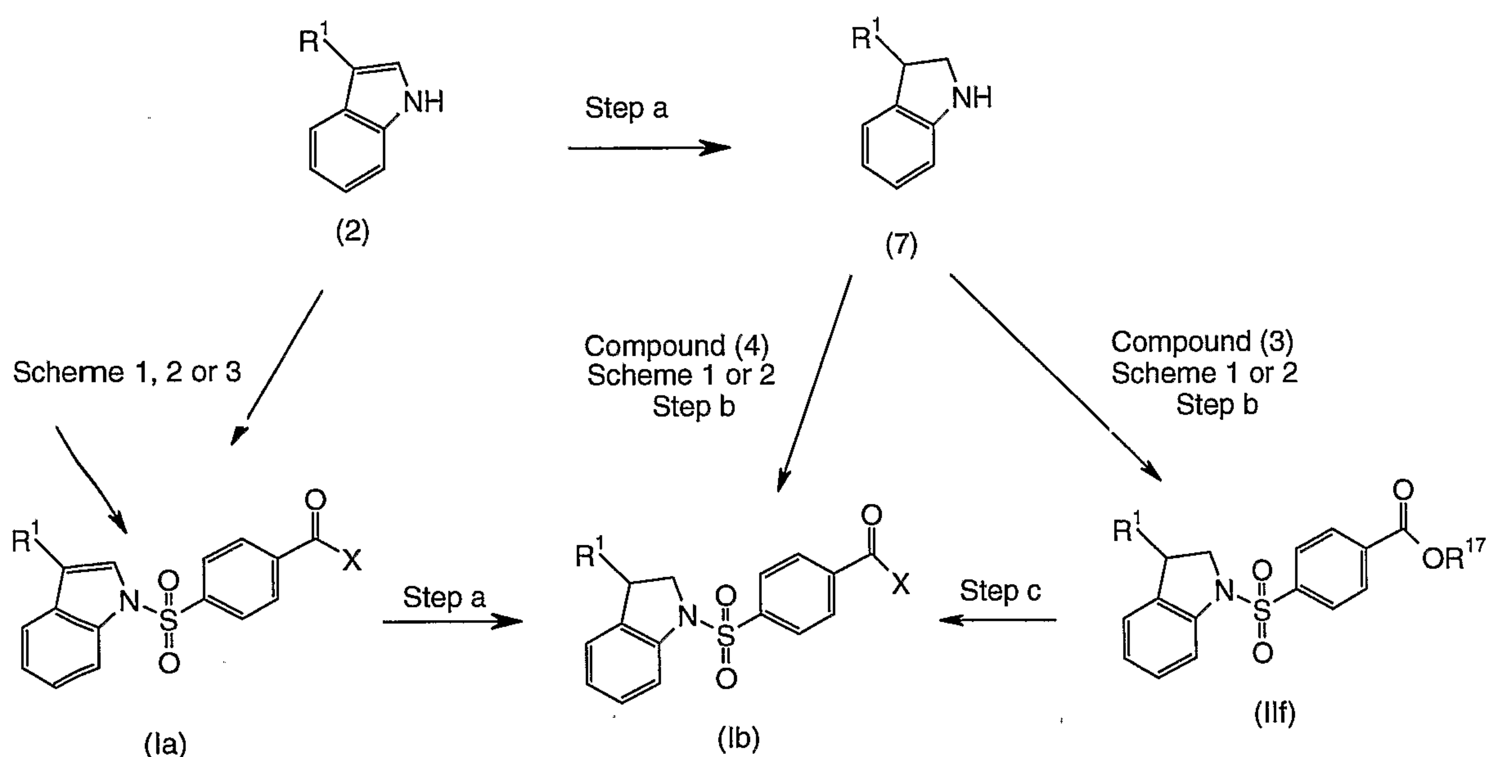
Scheme 4
