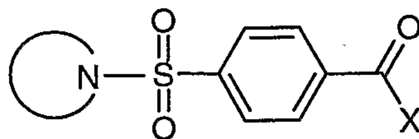
Formula I
