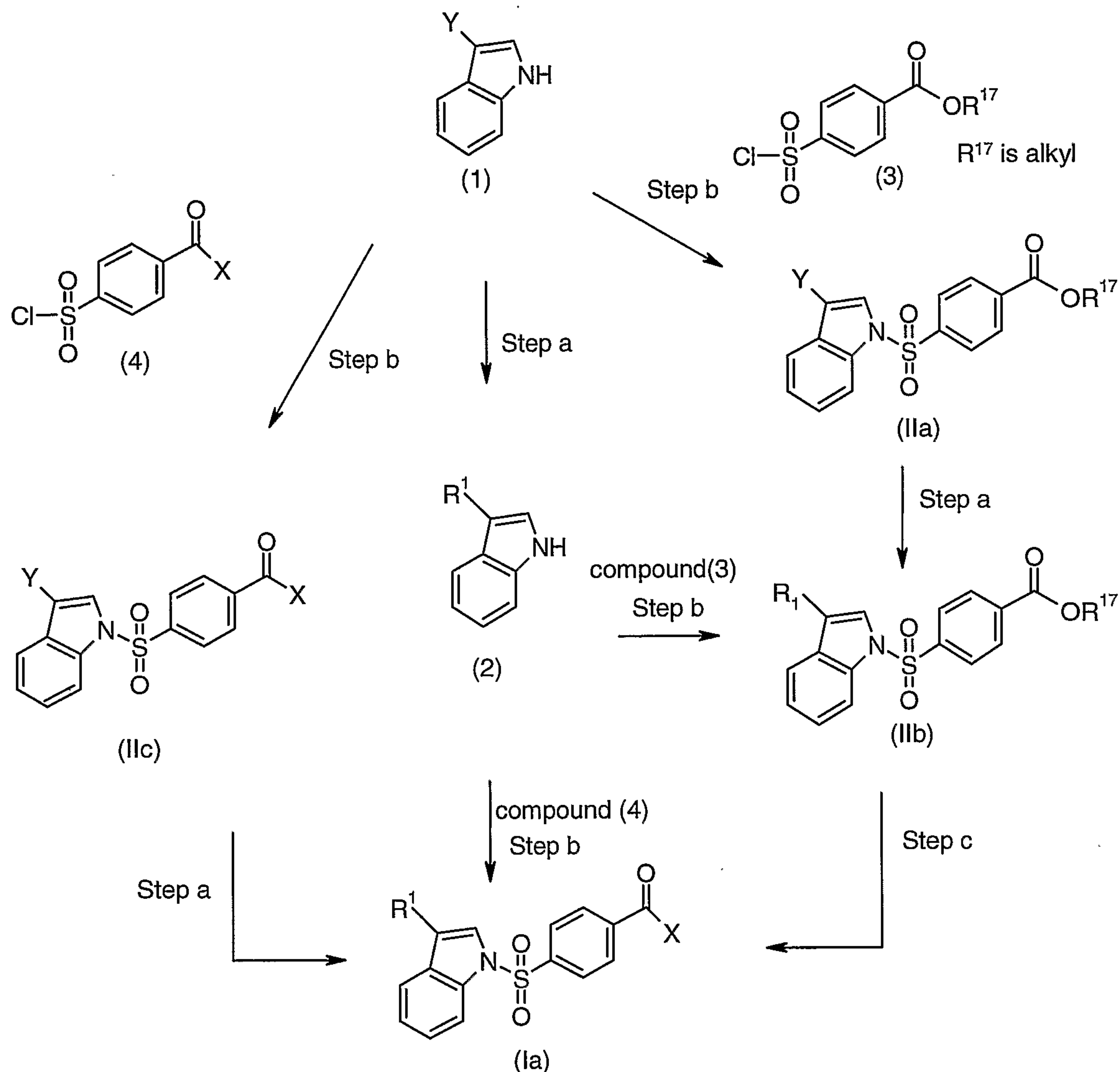
Scheme 1
