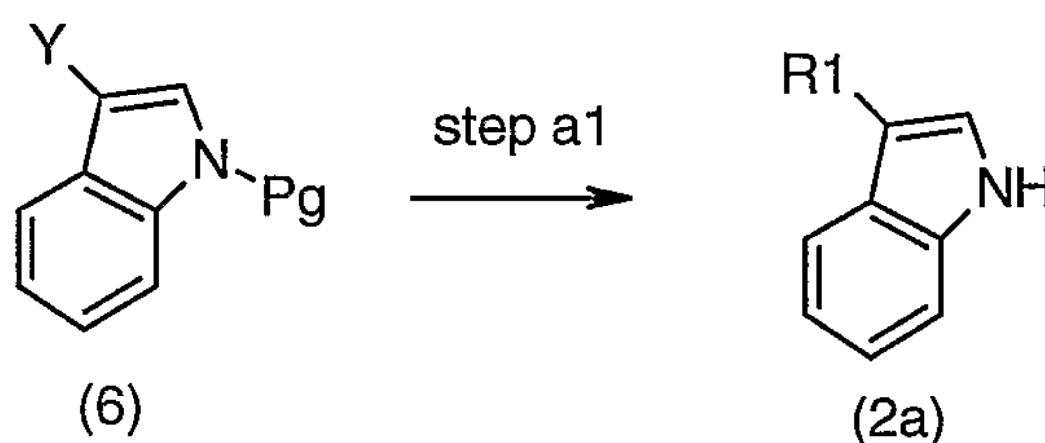
Scheme 3
