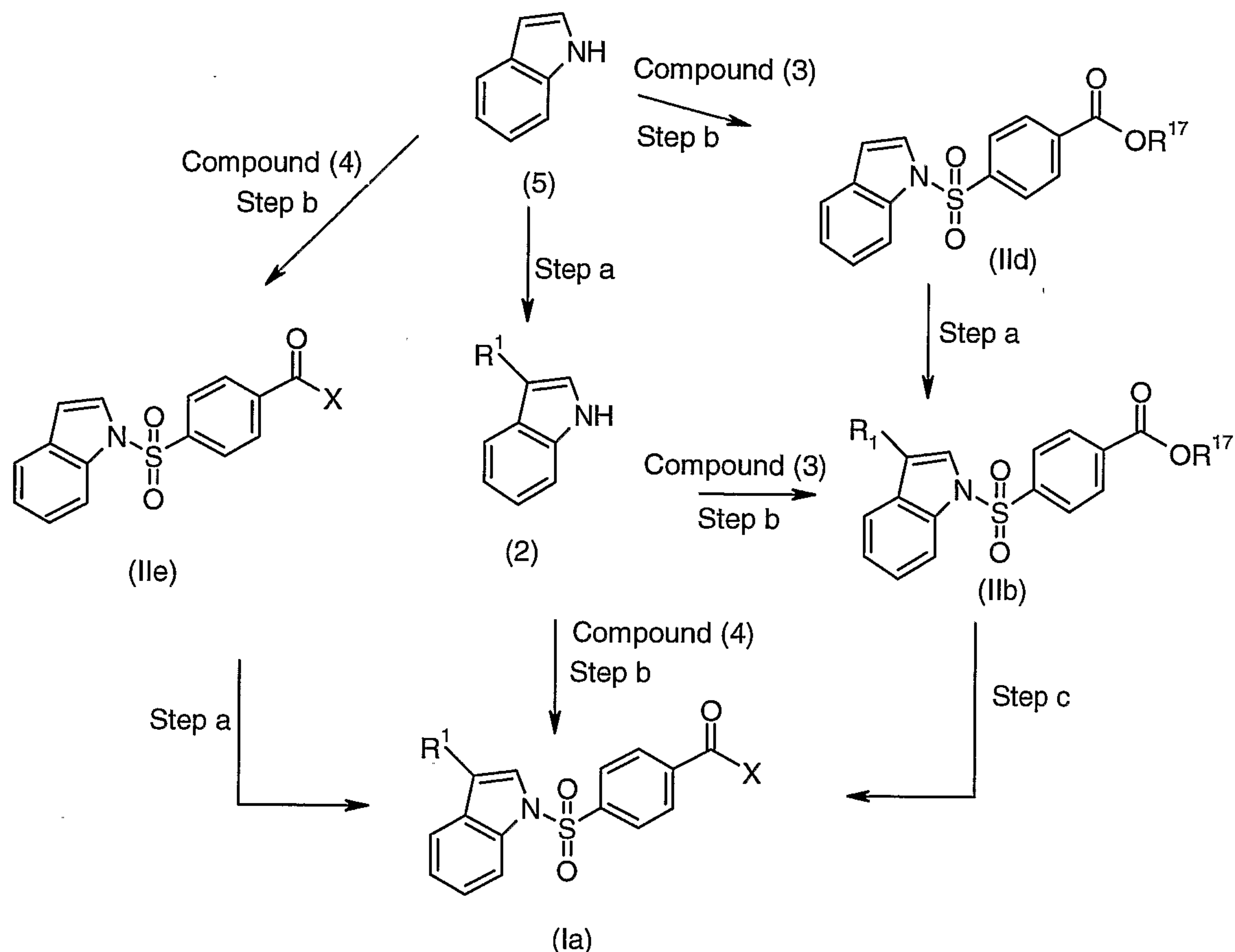
Scheme 2
