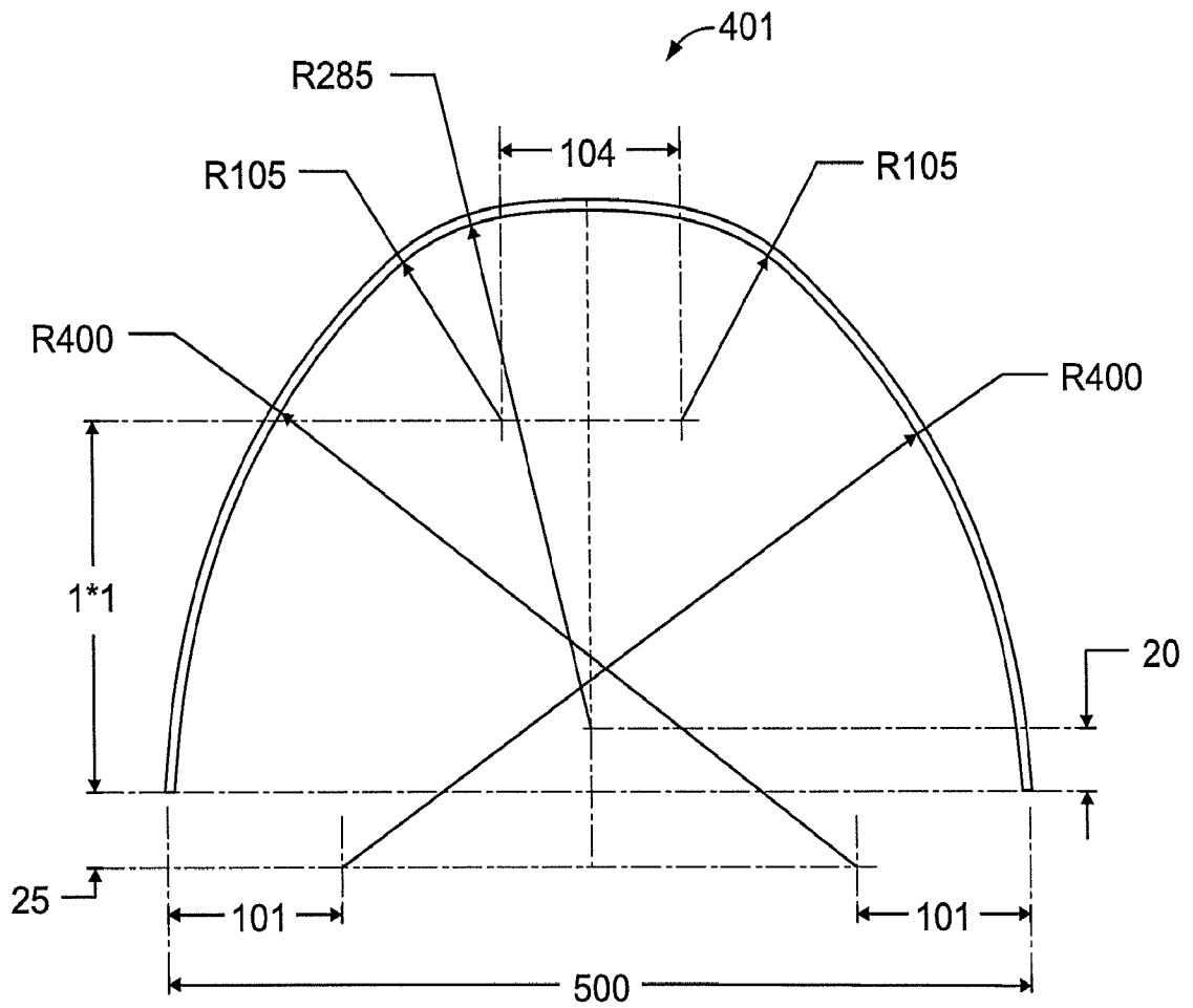
End view
