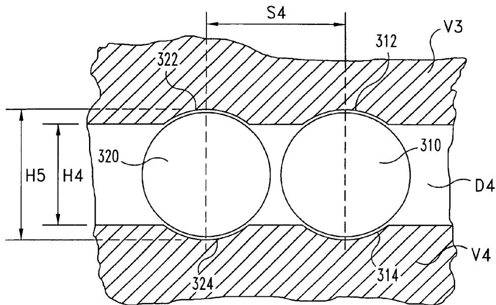
Fig. 11 (PRIOR ART)
