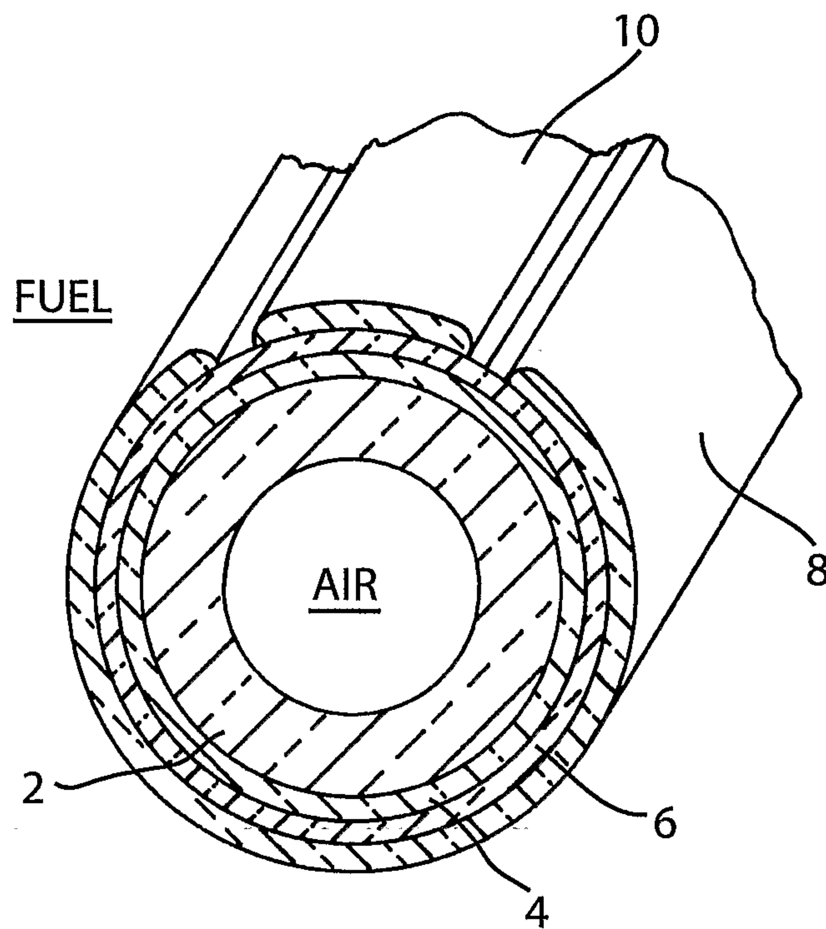
FIG. 1 PRIOR ART
