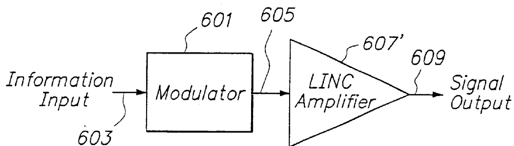
FIG. 6 (PRIOR ART)
