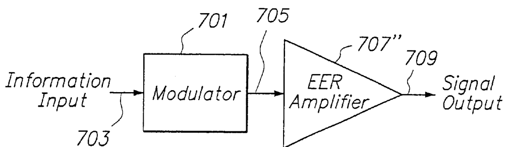
FIG. 7 (PRIOR ART)
