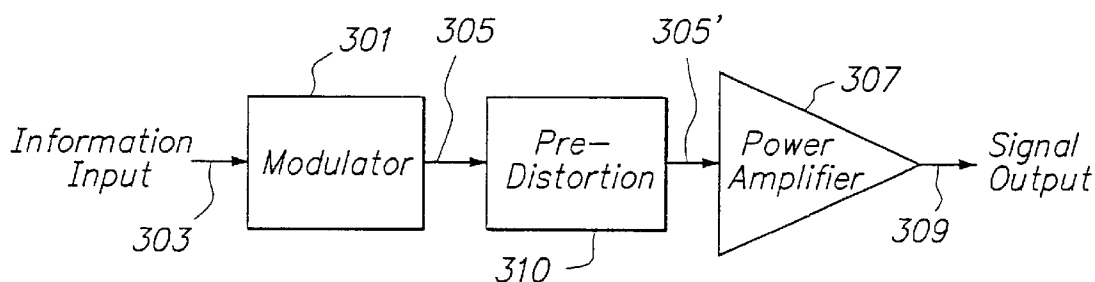
FIG. 3 (PRIOR ART)
