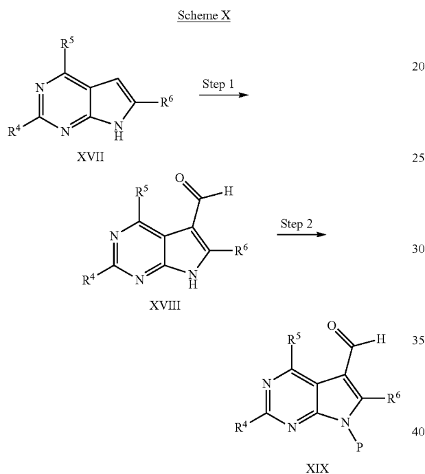
Step 1—Preparation of Compounds of Formula XVIII
