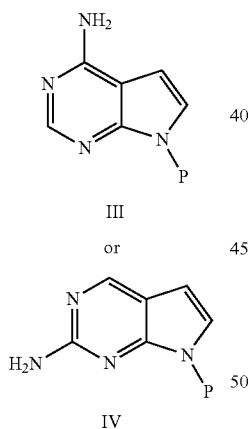
Step 1—Preparation of Compounds of Formula I or II
