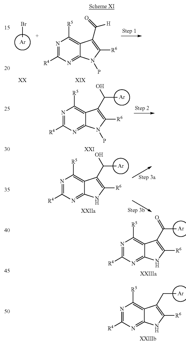
Step 1—Preparation of Compounds of Formula XXI
