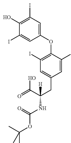
N-tert-butylloxycarbonyl-L-thyroxine
