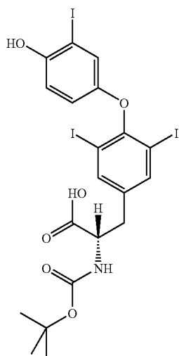
N-tert-butylloxycarbonyl-3',3',5-triiodo-L-thyronine
