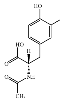
N-acetyl-3-iodo-L-thyroxine
