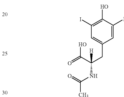
N-acetyl-3,5-diiodo-L-tyrosine
