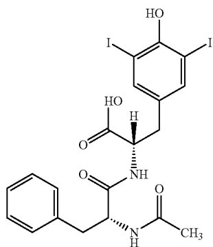
N-acetylphenylalanyl-3,5-diiodo-L-tyrosine
