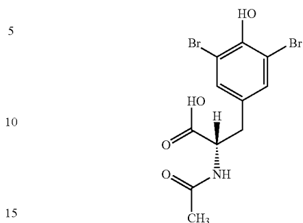
N-acetyl-3,5-dibromo-L-tyrosine
