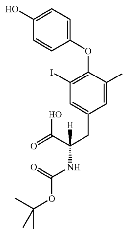
N-tert-butylloxycarbonyl-3,5-diiodo-L-thyronine
