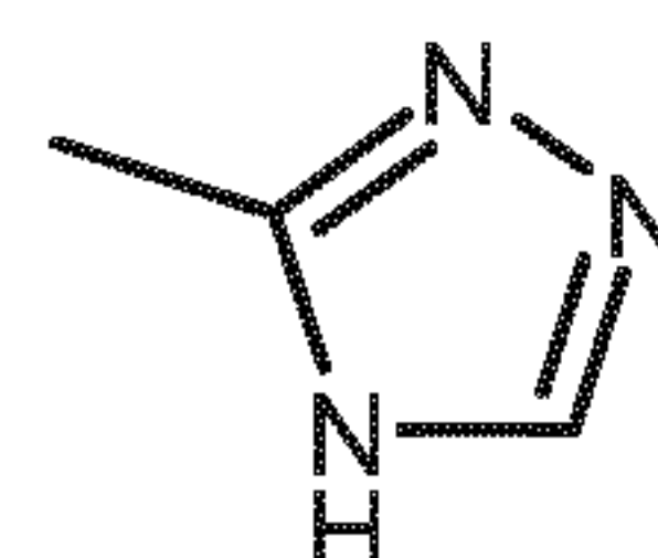
4H-tautomer.
