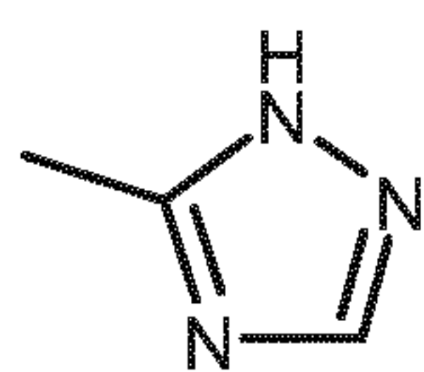
1H-tautomer
