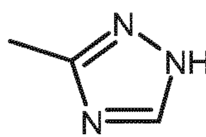
2H-tautomer
