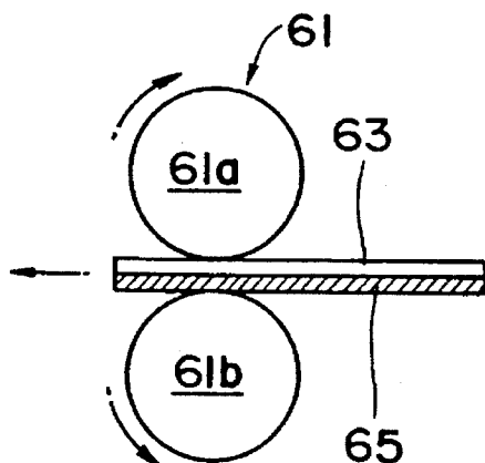
FIG. 8 (PRIOR ART)
