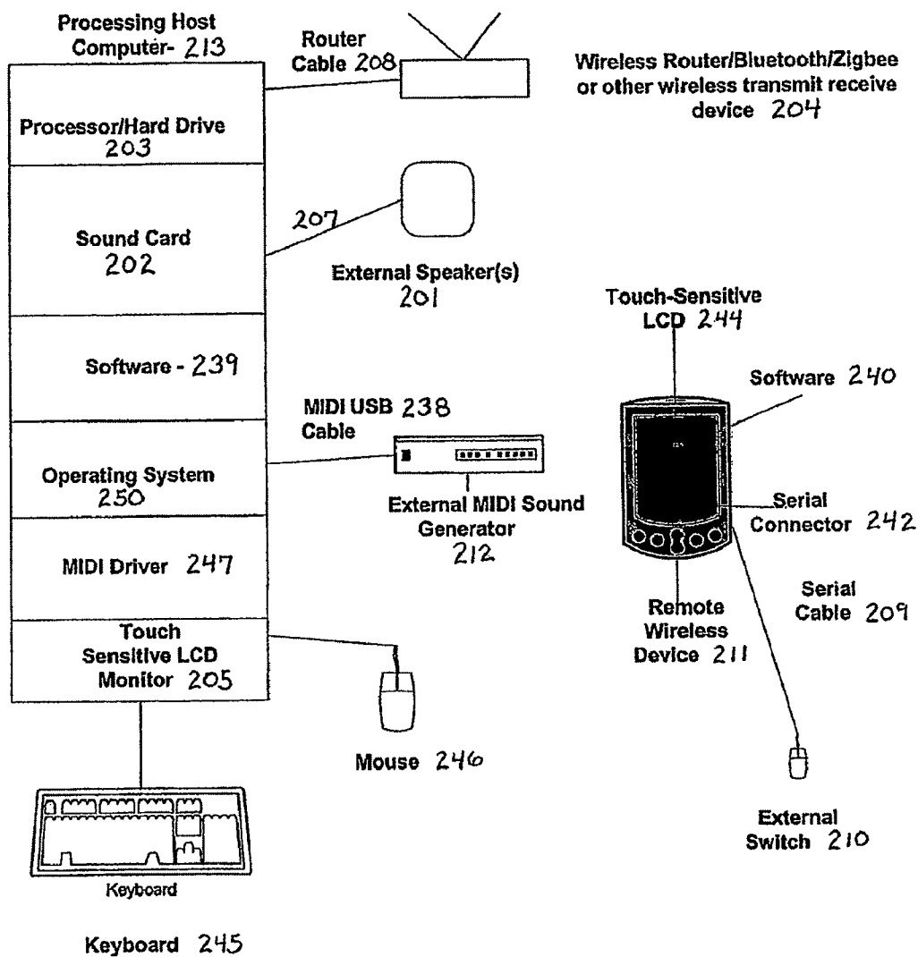
Fig. 1C - Alternative Schematic
