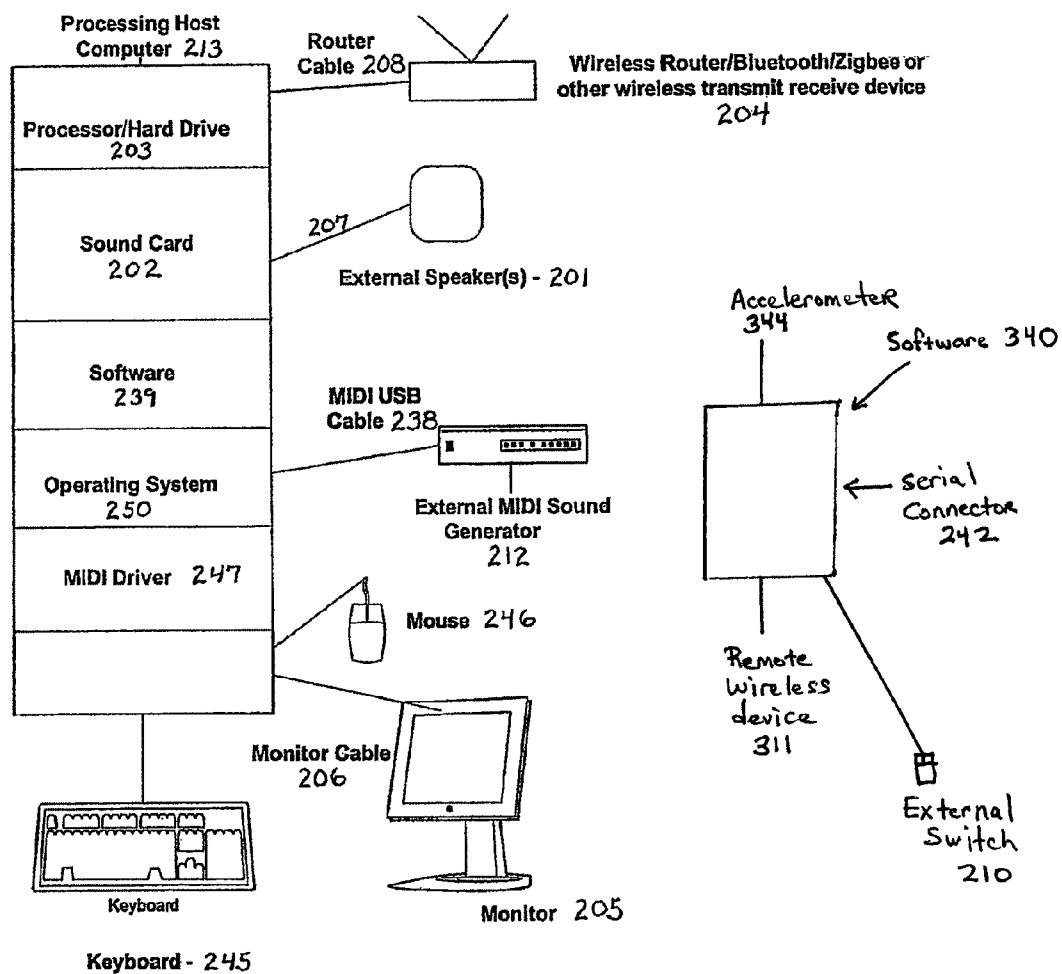
Fig. 1D - Schematic
