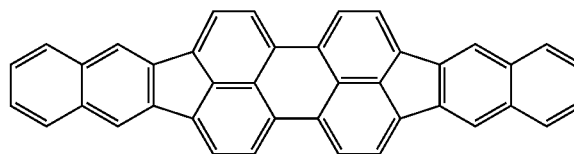
Formula 501-16
