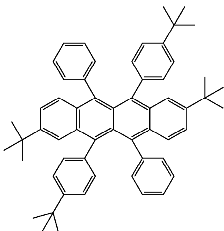
Compound FD(9)
