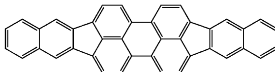
Formula 501-16
