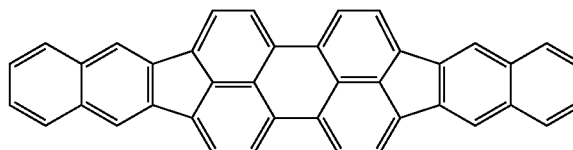
Formula 501-17
