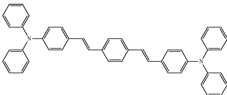
Compound FD(8)
