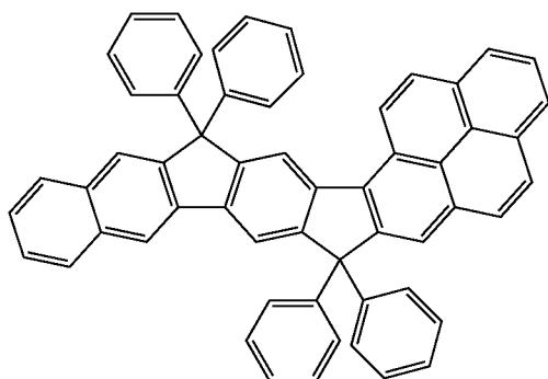
Formula 501-12
