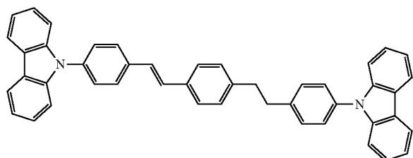
Compound FD(7)
