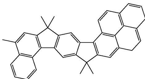
Compound FD(9)
