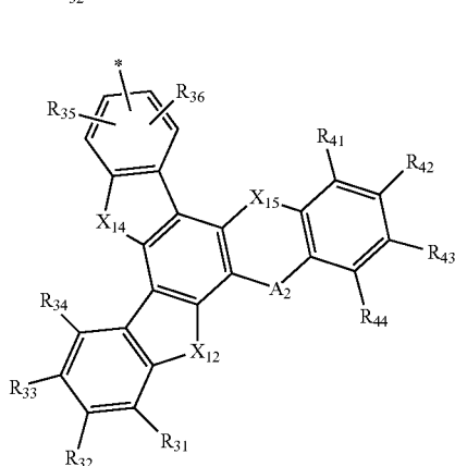
Formula 14-8
