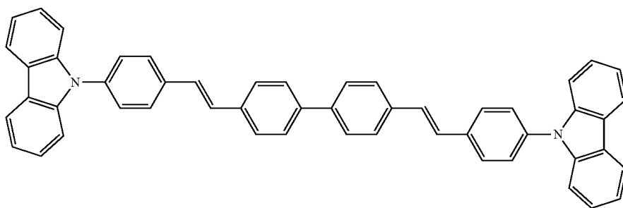
Compound FD(3)
