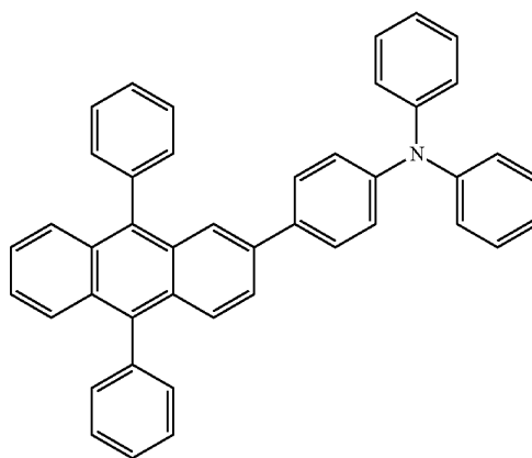
Compound FD(4)
