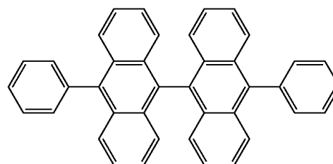
Compound FD(13)
