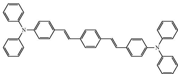
Compound FD(8)
