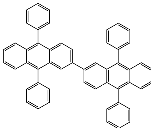
Compound FD(4)
