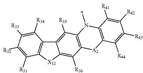
Formula 13-5
