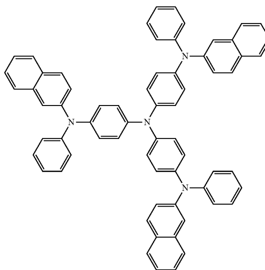
2-TNATA
