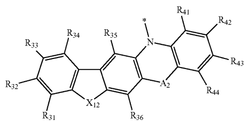
Formula 13-5
