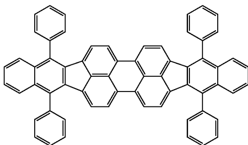
Compound FD(10)
