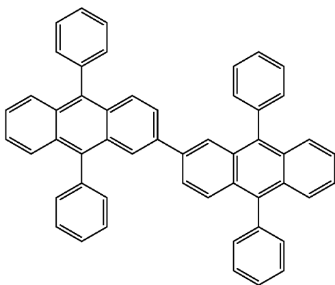
Compound FD(5)
