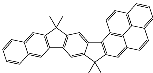
Formula 501-6
