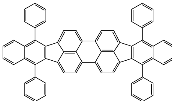
Compound FD(11)
