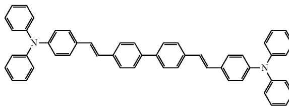
Compound FD(2)
