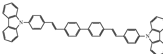
Compound FD(3)
