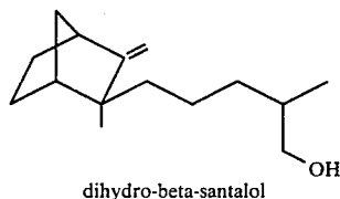
dihydro-beta-santalol
