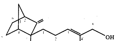
endo-3-methyl-exo-3-(trans-5'-hydroxy-4'-methylpent-3'-enyl)-2-methylenebicyclo[2.2.1]heptane
