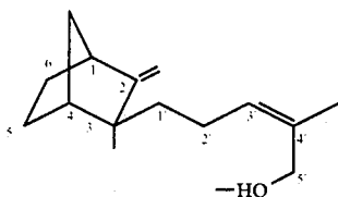
endo-3-methyl-exo-3-(cis-5'-hydroxy-4'-methylpent-3'-enyl)-2-methylenebicyclo[2.2.1]heptane
