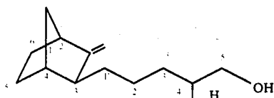
2-methylene-3-exo-(4'-methyl-5'-hydroxypentyl)-bicyclo[2.2.1]heptane; 3-normethyldihydro-beta-santalol
