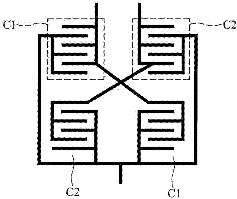
FIG. 2 (PRIOR ART)
