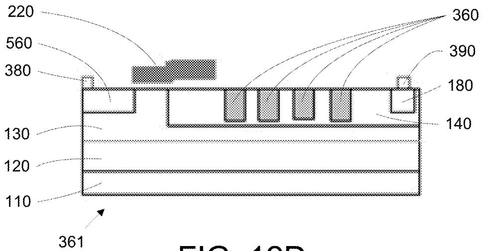
FIG. 12D
