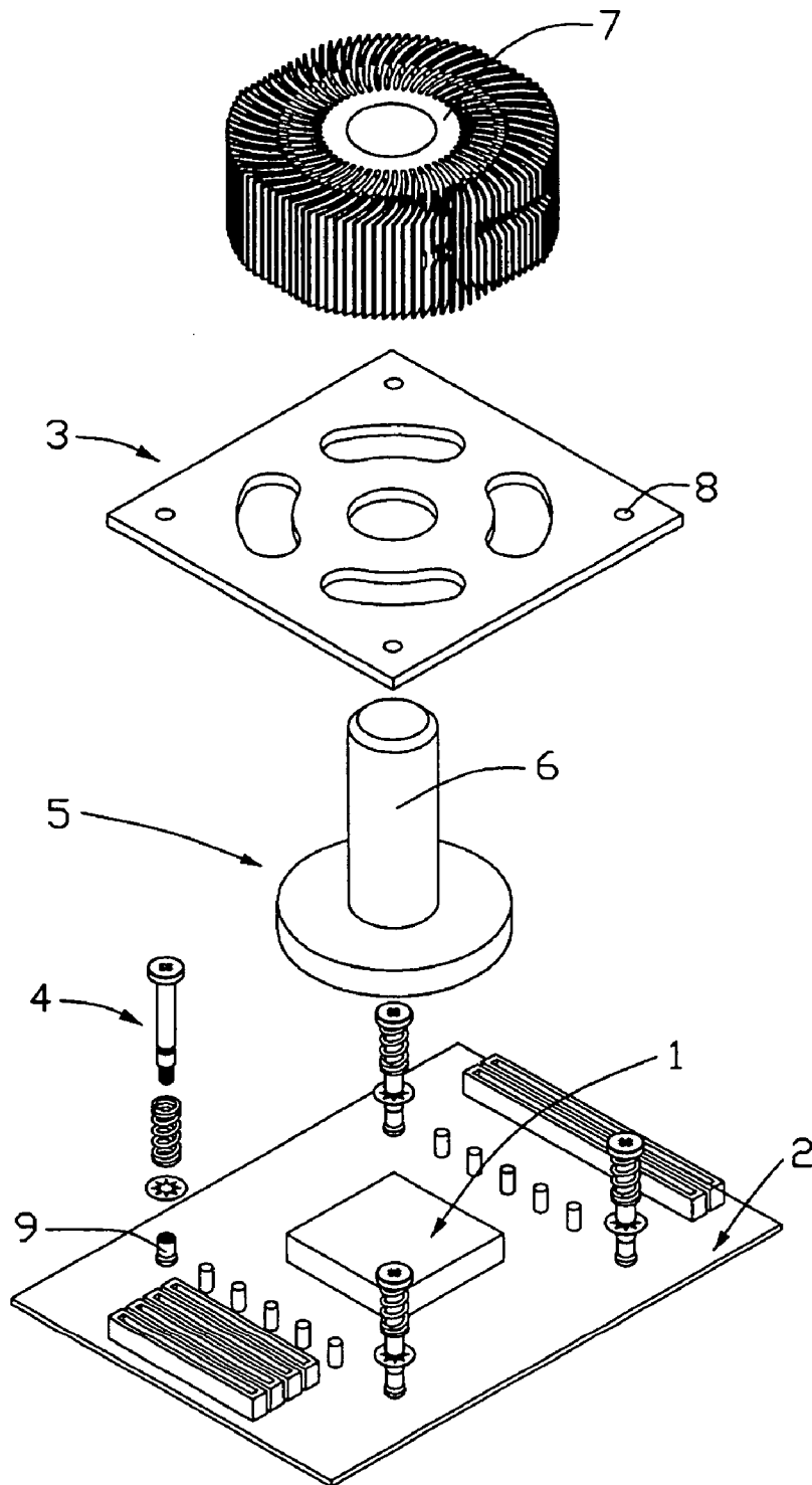
FIG. 5 (RELATED ART)
