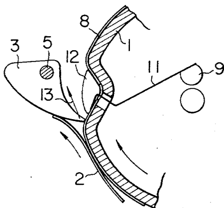
FIG. 3 PRIOR ART
