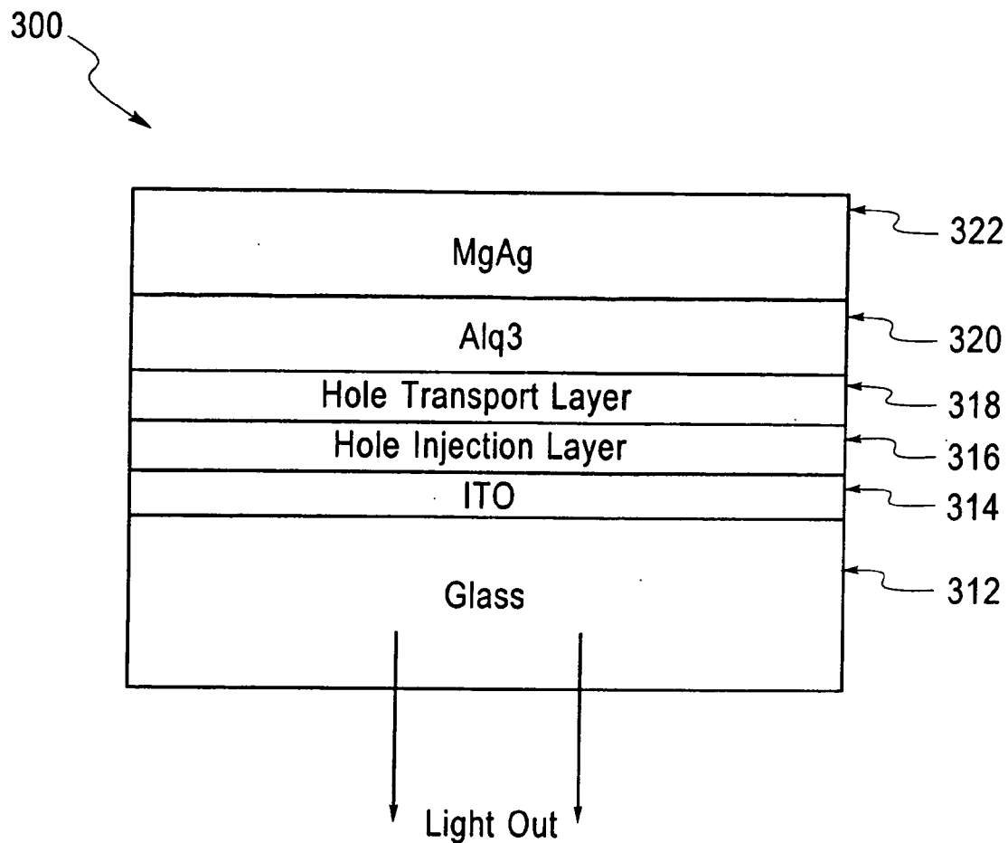
Fig. 18 Prior Art
