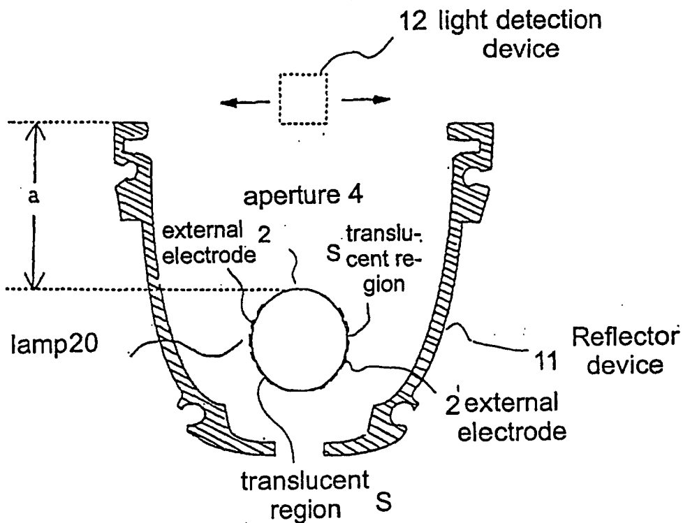
FIG. 9 Schematic of an arrangement of a first embodiment of an irradiation unit as claimed in the invention
