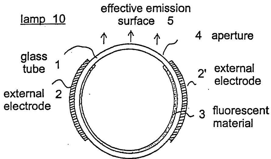
FIG. 8 Schematic of a fluorescent lamp of the external electrode type in which there is reflector material arranged
