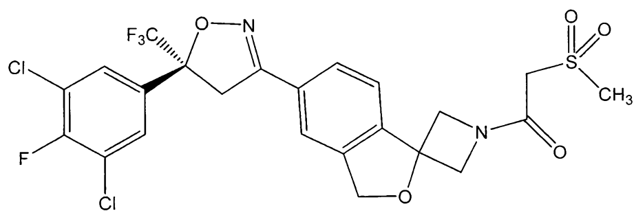
sarolaner
