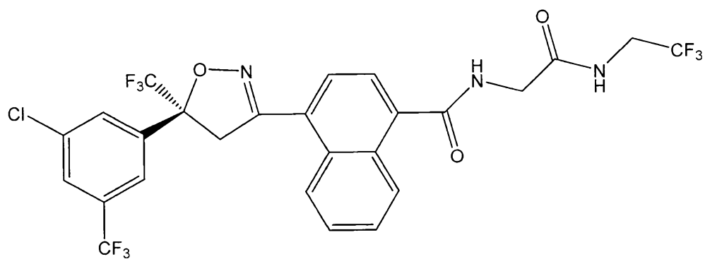
(S)-afoxolaner
