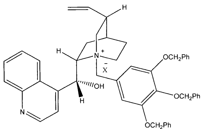
(IIIa-13-3)
