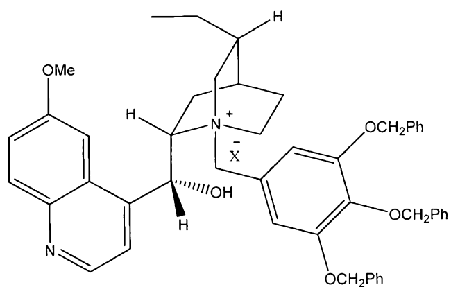
(IIIa-13-2)
