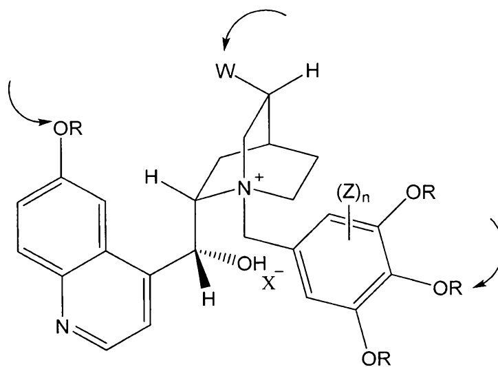
(IIIa-13)
