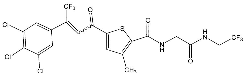
(IID-1)
