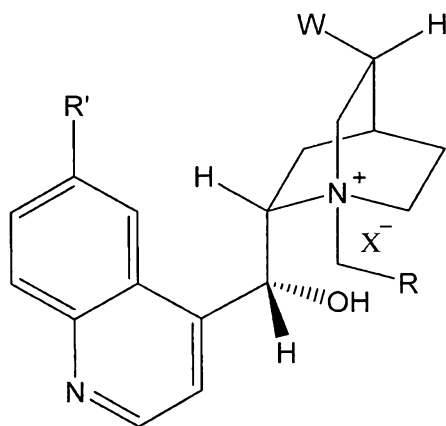
(IIIa)
