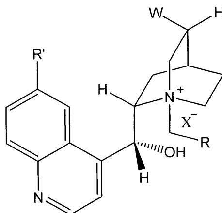
(IIIa)
