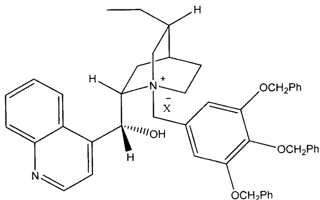
(IIIa-13-4)
