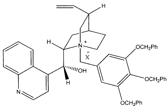
(IIIa-13-3)
