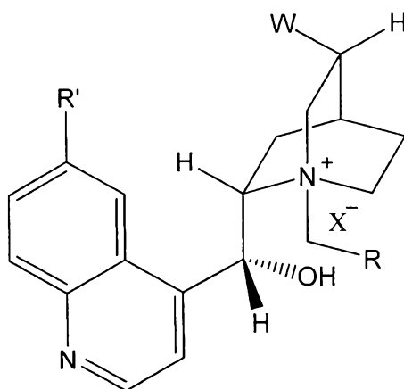
(IIIa)
