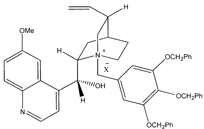
(IIIa-13-1)
