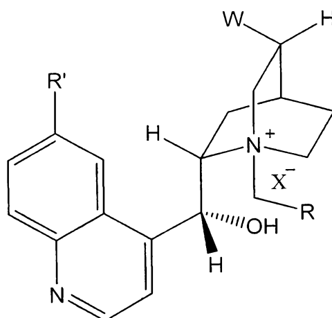
(IIIa)
