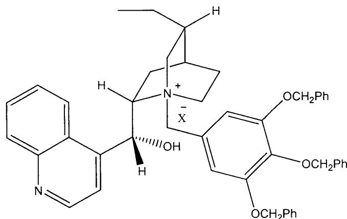
(IIIa-13-4)
