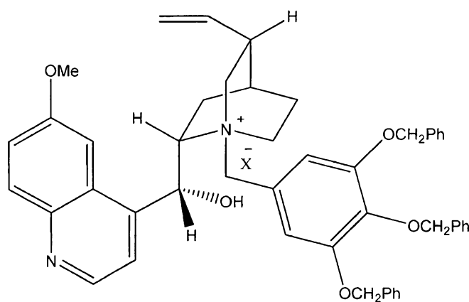
(IIIa-13-1)
