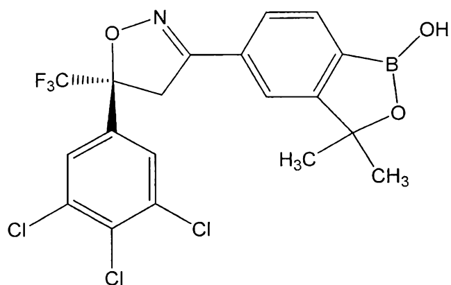
(S)-IE-1
