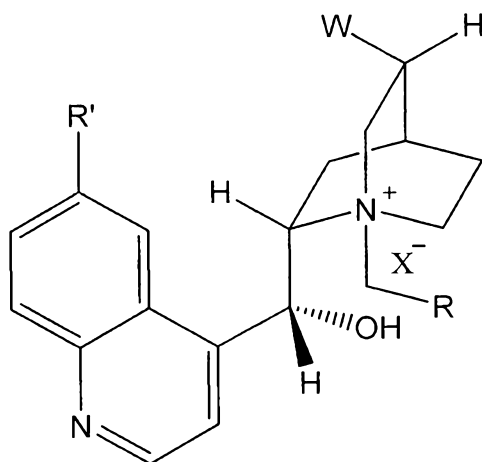
(IIIa)
