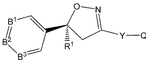
(S)-I
