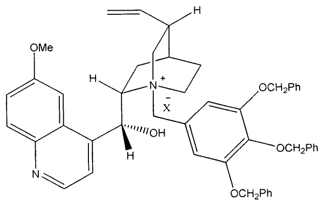
(IIIa-13-1)
