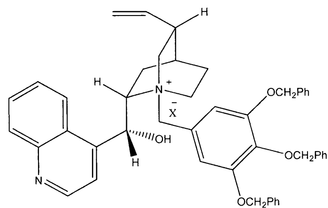
(IIIa-13-3)
