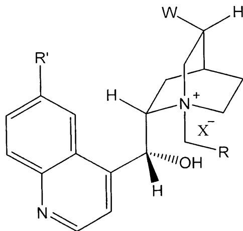
(IIIa)
