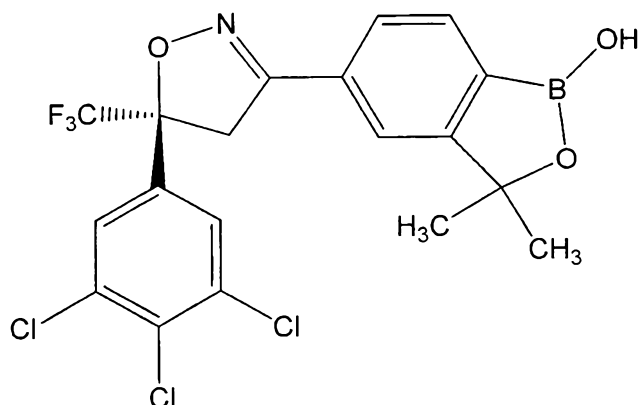
(S)-ID-1
