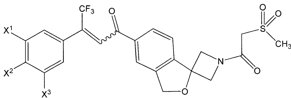
(IIC)
