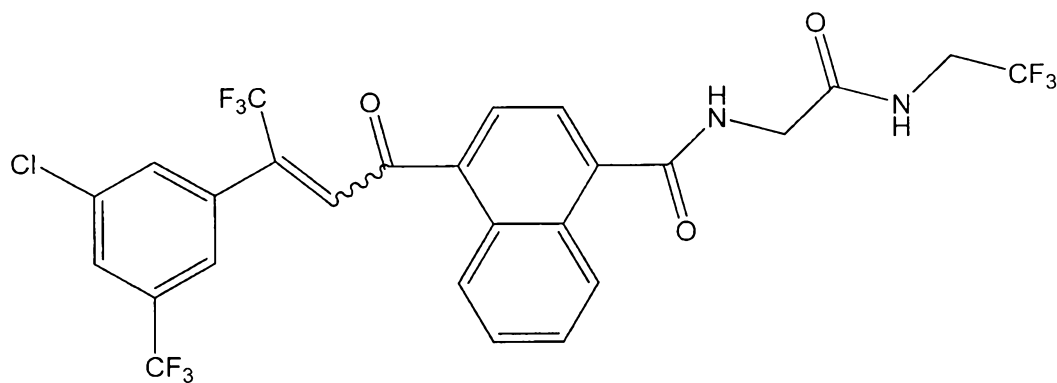
(IIA-1)
