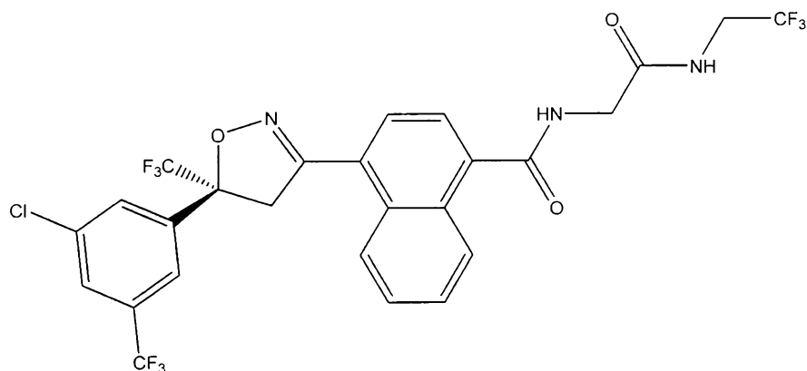
(S)-afoxolaner
