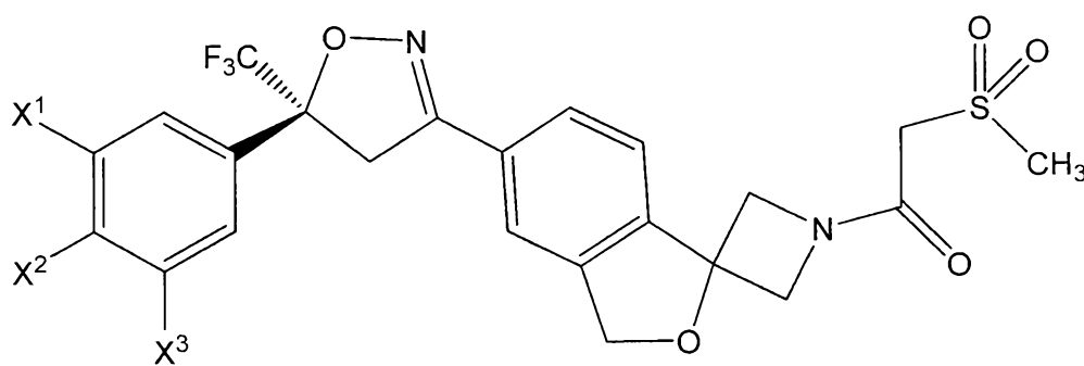
( S )-IC
