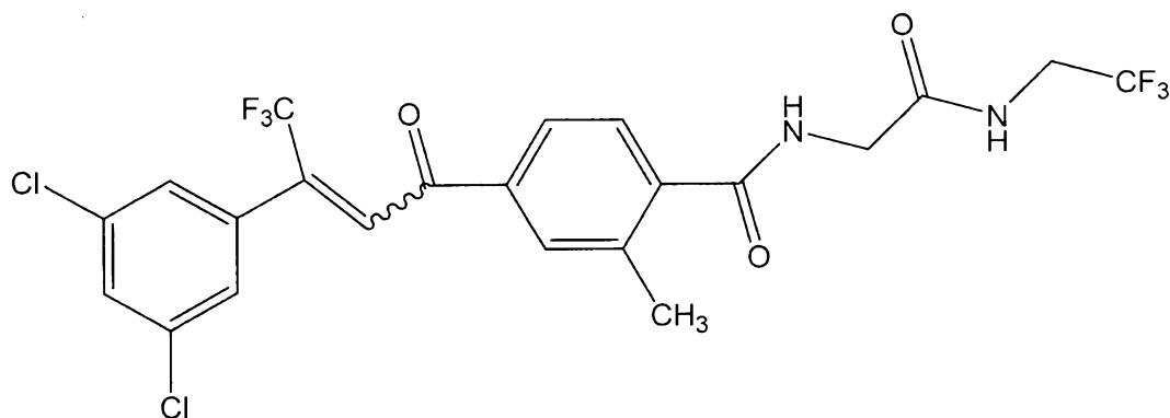
(IIB-1)
