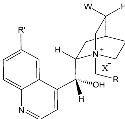
(IIIa)
