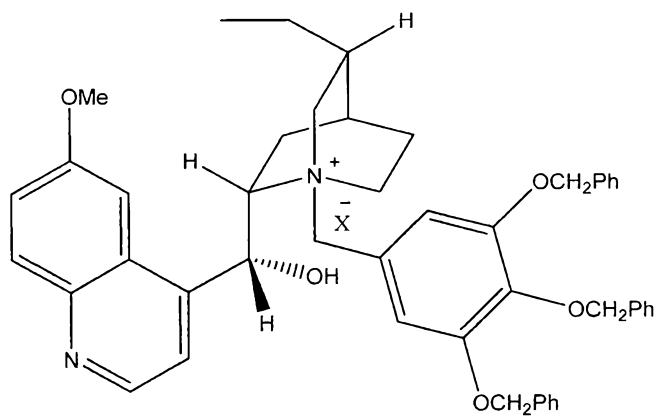
(IIIa-13-2)
