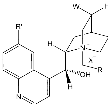
(IIIa)
