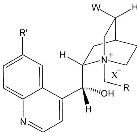
(IIIa)
