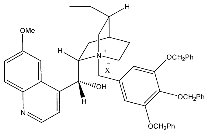
(IIIa-13-2)
