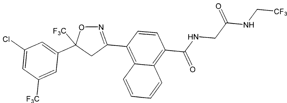
Afoxolaner
