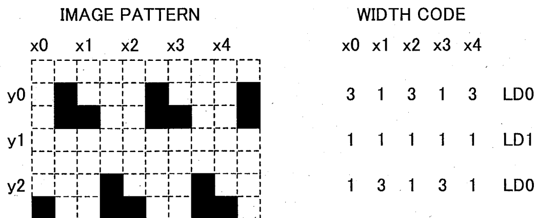
FIG.13D
