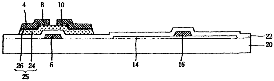
FIG. 2D RELATED ART
