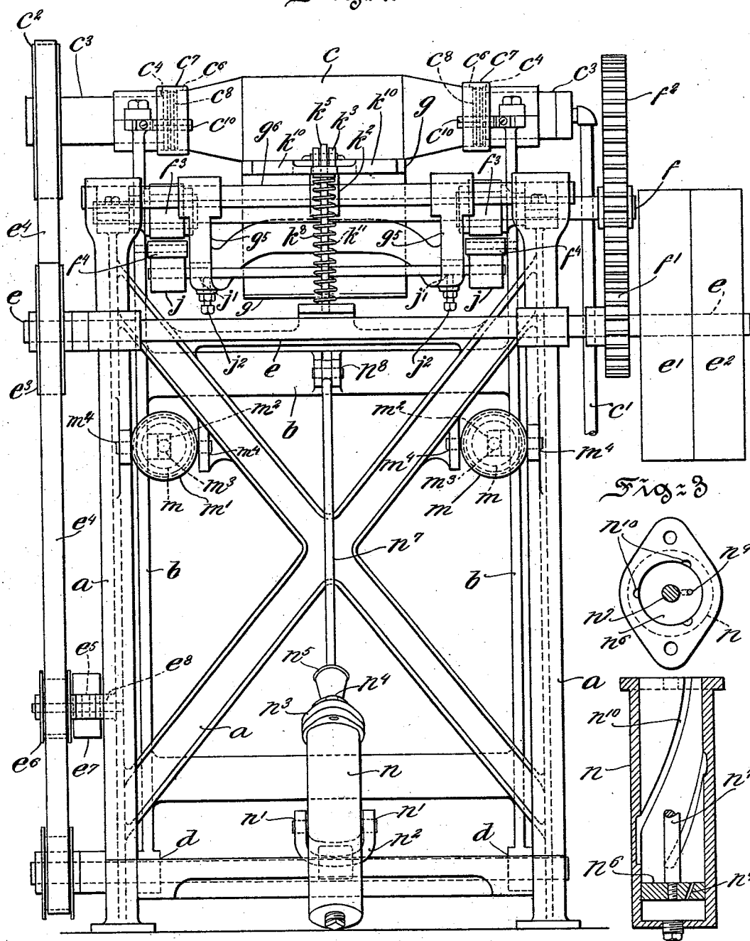
\sqrt{2} \approx 1.414
