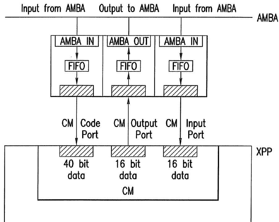
Receiver and transmitter for external units
