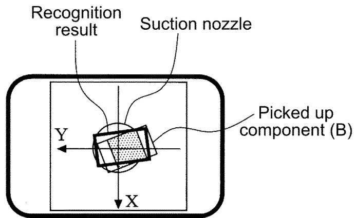
Image of suction state of component (B)
