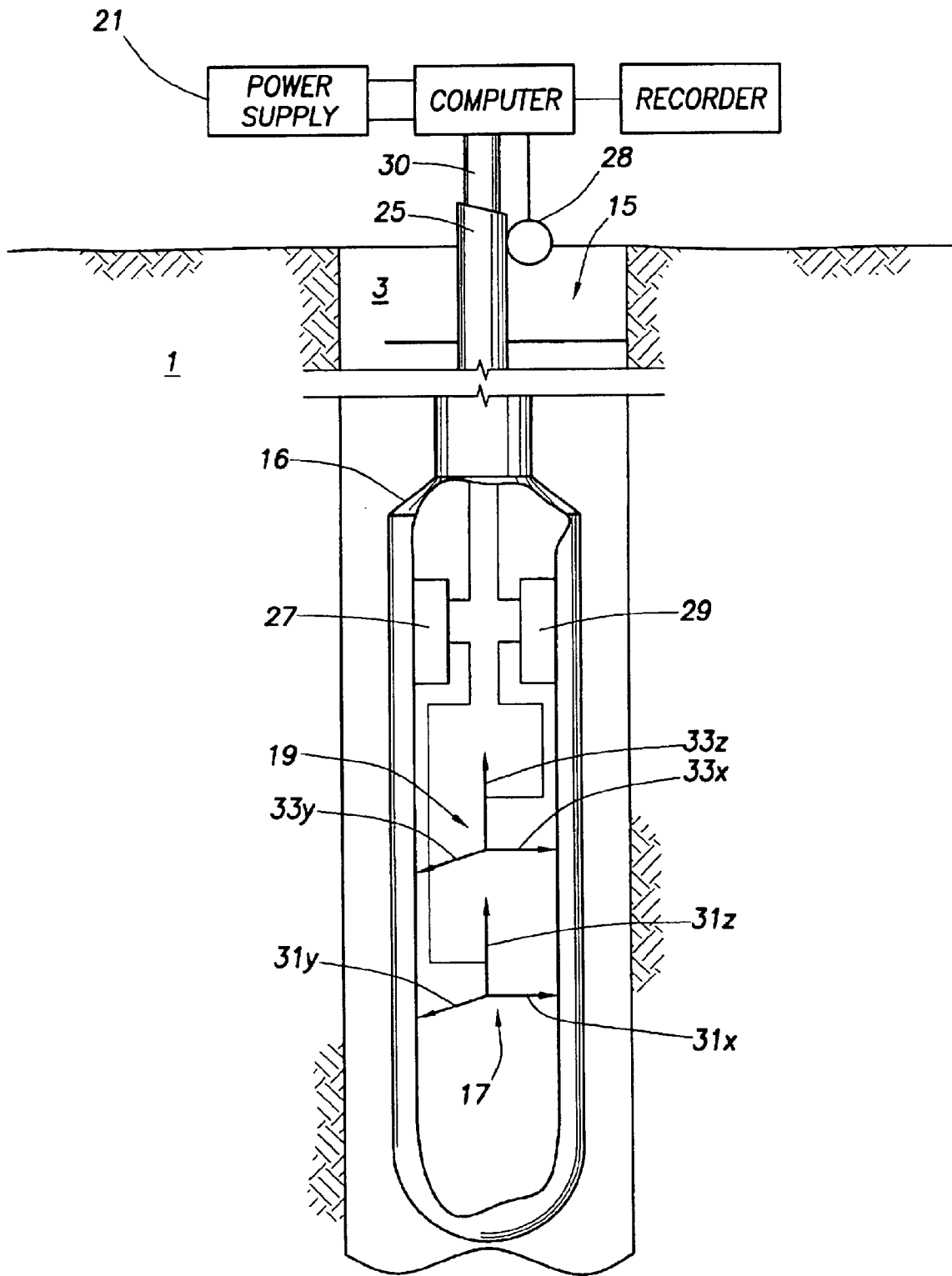
FIG.2 (PRIOR ART)
